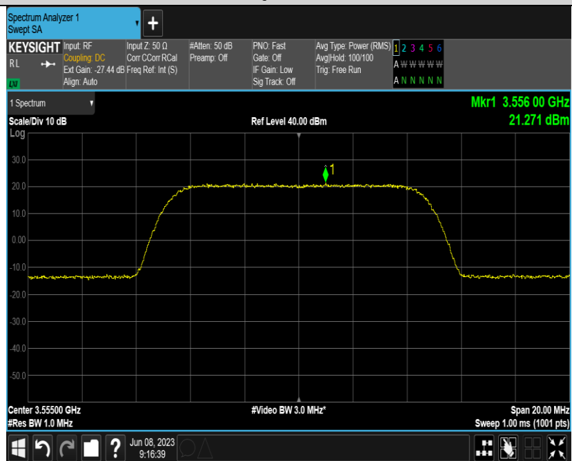
Band48-10MHz-256QAM-55990-E-TM3.1A-1000
