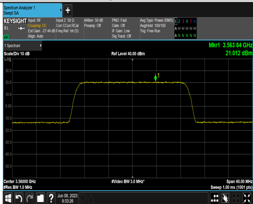
Band48-20MHz-QPSK-55990-E-TM1.1-1000
