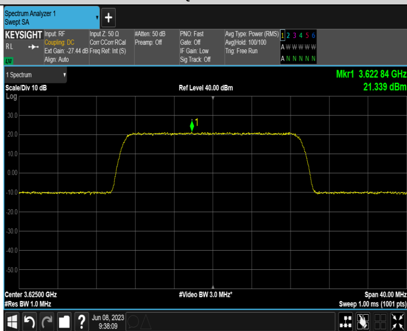
Band48-20MHz-256QAM-56640-E-TM3.1A-1000
