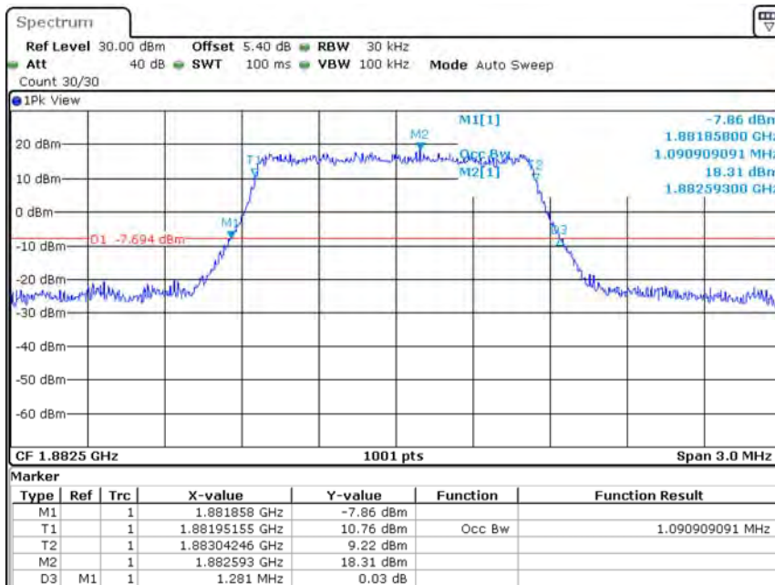
Band25-1.4MHz-QPSK-26365-6RB#0-1.091
