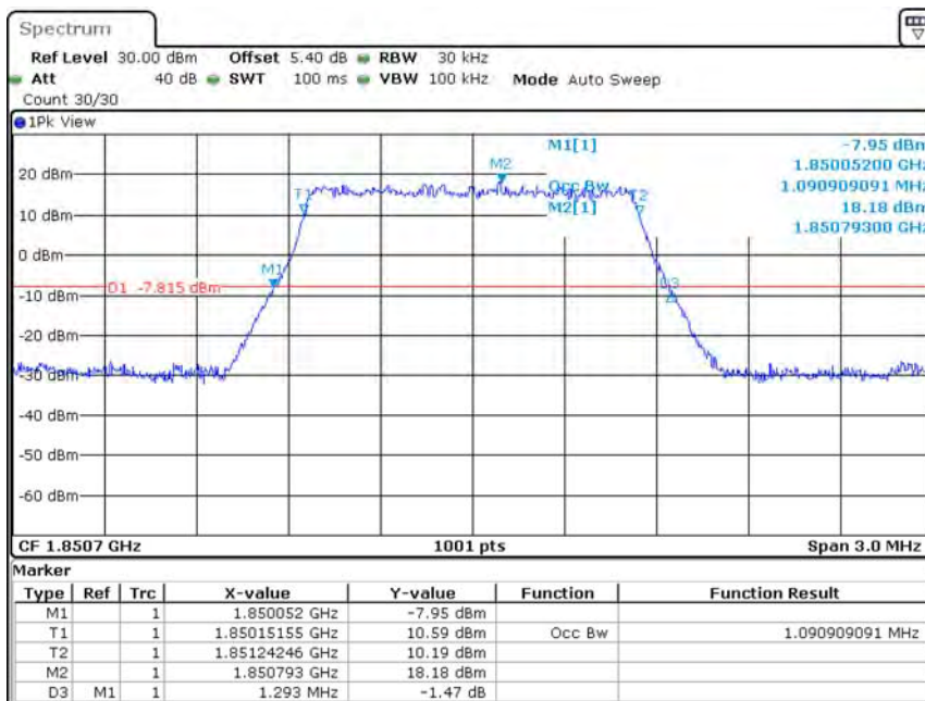
Band25-1.4MHz-QPSK-26047-6RB#0-1.091
