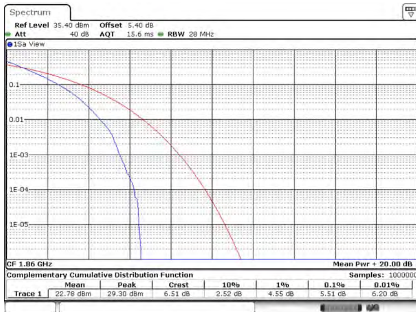
Band25-20MHz-QPSK-26140-100RB#0
