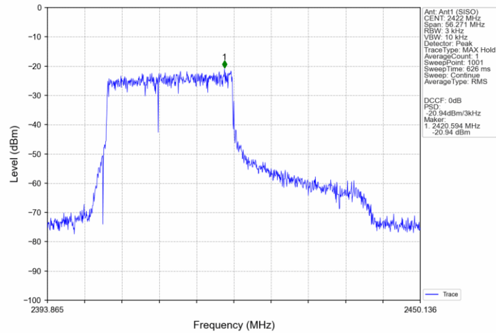
802.11ax(HEW40)_LCH_2422MHz_RU484_65_Ant1 (SISO)_NTNV
