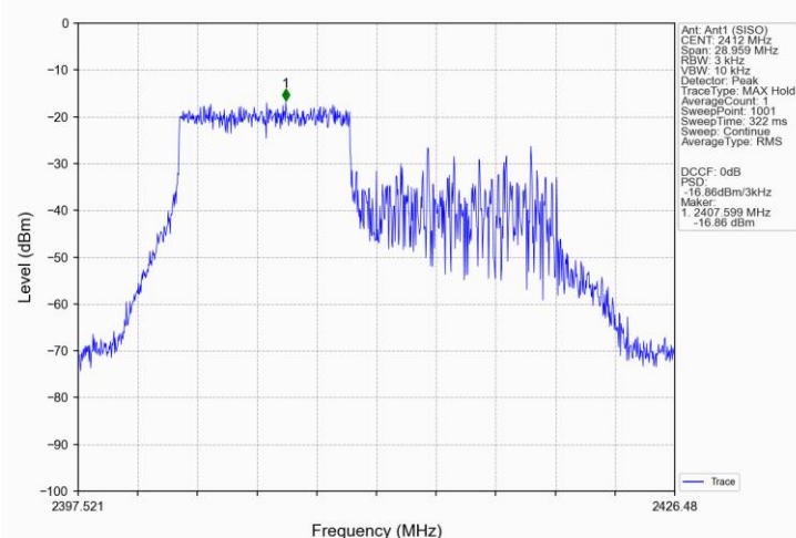
802.11ax(HEW20)_LCH_2412MHz_RU242_61_Ant1 (SISO)_NTNV
