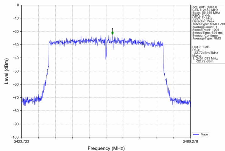
802.11ax(HEW40)_HCH_2452MHz_RU484_65_Ant1 (SISO)_NTNV
