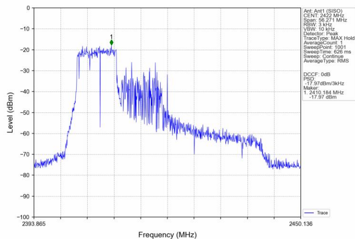
802.11ax(HEW40)_LCH_2422MHz_RU242_61_Ant1 (SISO)_NTNV
