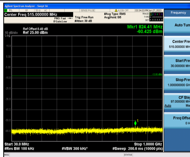
Band4-1.4MHz-16QAM-20393-1-0-Low-30-1000--60.43-PASS
