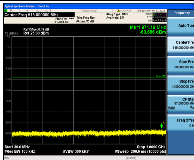
Band4-1.4MHz-QPSK-20393-1-0-Low-30-1000--60.69-PASS
