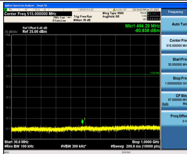
Band4-1.4MHz-QPSK-20175-1-0-Low-30-1000--60.84-PASS
