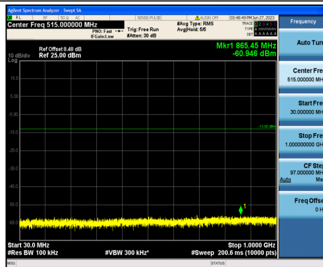
Band4-3MHz-QPSK-20385-1-0-Low-30-1000--60.95-PASS
