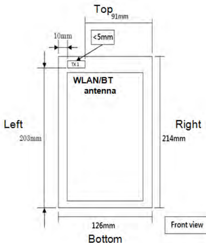
Fig.8 Antenna position (Front view)
