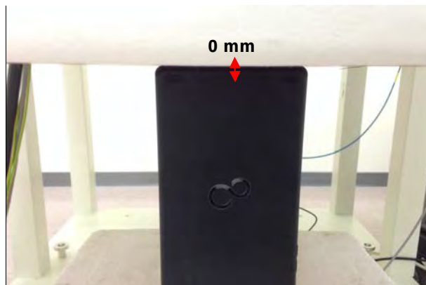
Fig.4 Top side to flat phantom
