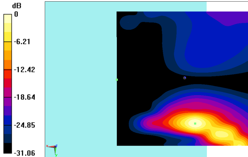
Fig B.1 T-Coil GSM850
