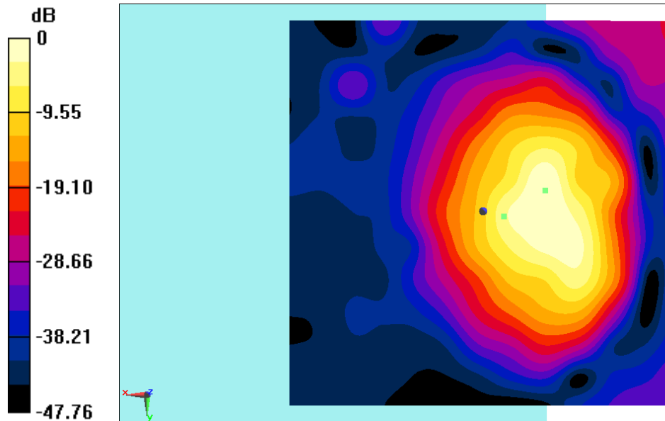
Fig B.4 T-Coil GSM850
