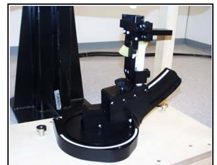
Device Holder
