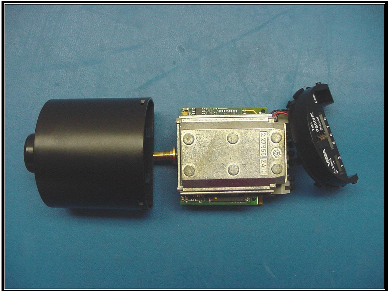
PHOTOGRAPH 27: EUT MODULE PARTS INSIDE VIEW
