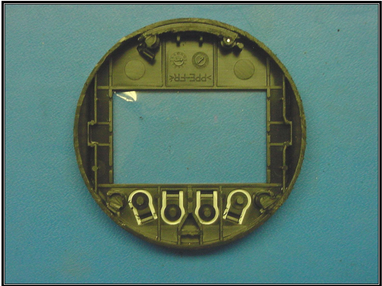
PHOTOGRAPH 20: EUT LCD DISPLAY INSIDE VIEW
