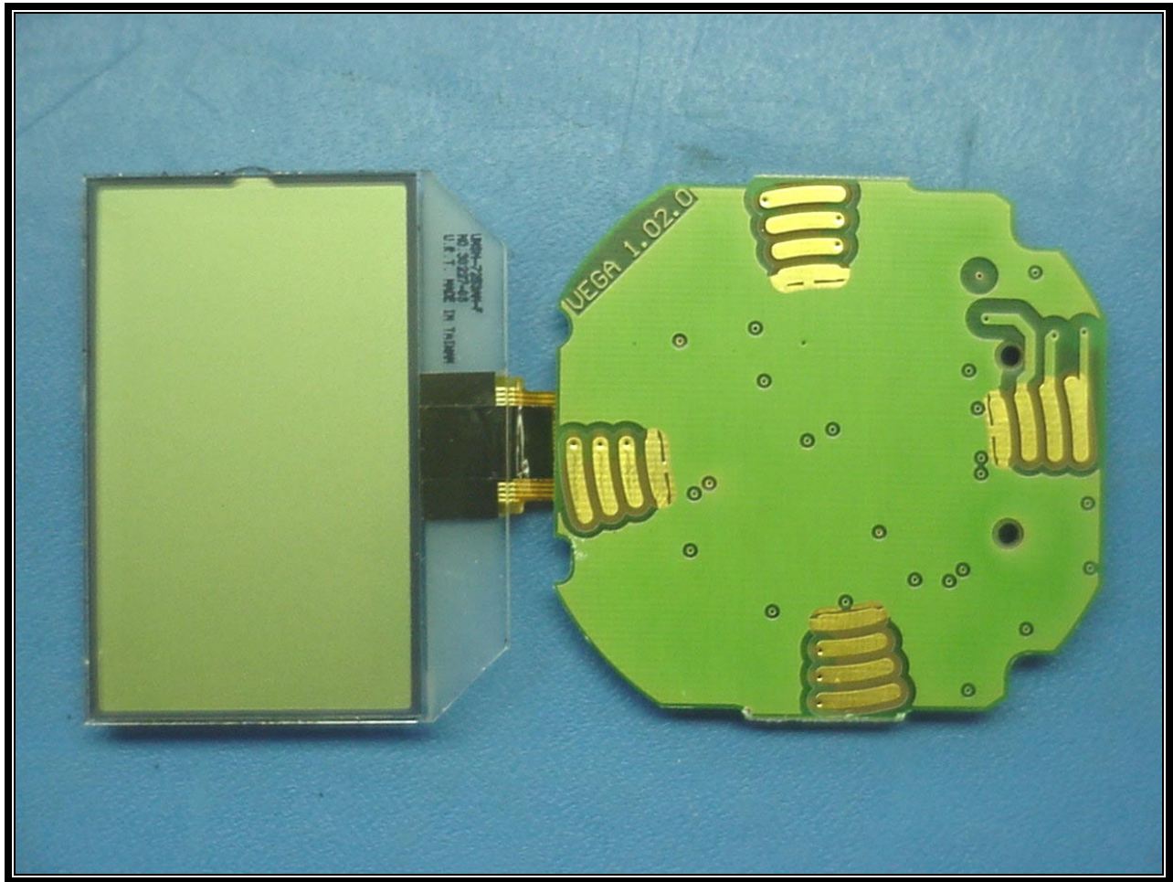
PHOTOGRAPH 21: EUT LCD DISPLAY – PCB BOTTOM VIEW
