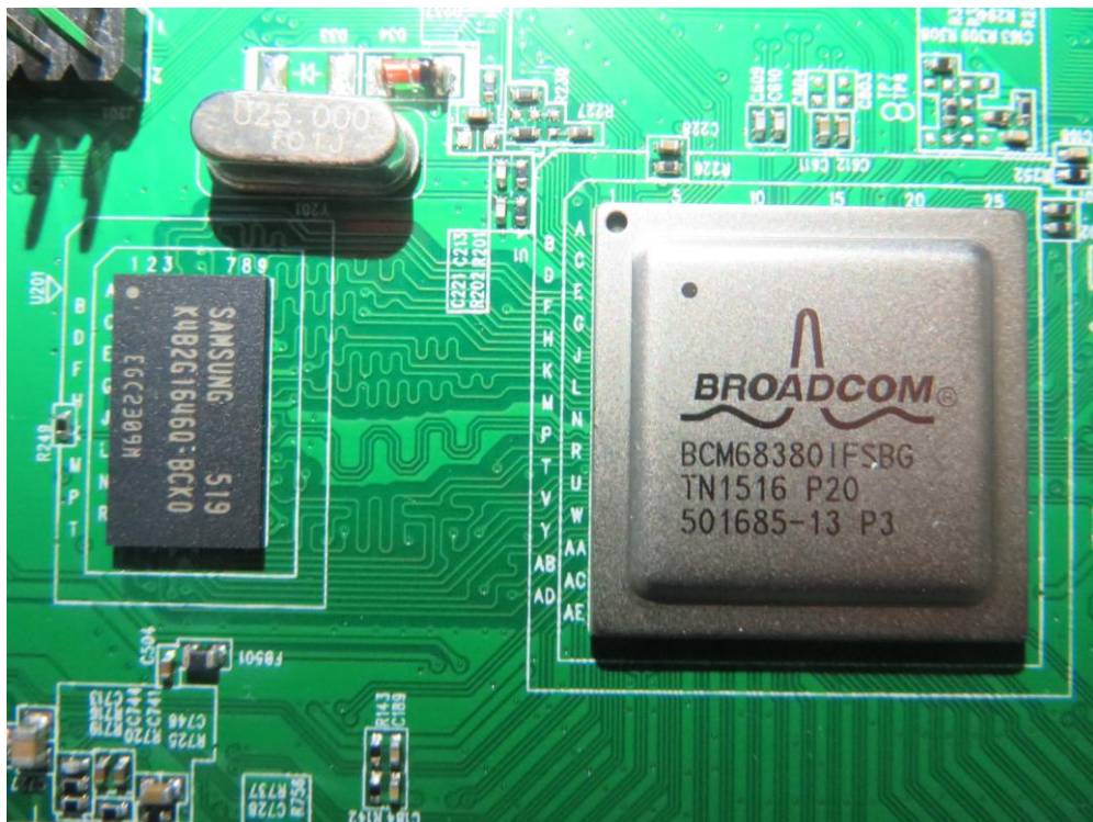
(6) EUT Photo (844GE-2)
