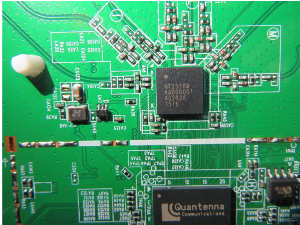
(9) EUT Photo (844GE-2)
