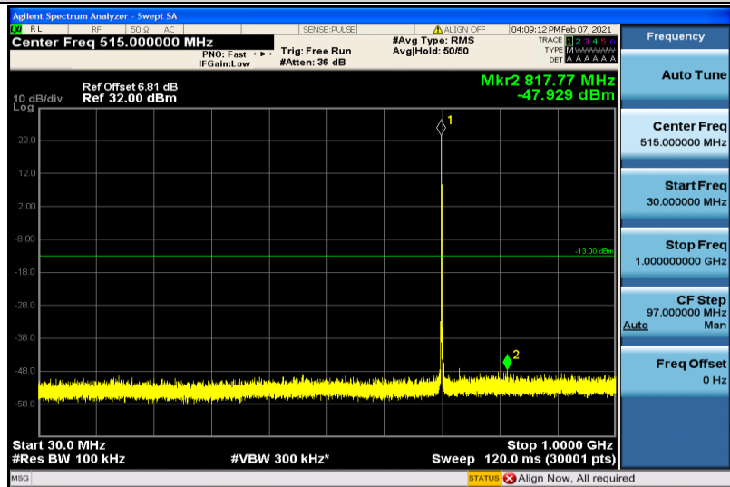
Band12-1.4MHz-QPSK-23095-1RB#0-30~1000MHz
