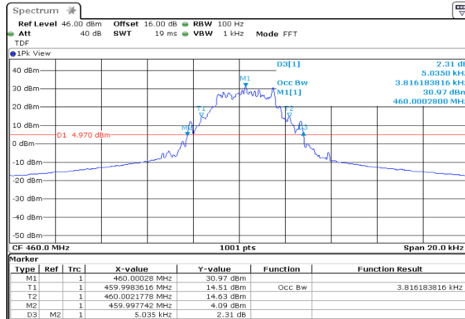
Plot 7.2.3 Occupied bandwidth test result at high frequency
