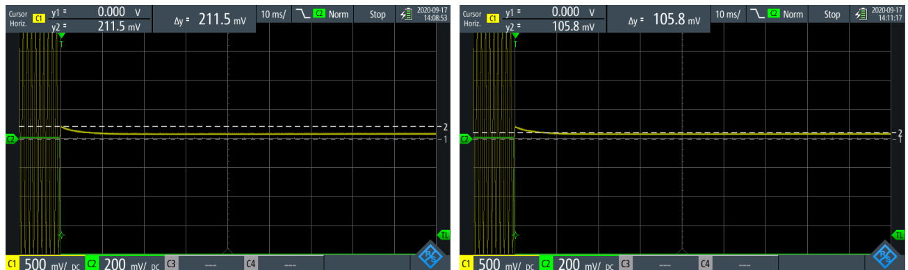
Plot 7.6.2 Transient frequency during power OFF test results at low carrier frequency
