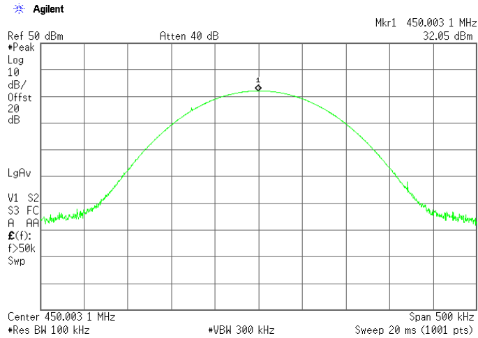
Plot 7.1.2 Peak output power at mid frequency and Unom
