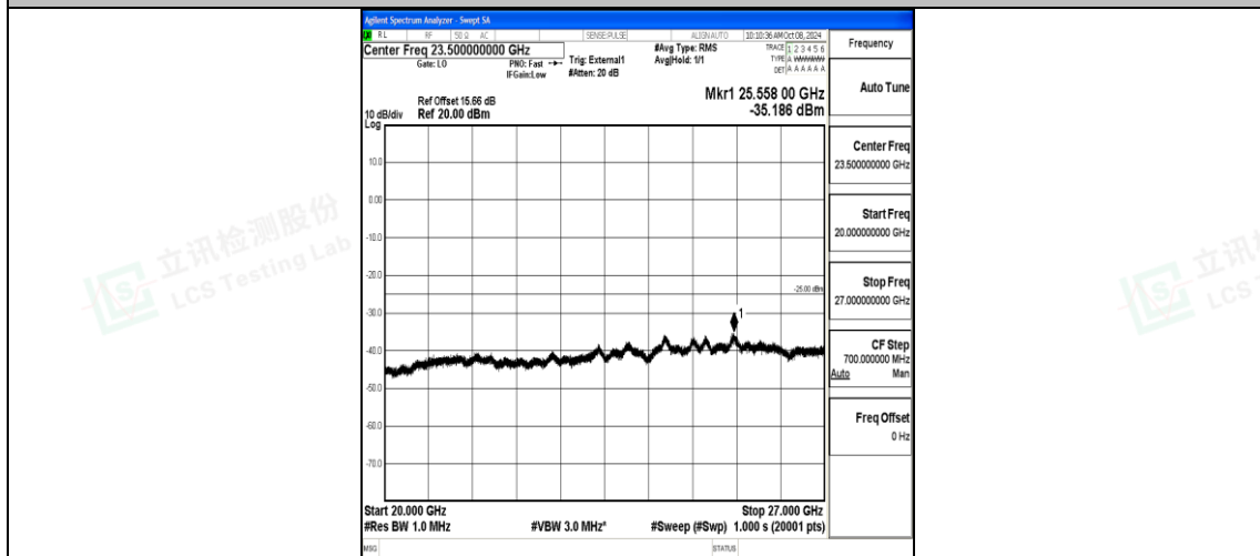
Band38_15MHz_16QAM_38175_1RB#0_20000~27000_20000~27000
