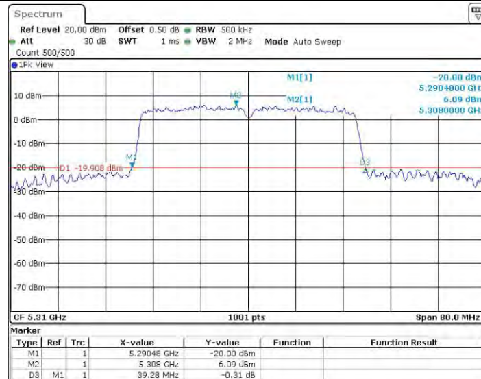
11AC40SISO_Ant0_5310
