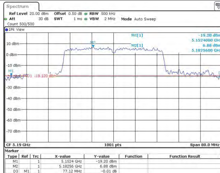
11AC40SISO_Ant0_5190
