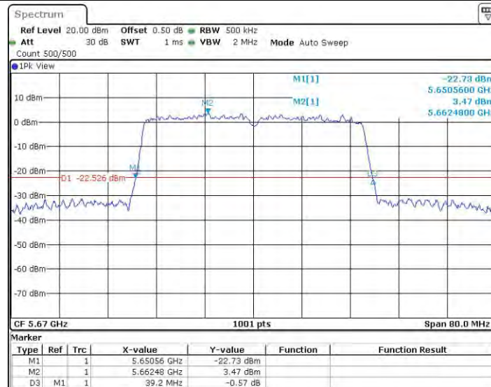
11AC40SISO_Ant0_5670
