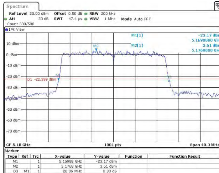
11AX20SISO_Ant1_5180
