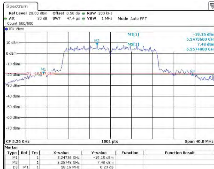
11AC20SISO_Ant0_5260
