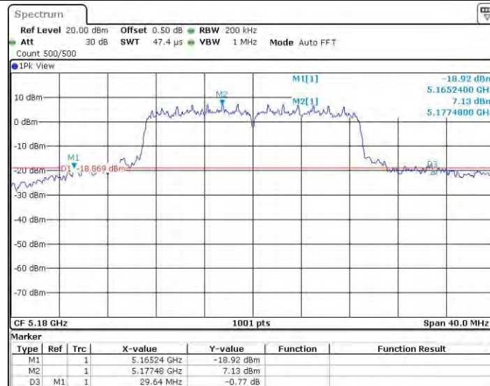
11N20SISO_Ant0_5180
