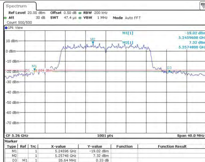
11N20SISO_Ant0_5260
