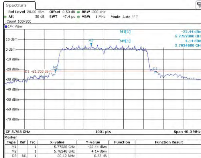
11N20SISO_Ant0_5785
