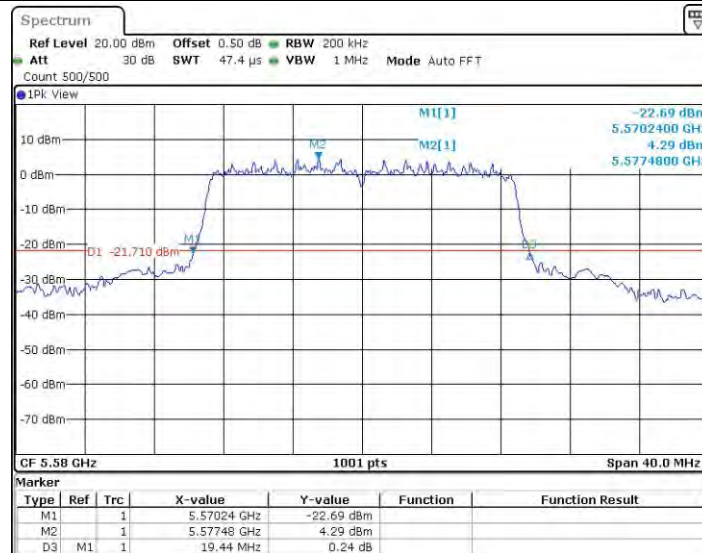
11AC20SISO_Ant1_5580
