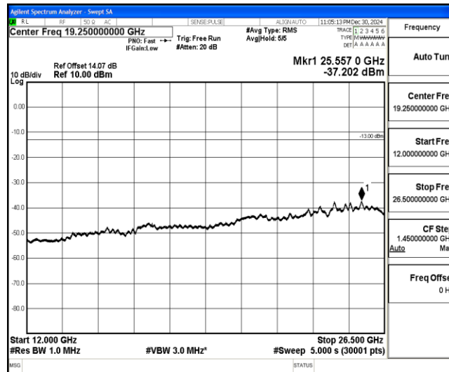
Band4-5MHz-16QAM-20175-1-0-Low-12000-26500--37.2-PASS
