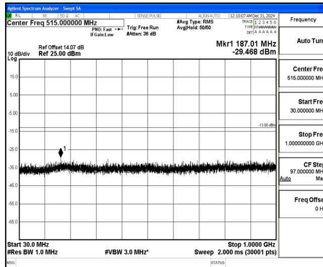
Band4-20MHz-QPSK-20300-1-0-High-30-1000--29.47-PASS
