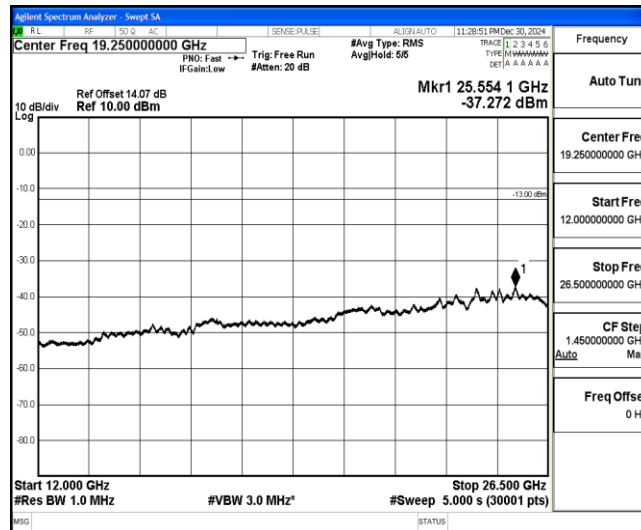
Band4-10MHz-QPSK-20350-1-0-High-12000-26500--37.27-PASS
