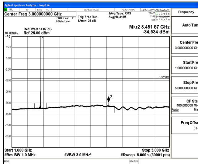
Band4-15MHz-16QAM-20175-1-0-Low-1000-5000--34.53-PASS
