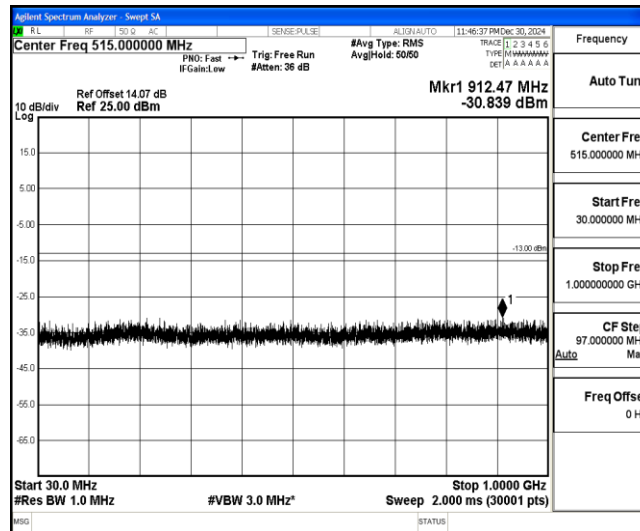
Band4-15MHz-16QAM-20175-1-0-Low-30-1000--30.84-PASS
