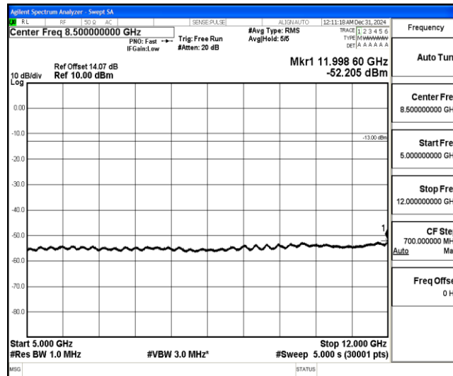
Band4-20MHz-QPSK-20300-1-0-High-5000-12000--52.21-PASS
