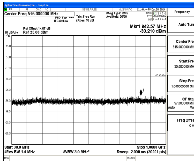
Band4-15MHz-QPSK-20175-1-0-Low-30-1000--30.21-PASS
