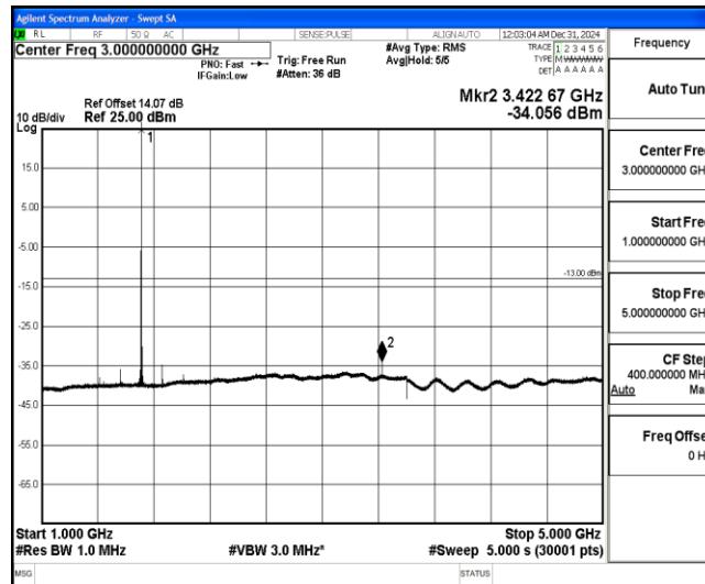
Band4-20MHz-QPSK-20050-1-0-Low-1000-5000--34.06-PASS
