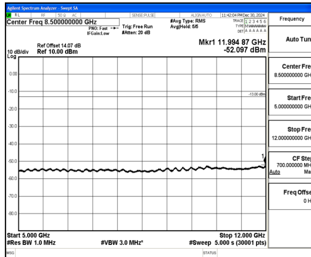
Band4-15MHz-QPSK-20025-1-0-Low-5000-12000--52.1-PASS
