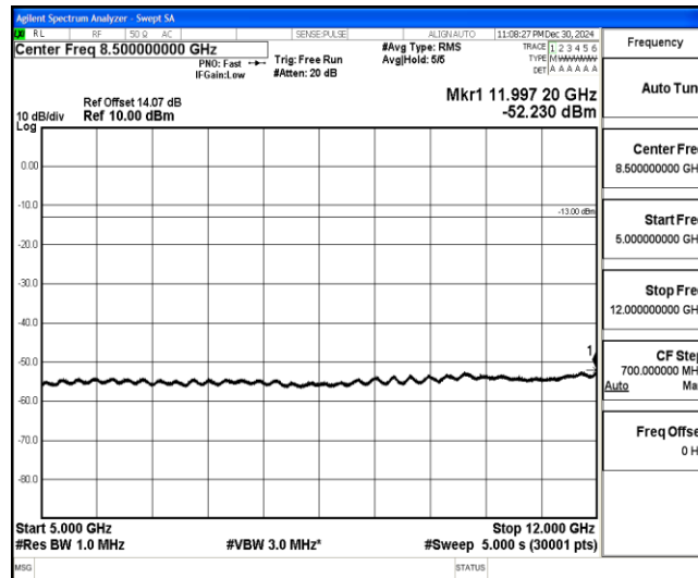
Band4-5MHz-16QAM-20375-1-0-High-5000-12000--52.23-PASS
