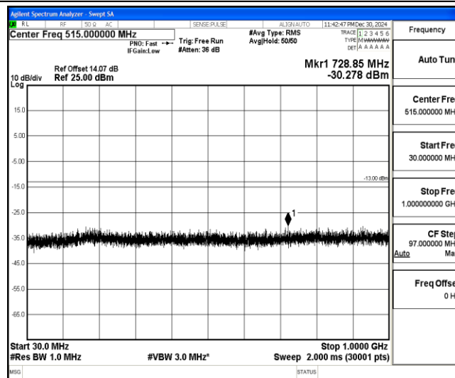
Band4-15MHz-16QAM-20025-1-0-Low-30-1000--30.28-PASS
