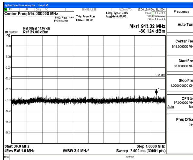
Band4-20MHz-QPSK-20175-1-0-Low-30-1000--30.12-PASS
