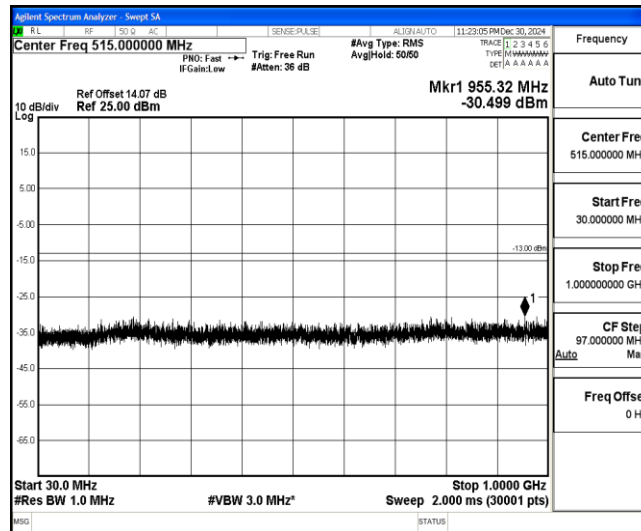
Band4-10MHz-QPSK-20175-1-0-Low-30-1000--30.5-PASS
