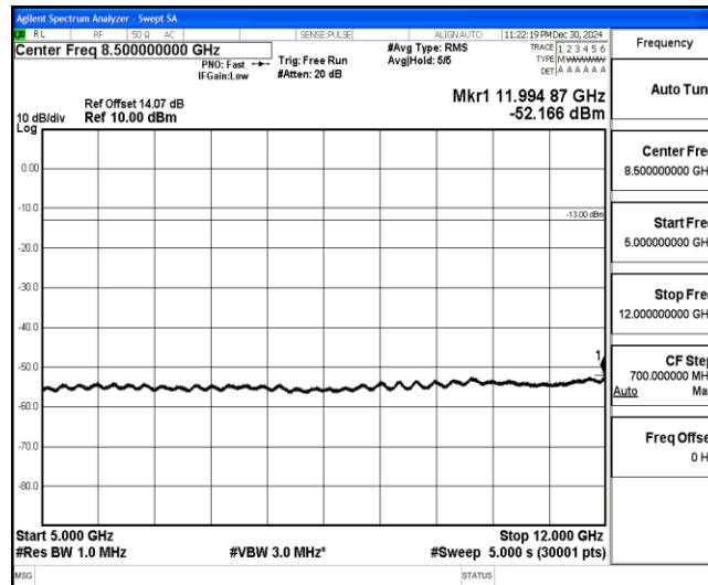
Band4-10MHz-16QAM-20000-1-0-Low-5000-12000--52.17-PASS
