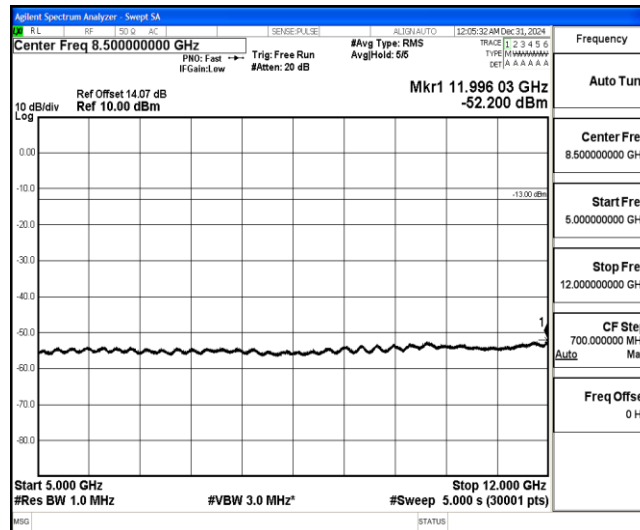
Band4-20MHz-16QAM-20050-1-0-Low-5000-12000--52.2-PASS
