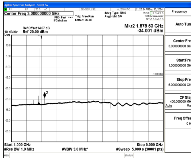
Band4-10MHz-16QAM-20175-1-0-Low-1000-5000--34-PASS
