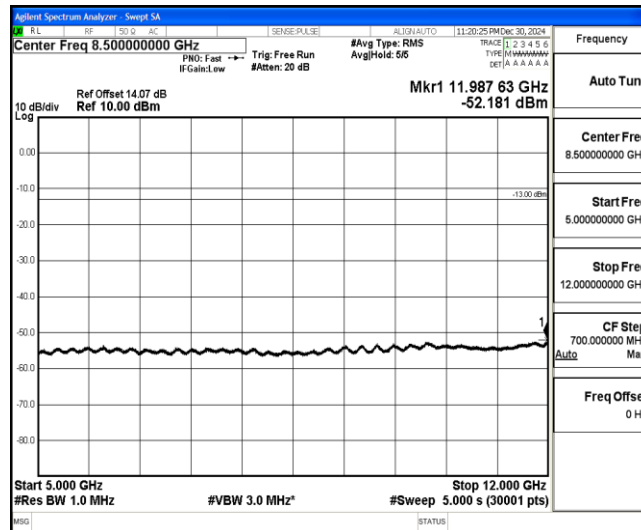
Band4-10MHz-QPSK-20000-1-0-Low-5000-12000--52.18-PASS
