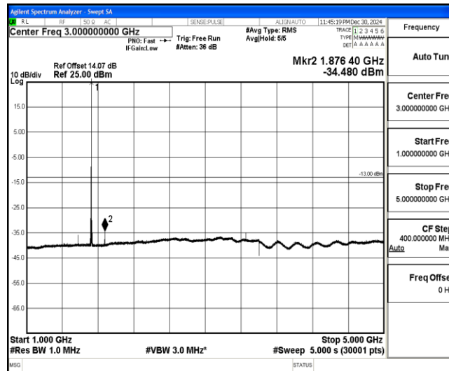
Band4-15MHz-QPSK-20175-1-0-Low-1000-5000--34.48-PASS
