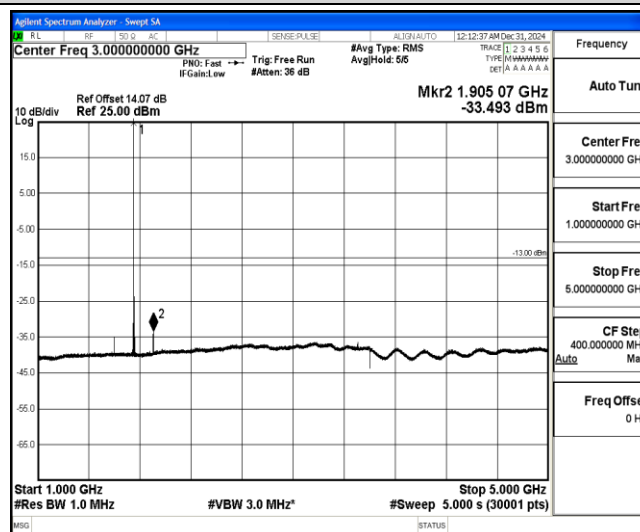
Band4-20MHz-16QAM-20300-1-0-High-1000-5000--33.49-PASS
