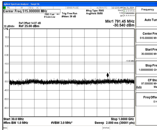
Band4-20MHz-16QAM-20300-1-0-High-30-1000--30.54-PASS
