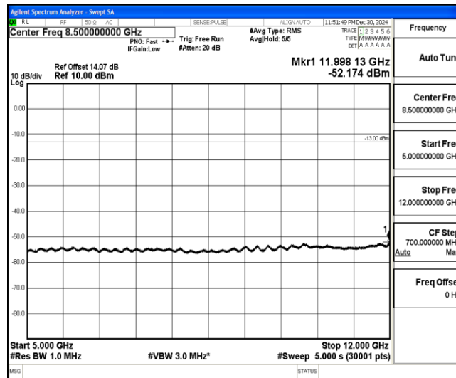
Band4-15MHz-16QAM-20325-1-0-High-5000-12000--52.17-PASS
