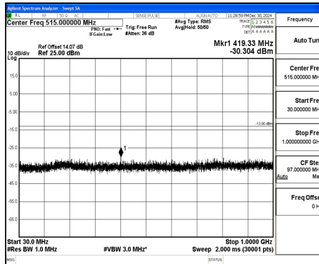
Band4-10MHz-16QAM-20350-1-0-High-30-1000--30.3-PASS
