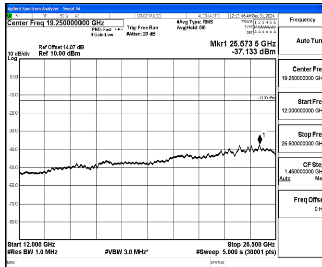
Band4-20MHz-16QAM-20300-1-0-High-12000-26500--37.13-PASS
