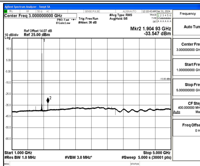
Band4-20MHz-QPSK-20300-1-0-High-1000-5000--33.55-PASS
