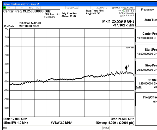
Band4-5MHz-16QAM-20375-1-0-High-12000-26500--37.16-PASS
