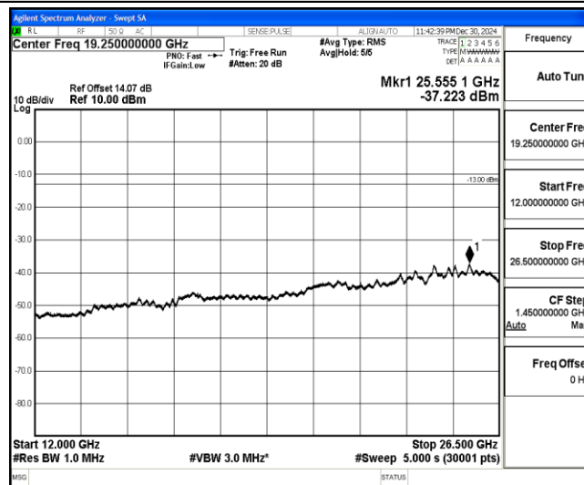
Band4-15MHz-QPSK-20025-1-0-Low-12000-26500--37.22-PASS
