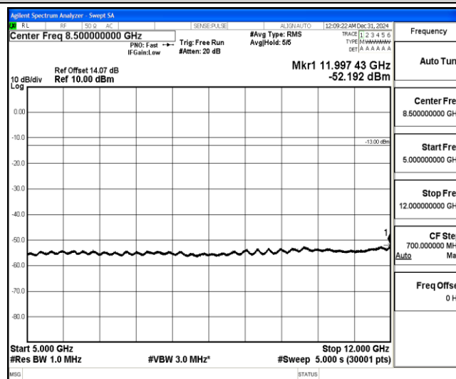
Band4-20MHz-16QAM-20175-1-0-Low-5000-12000--52.19-PASS
