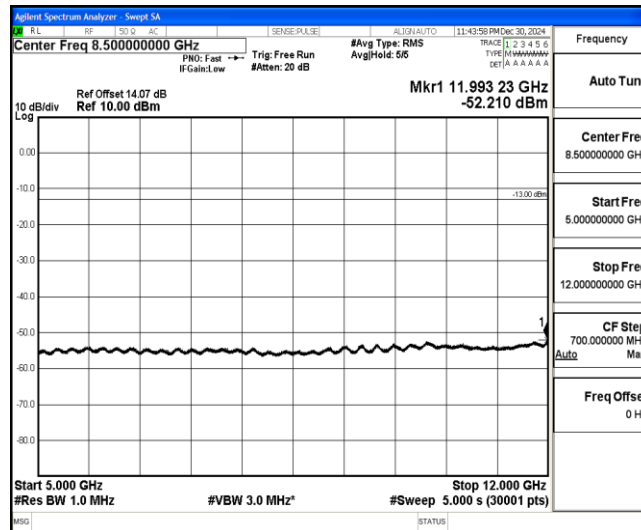
Band4-15MHz-16QAM-20025-1-0-Low-5000-12000--52.21-PASS
