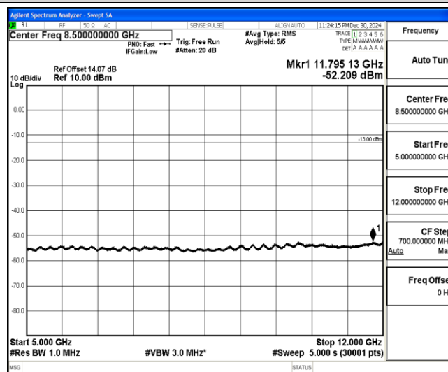
Band4-10MHz-QPSK-20175-1-0-Low-5000-12000--52.21-PASS
