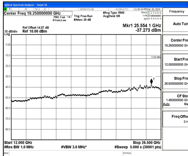
Band4-10MHz-16QAM-20175-1-0-Low-12000-26500--37.27-PASS
