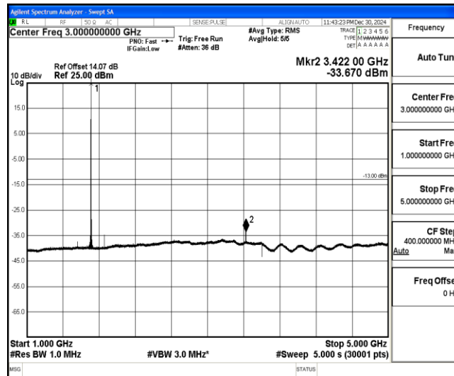
Band4-15MHz-16QAM-20025-1-0-Low-1000-5000--33.67-PASS
