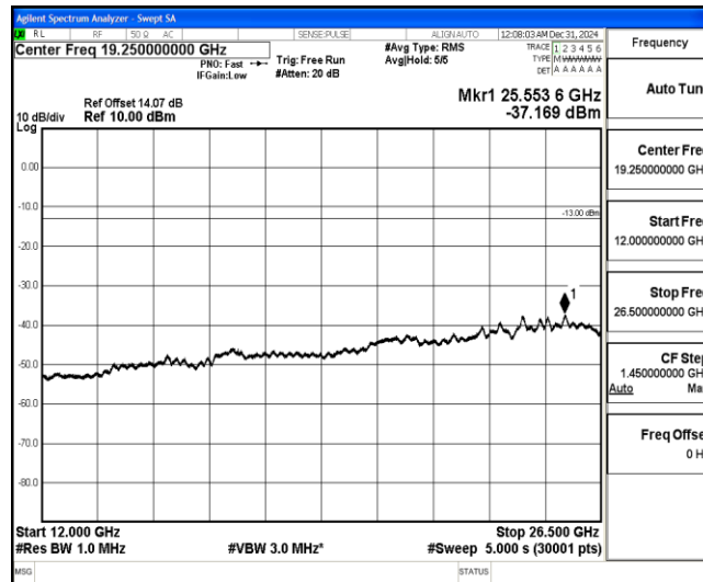
Band4-20MHz-QPSK-20175-1-0-Low-12000-26500--37.17-PASS
