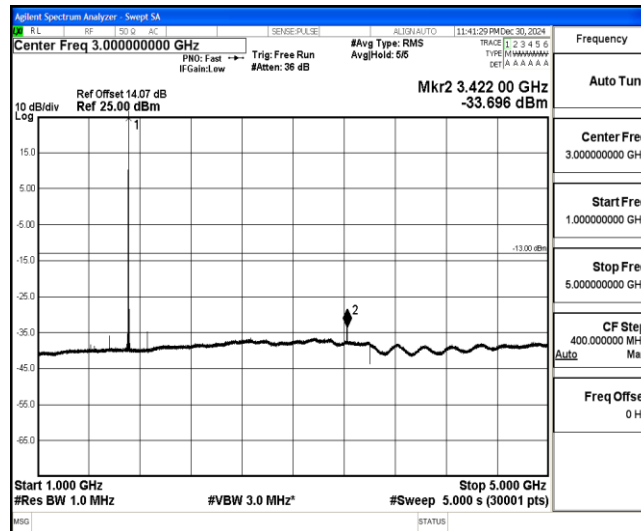
Band4-15MHz-QPSK-20025-1-0-Low-1000-5000--33.7-PASS
