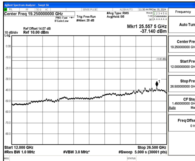
Band4-10MHz-16QAM-20350-1-0-High-12000-26500--37.14-PASS
