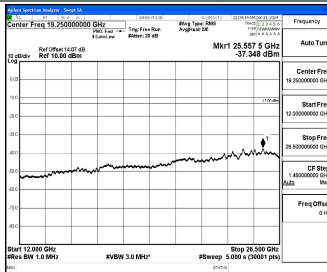
Band4-20MHz-QPSK-20050-1-0-Low-12000-26500--37.35-PASS
