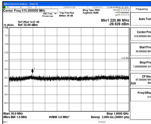
Band4-15MHz-QPSK-20325-1-0-High-30-1000--29.63-PASS
