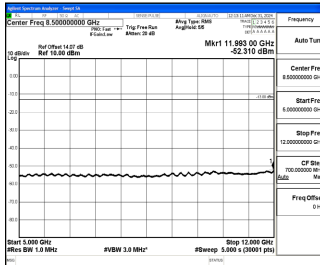
Band4-20MHz-16QAM-20300-1-0-High-5000-12000--52.31-PASS
