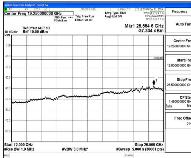
Band4-20MHz-QPSK-20300-1-0-High-12000-26500--37.33-PASS
