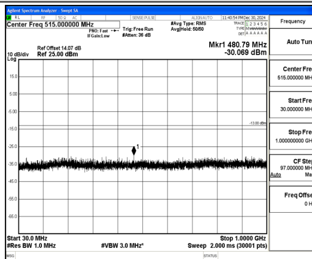
Band4-15MHz-QPSK-20025-1-0-Low-30-1000--30.07-PASS
