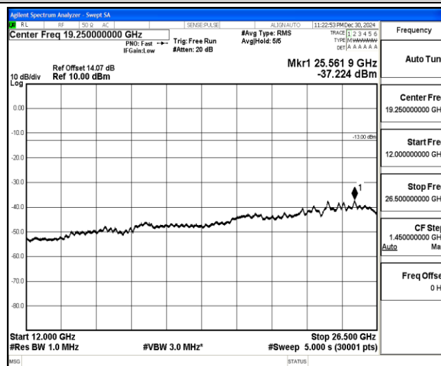
Band4-10MHz-16QAM-20000-1-0-Low-12000-26500--37.22-PASS
