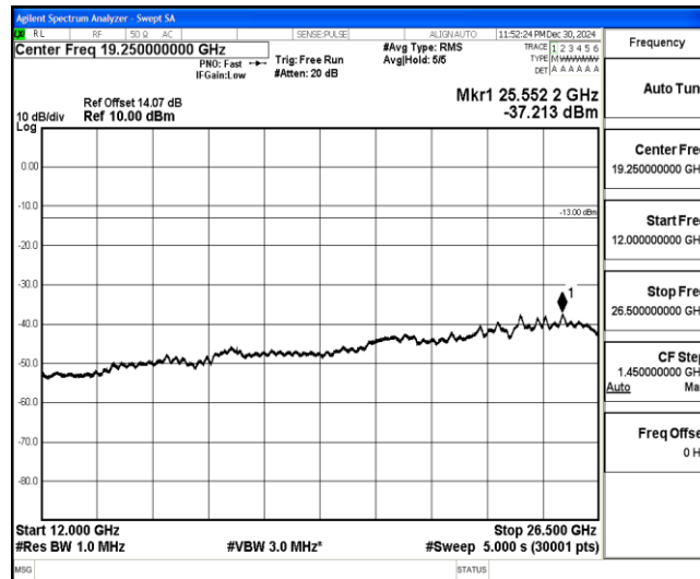
Band4-15MHz-16QAM-20325-1-0-High-12000-26500--37.21-PASS
