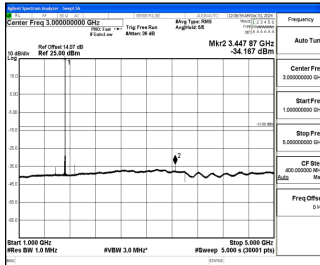
Band4-20MHz-QPSK-20175-1-0-Low-1000-5000--34.17-PASS
