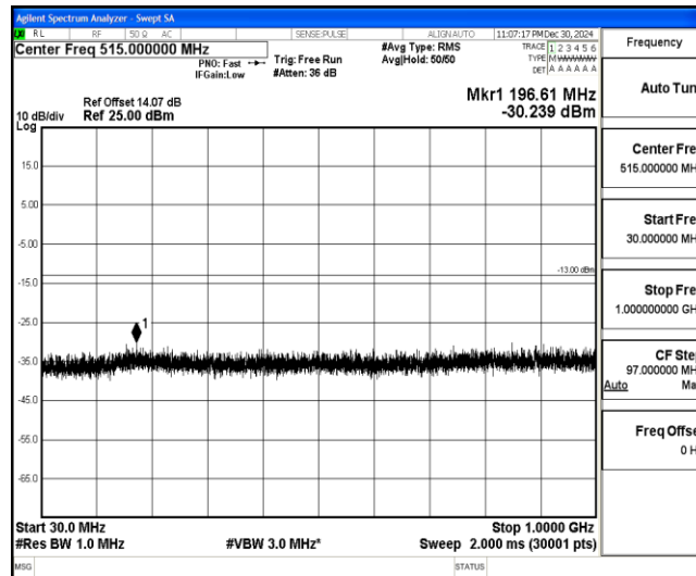
Band4-5MHz-16QAM-20375-1-0-High-30-1000--30.24-PASS
