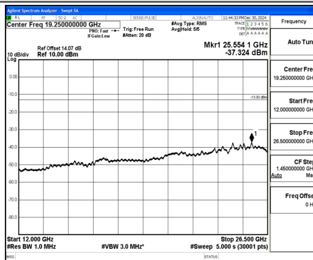
Band4-15MHz-16QAM-20025-1-0-Low-12000-26500--37.32-PASS
