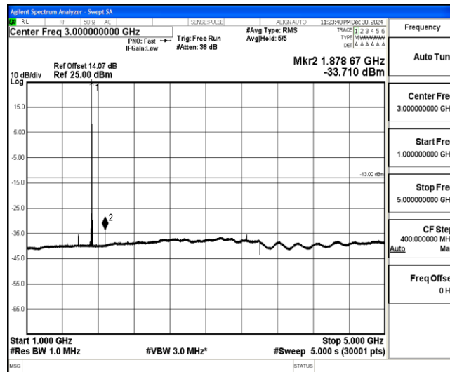
Band4-10MHz-QPSK-20175-1-0-Low-1000-5000--33.71-PASS
