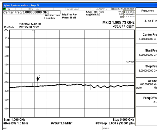
Band4-10MHz-16QAM-20350-1-0-High-1000-5000--33.68-PASS
