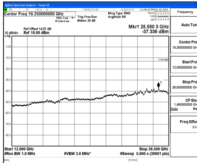
Band4-15MHz-16QAM-20175-1-0-Low-12000-26500--37.34-PASS
