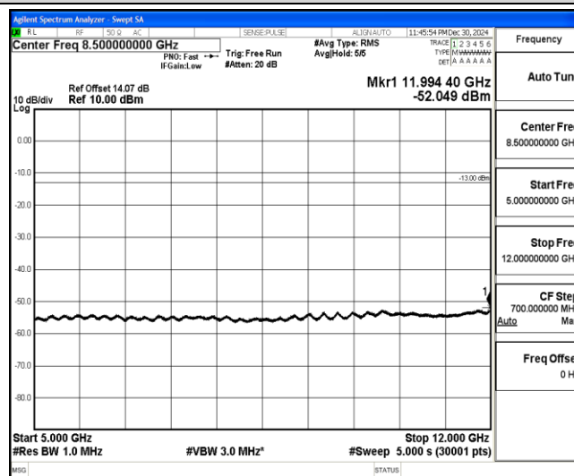
Band4-15MHz-QPSK-20175-1-0-Low-5000-12000--52.05-PASS
