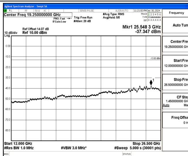
Band4-10MHz-QPSK-20000-1-0-Low-12000-26500--37.35-PASS
