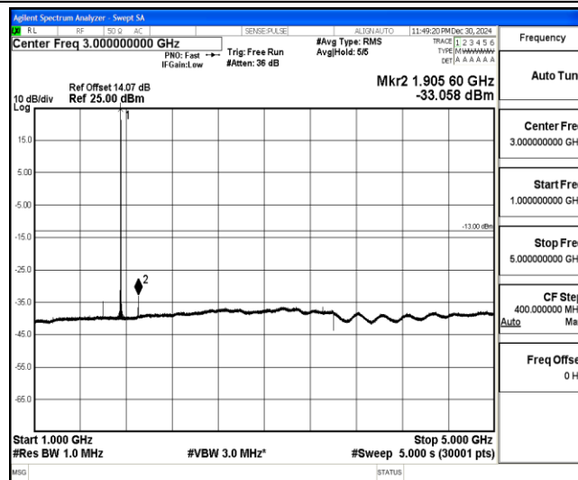
Band4-15MHz-QPSK-20325-1-0-High-1000-5000--33.06-PASS
