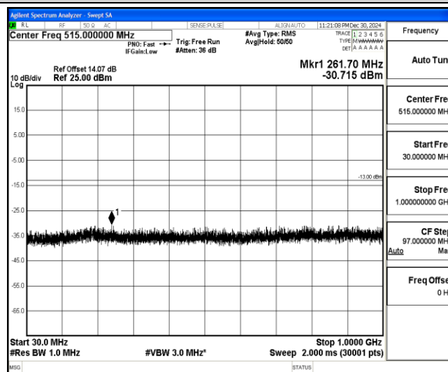
Band4-10MHz-16QAM-20000-1-0-Low-30-1000--30.72-PASS
