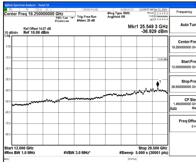
Band4-20MHz-16QAM-20175-1-0-Low-12000-26500--36.93-PASS
