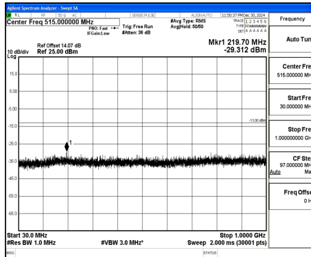
Band4-15MHz-16QAM-20325-1-0-High-30-1000--29.31-PASS
