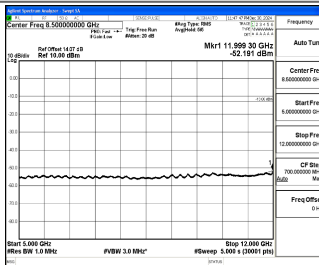
Band4-15MHz-16QAM-20175-1-0-Low-5000-12000--52.19-PASS
