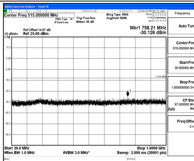
Band4-20MHz-16QAM-20050-1-0-Low-30-1000--30.13-PASS
