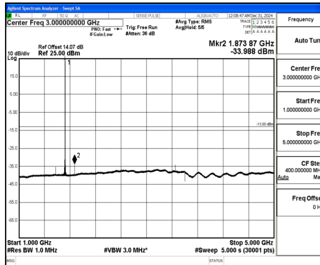
Band4-20MHz-16QAM-20175-1-0-Low-1000-5000--33.99-PASS
