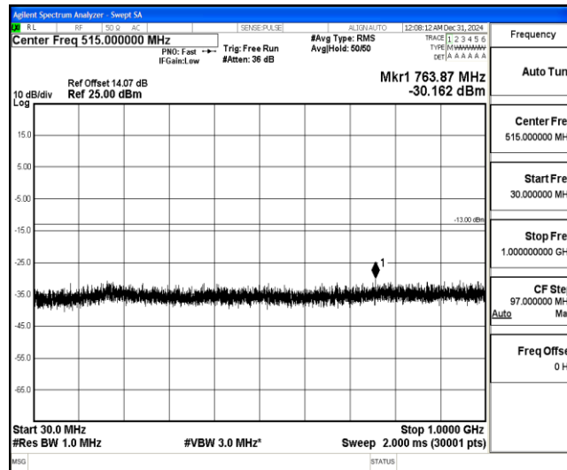
Band4-20MHz-16QAM-20175-1-0-Low-30-1000--30.16-PASS
