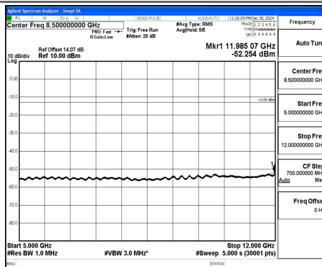
Band4-10MHz-16QAM-20175-1-0-Low-5000-12000--52.25-PASS
