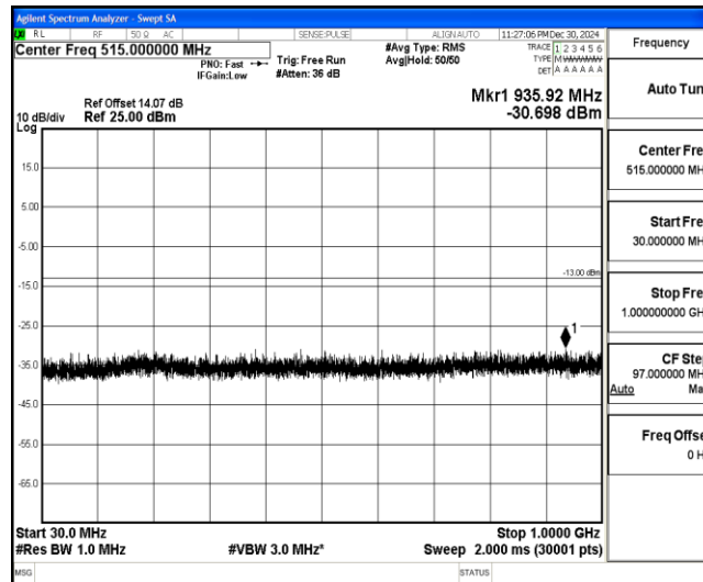
Band4-10MHz-QPSK-20350-1-0-High-30-1000--30.7-PASS
