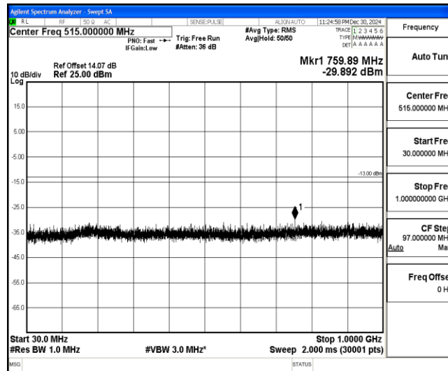
Band4-10MHz-16QAM-20175-1-0-Low-30-1000--29.89-PASS
