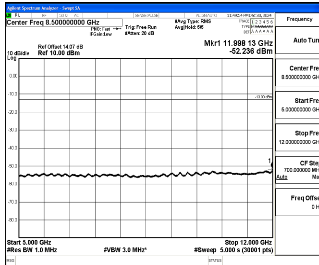
Band4-15MHz-QPSK-20325-1-0-High-5000-12000--52.24-PASS
