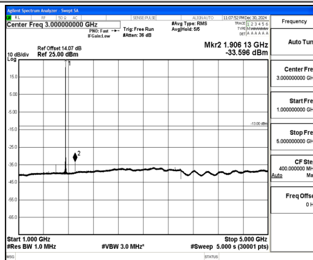
Band4-5MHz-16QAM-20375-1-0-High-1000-5000--33.6-PASS
