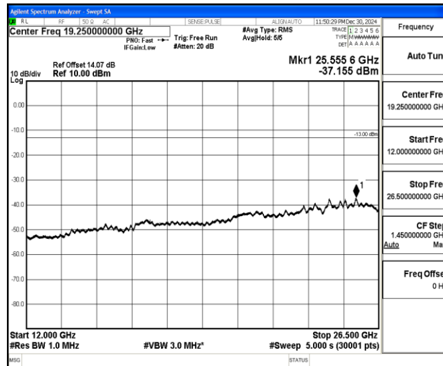
Band4-15MHz-QPSK-20325-1-0-High-12000-26500--37.16-PASS
