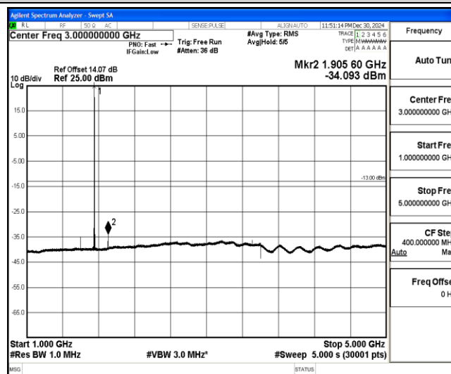
Band4-15MHz-16QAM-20325-1-0-High-1000-5000--34.09-PASS
