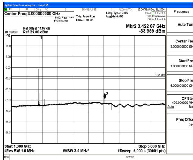
Band4-20MHz-16QAM-20050-1-0-Low-1000-5000--33.99-PASS
