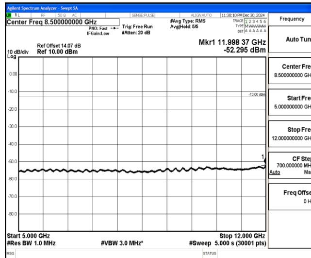
Band4-10MHz-16QAM-20350-1-0-High-5000-12000--52.3-PASS
