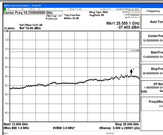
Band4-20MHz-16QAM-20050-1-0-Low-12000-26500--37.4-PASS
