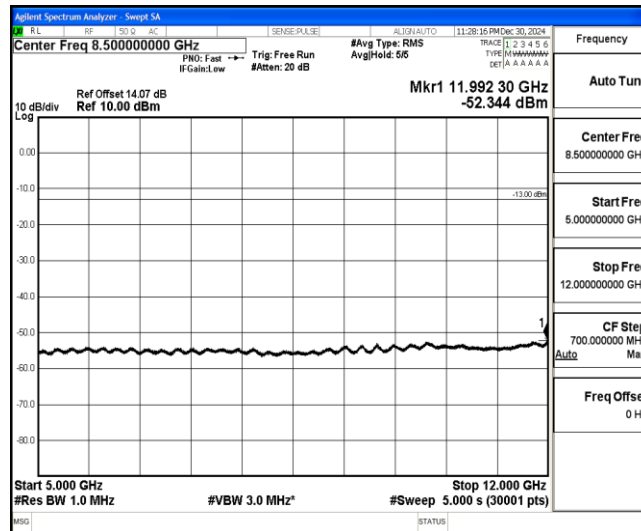
Band4-10MHz-QPSK-20350-1-0-High-5000-12000--52.34-PASS
