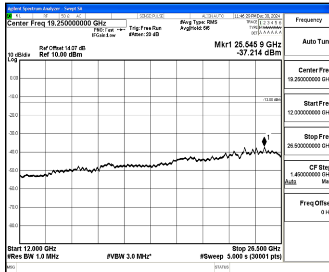
Band4-15MHz-QPSK-20175-1-0-Low-12000-26500--37.21-PASS
