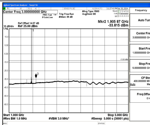
Band4-10MHz-QPSK-20350-1-0-High-1000-5000--33.82-PASS
