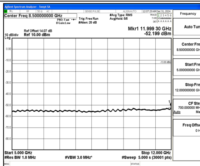
Band4-20MHz-QPSK-20175-1-0-Low-5000-12000--52.2-PASS
