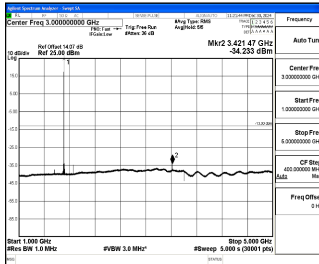
Band4-10MHz-16QAM-20000-1-0-Low-1000-5000--34.23-PASS
