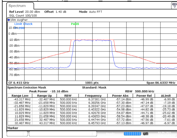
802.11ax (20MHz) 6415MHz Chain C NSS-4
