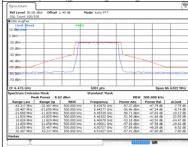
802.11ax (20MHz) 6475MHz Chain A NSS-4
