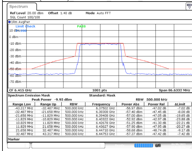
802.11ax (20MHz) 6415MHz Chain A NSS-4
