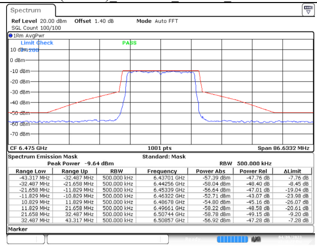
802.11ax (20MHz) 6475MHz Chain B NSS-4
