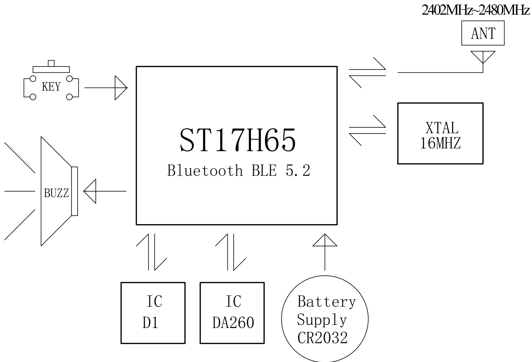
Block Diagram
