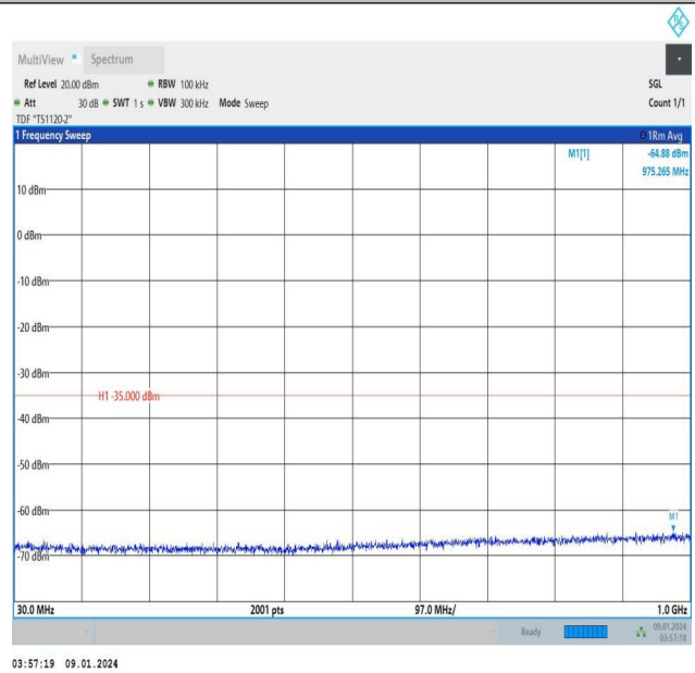
Band38_5MHz_16QAM_37775_1RB#0_30~1000_30~1000
