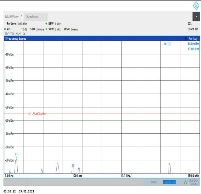
Band38_5MHz_16QAM_37775_1RB#24_0.009~0.15_0.009~0.15
