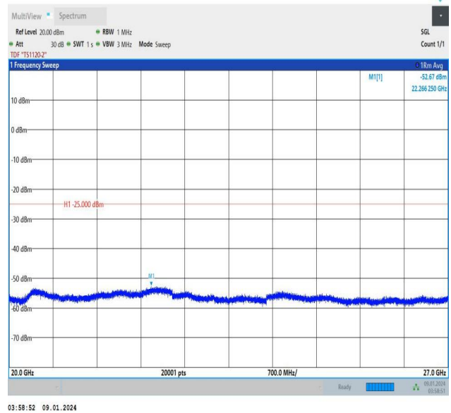
Band38_5MHz_16QAM_37775_1RB#24_20000~27000_20000~27000
