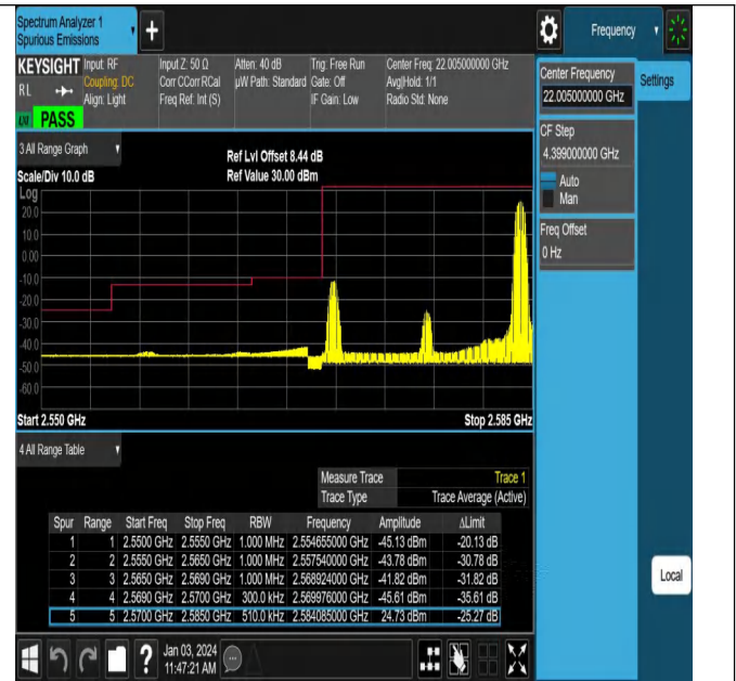
Band38_15MHz_16QAM_37825_1RB#74
