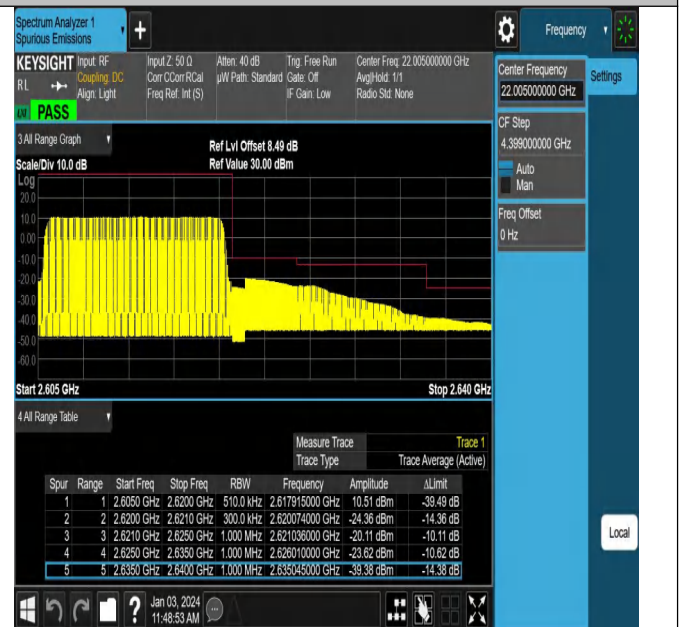
Band38_15MHz_QPSK_38175_75RB#0
