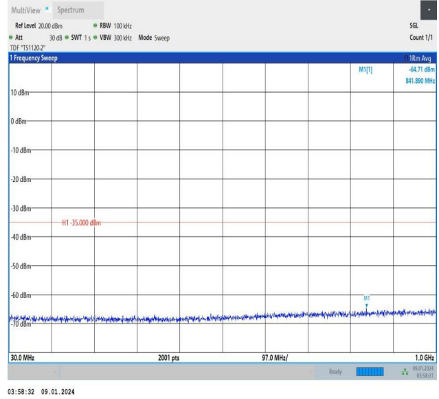
Band38_5MHz_16QAM_37775_1RB#24_30~1000_30~1000
