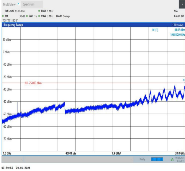
Band38_5MHz_16QAM_37775_25RB#0_1000~20000_1000~20000
