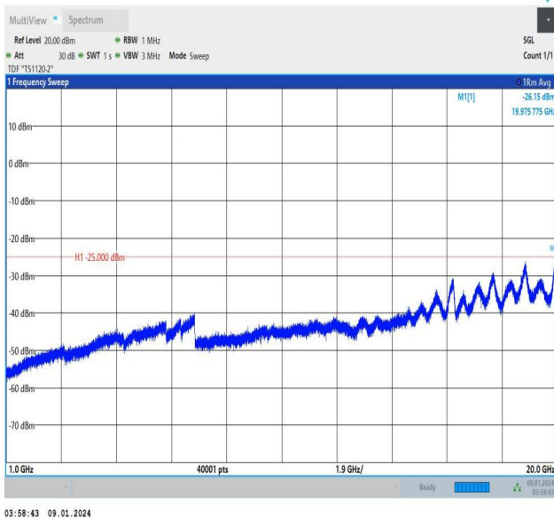
Band38_5MHz_16QAM_37775_1RB#24_1000~20000_1000~20000
