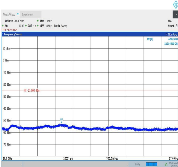
Band38_5MHz_QPSK_38000_1RB#0_20000~27000_20000~27000
