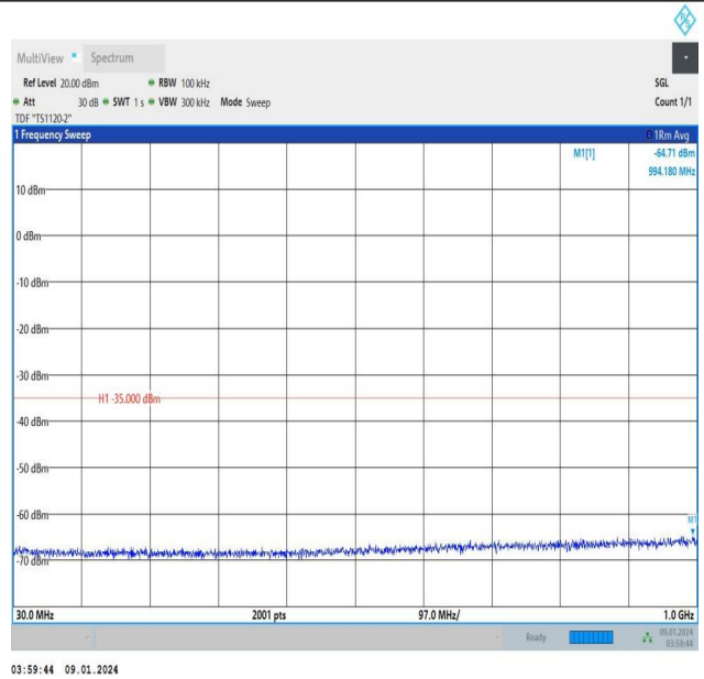
Band38_5MHz_16QAM_37775_25RB#0_30~1000_30~1000
