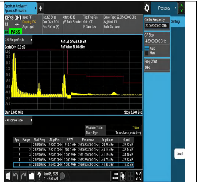
Band38_15MHz_QPSK_38175_1RB#0
