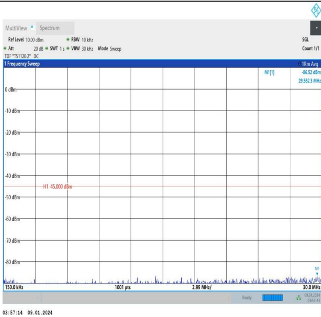
Band38_5MHz_16QAM_37775_1RB#0_0.15~30_0.15~30
