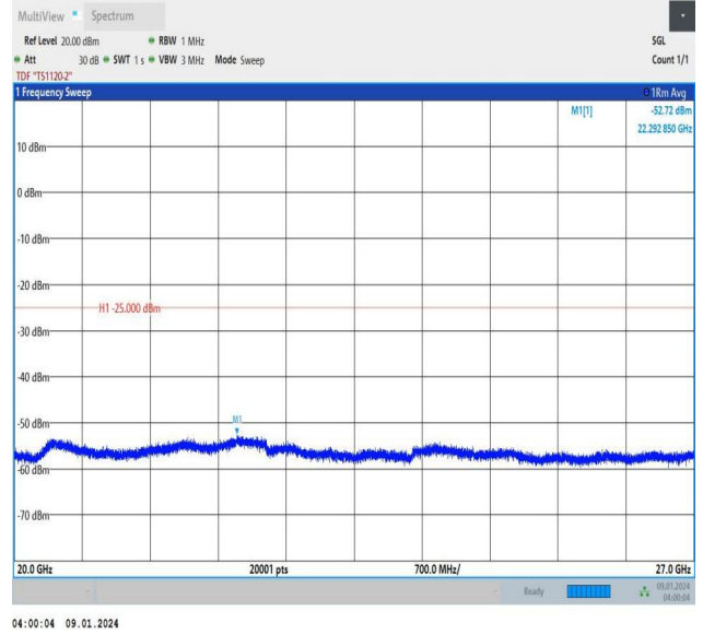
Band38_5MHz_16QAM_37775_25RB#0_20000~27000_20000~27000
