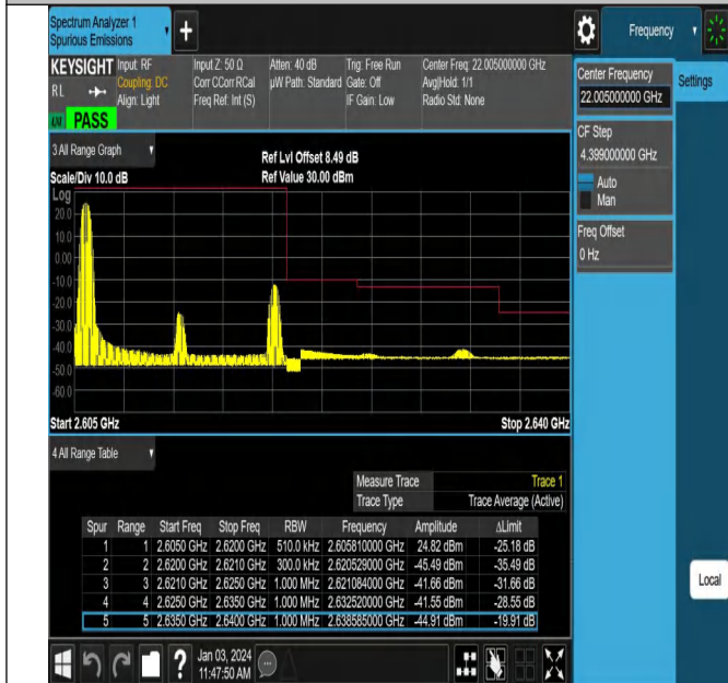
Band38_15MHz_16QAM_38175_1RB#0
