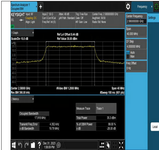
Band38-20MHz-QPSK-37850-100RB#0-PASS
