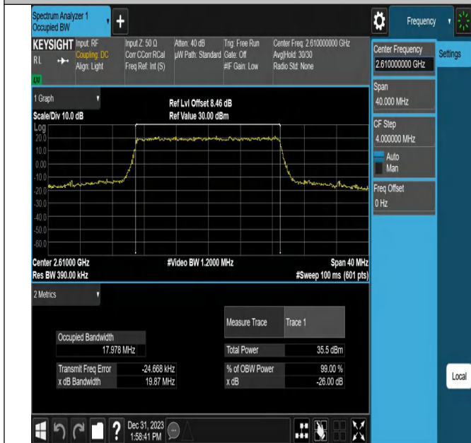
Band38-20MHz-QPSK-38150-100RB#0-PASS
