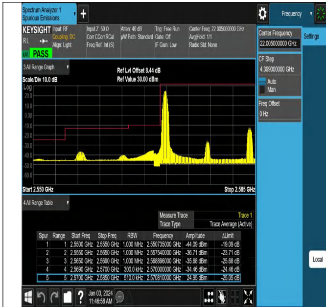
Band38_15MHz_16QAM_37825_1RB#0
