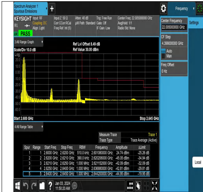
Band38_20MHz_16QAM_38150_1RB#0
