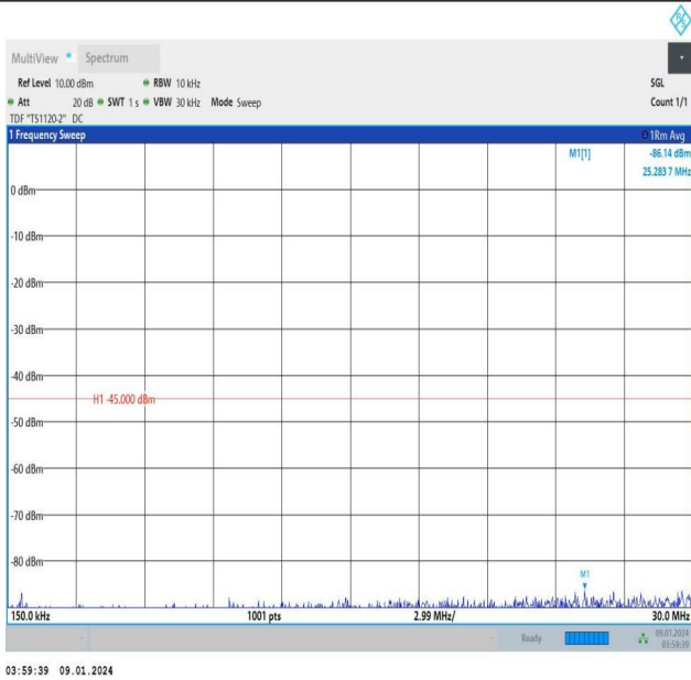
Band38_5MHz_16QAM_37775_25RB#0_0.15~30_0.15~30
