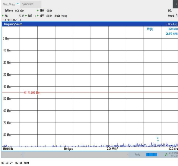
Band38_5MHz_16QAM_37775_1RB#24_0.15~30_0.15~30
