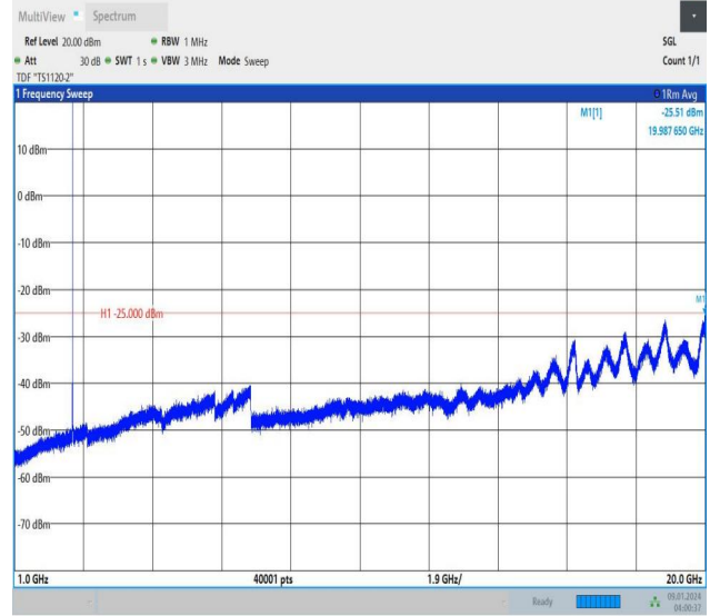
Band38_5MHz_QPSK_38000_1RB#0_1000~20000_1000~20000
