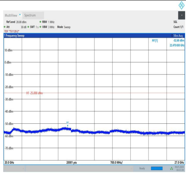
Band38_5MHz_16QAM_37775_1RB#0_20000~27000_20000
