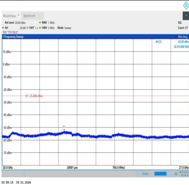
Band38_5MHz_QPSK_37775_1RB#24_20000~27000_20000~27000
