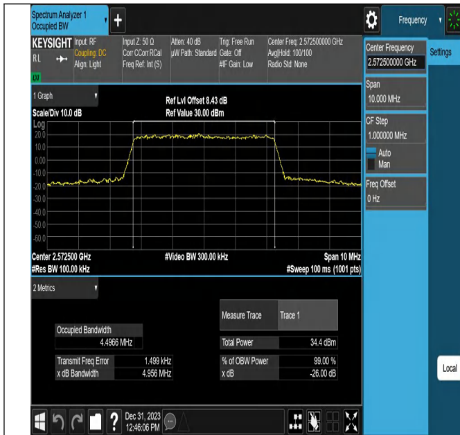
Band38-5MHz-QPSK-37775-25RB#0-PASS
