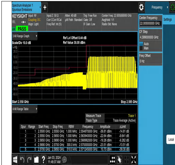
Band38_15MHz_QPSK_37825_75RB#0
