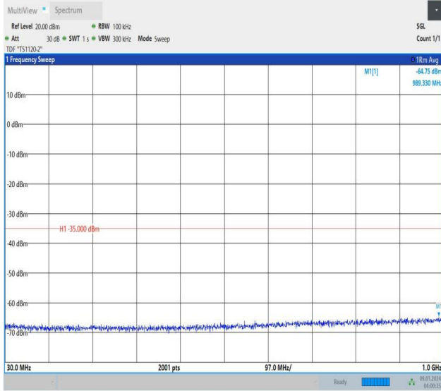
Band38_5MHz_QPSK_38000_1RB#0_30~1000_30~1000
