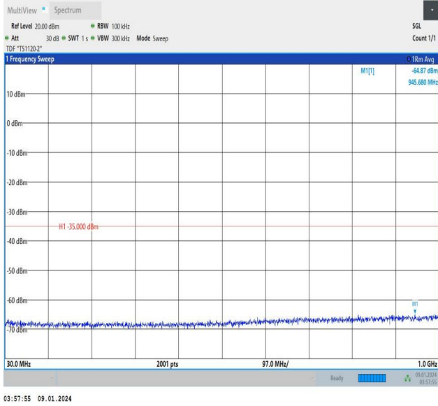
Band38_5MHz_QPSK_37775_1RB#24_30~1000_30~1000
