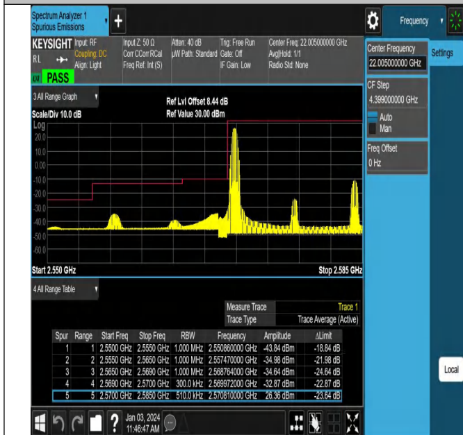
Band38_15MHz_QPSK_37825_1RB#0
