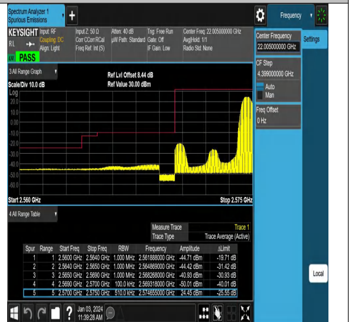
Band38_5MHz_16QAM_37775_1RB#24
