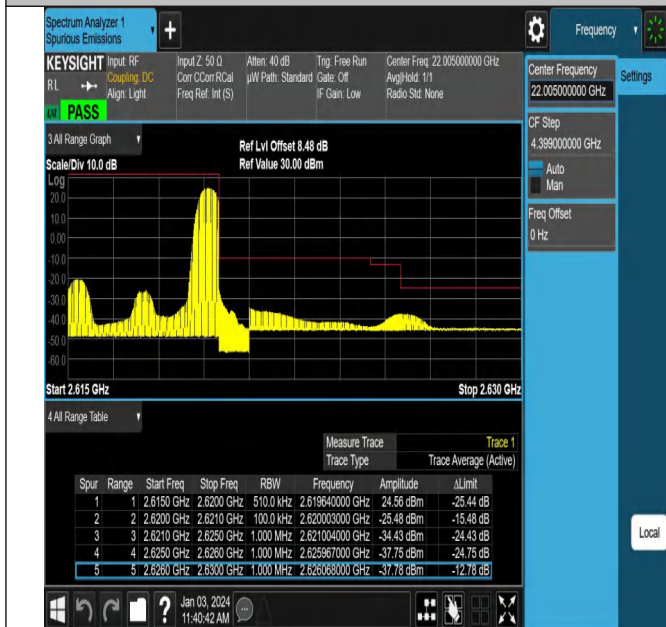
Band38_5MHz_16QAM_38225_1RB#24
