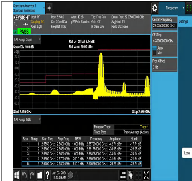
Band38_10MHz_QPSK_37800_1RB#0
