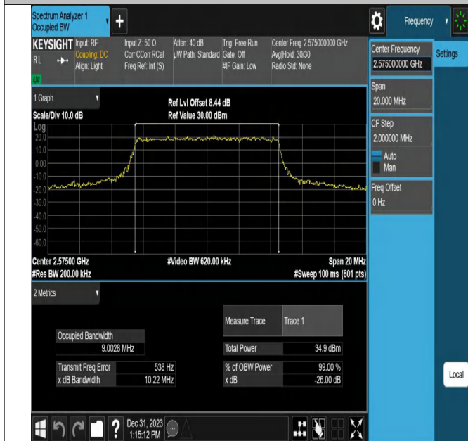
Band38-10MHz-QPSK-37800-50RB#0-PASS
