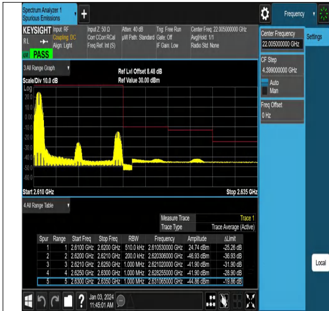
Band38_10MHz_16QAM_38200_1RB#0
