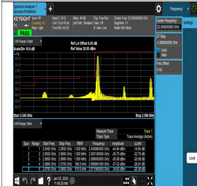
Band38_20MHz_16QAM_37850_1RB#0
