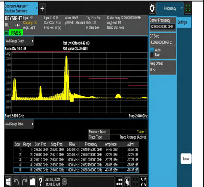
Band38_15MHz_16QAM_38175_1RB#74
