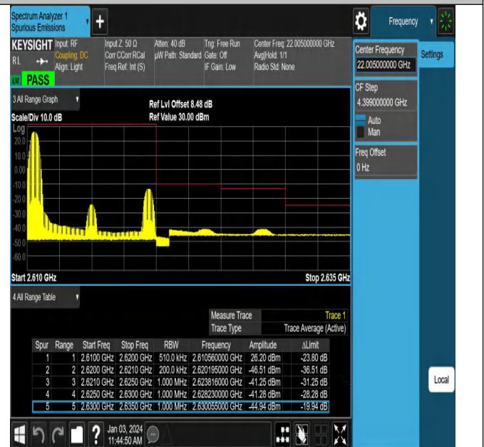
Band38_10MHz_QPSK_38200_1RB#0
