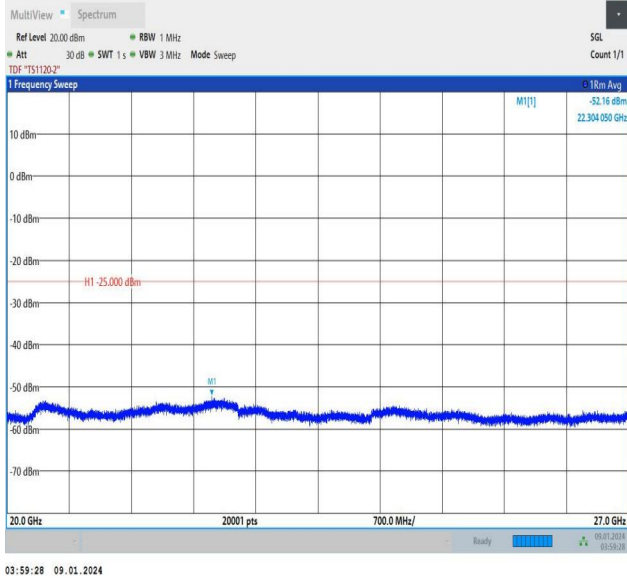
Band38_5MHz_QPSK_37775_25RB#0_20000~27000_20000~27000
