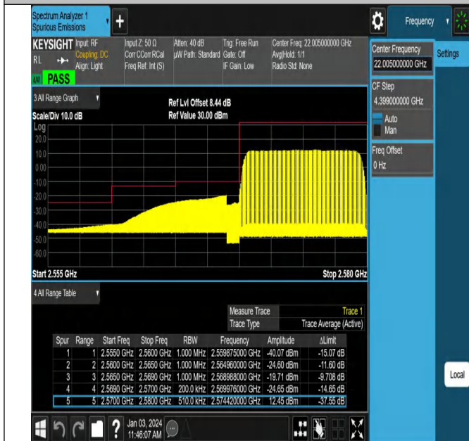
Band38_10MHz_QPSK_37800_50RB#0
