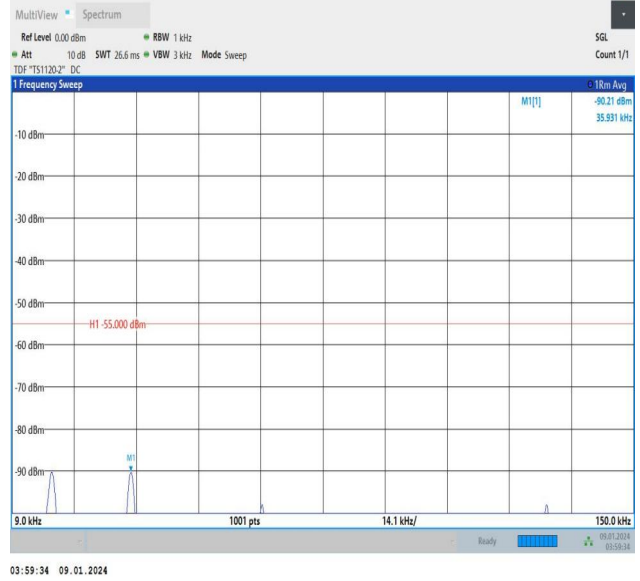
Band38_5MHz_16QAM_37775_25RB#0_0.009~0.15_0.009~0.15
