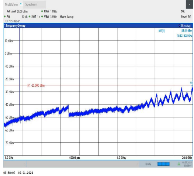
Band38_5MHz_QPSK_37775_1RB#24_1000~20000_1000~20000
