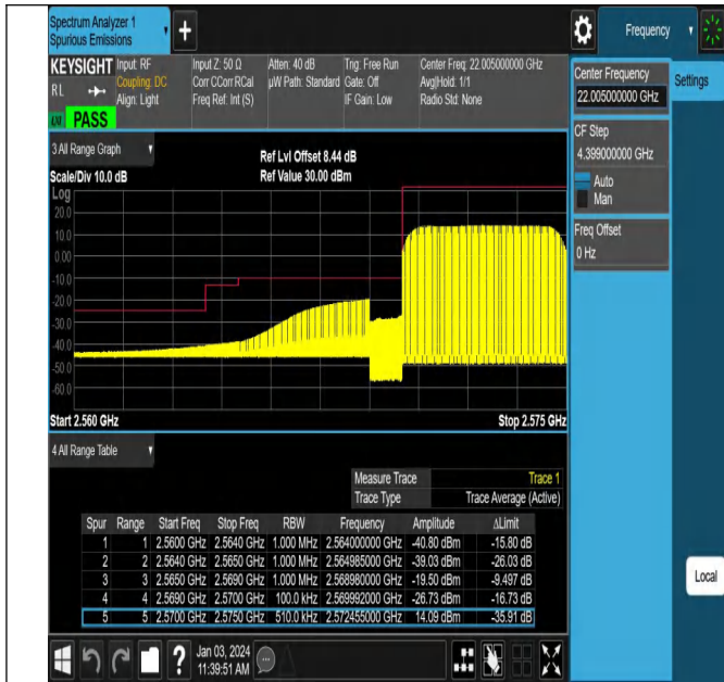
Band38_5MHz_16QAM_37775_25RB#0
