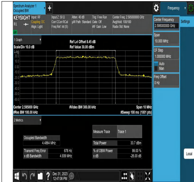
Band38-5MHz-16QAM-38000-25RB#0-PASS
