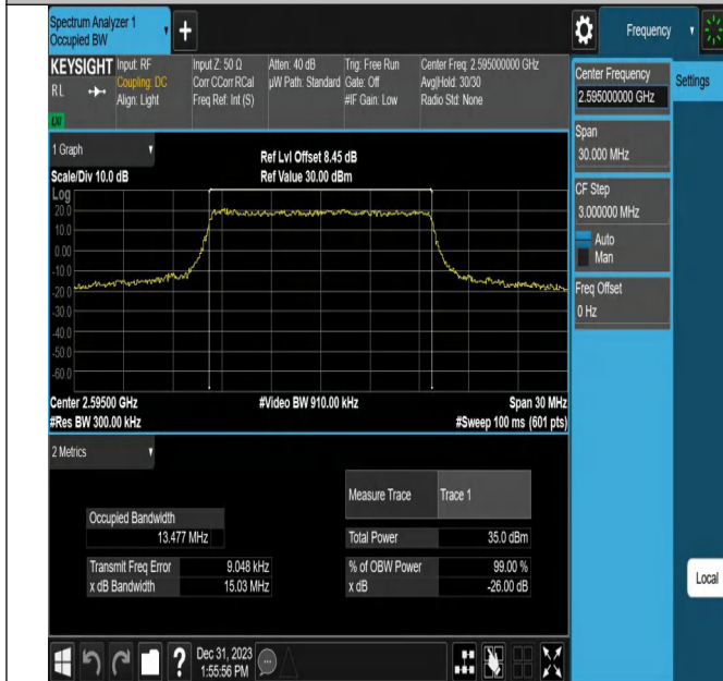
Band38-15MHz-QPSK-38000-75RB#0-PASS
