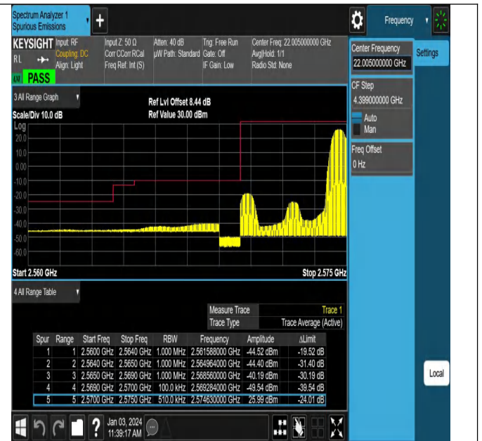
Band38_5MHz_QPSK_37775_1RB#24
