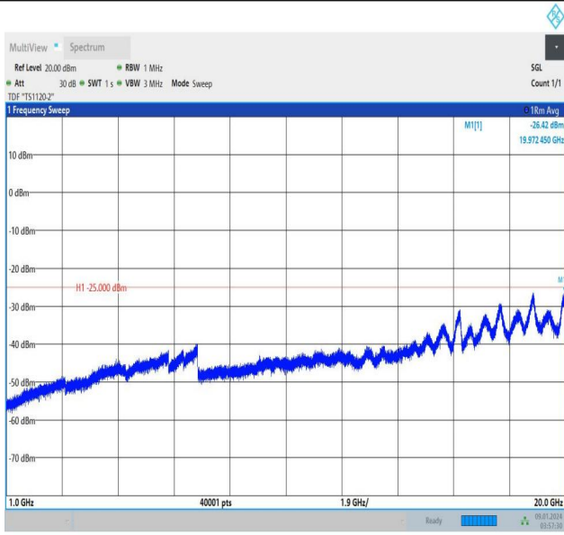
Band38_5MHz_16QAM_37775_1RB#0_1000~20000_1000~20000
