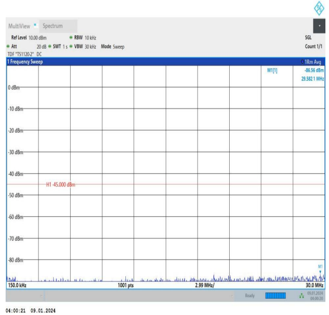
Band38_5MHz_QPSK_38000_1RB#0_0.15~30_0.15~30
