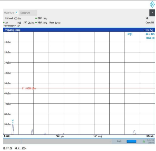
Band38_5MHz_16QAM_37775_1RB#0_0.009~0.15_0.009~0.15
