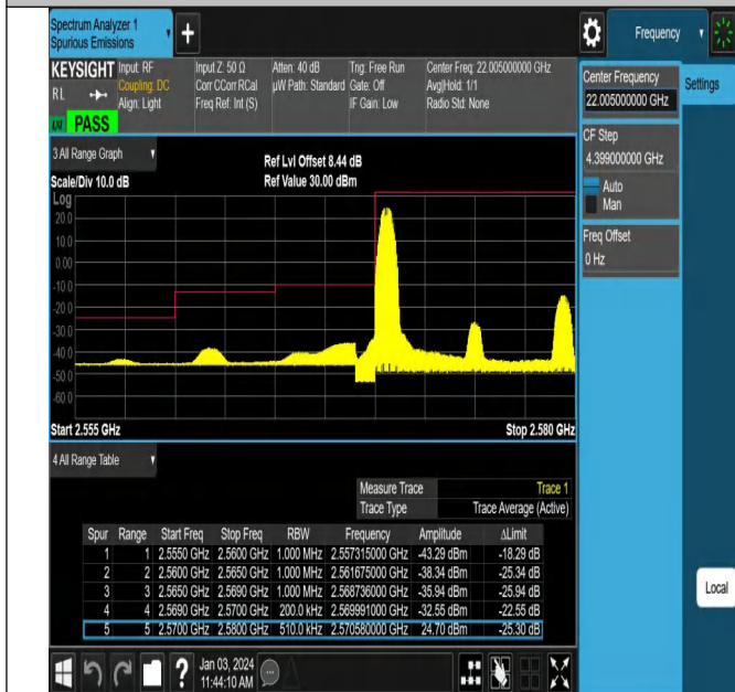
Band38_10MHz_16QAM_37800_1RB#0
