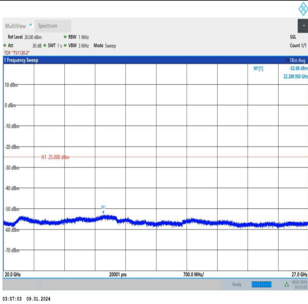
Band38_5MHz_QPSK_37775_1RB#0_20000~27000_20000~27000
