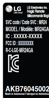
Label position
