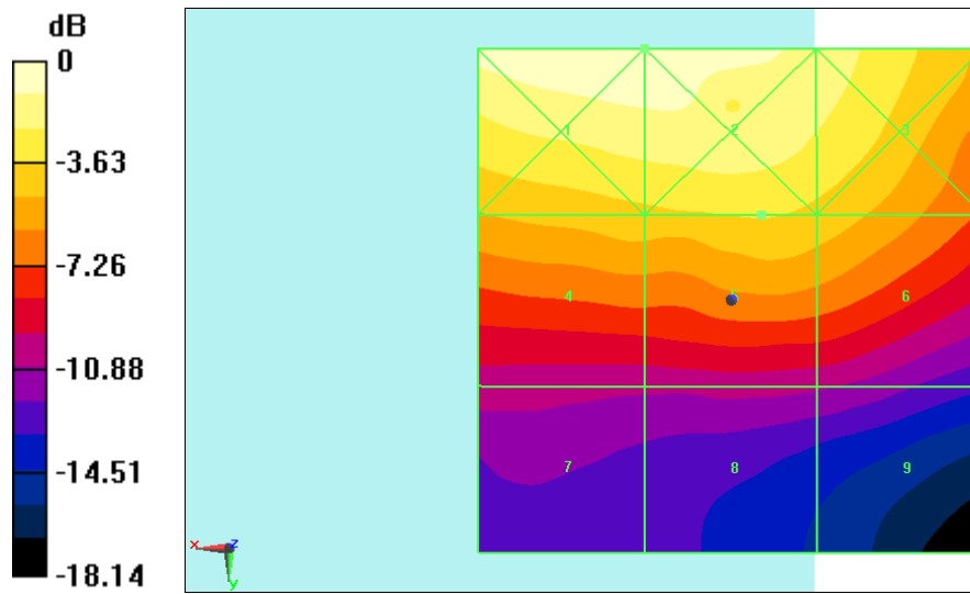
Fig B.4 HAC RF E-Field LTE Band41 PC3 64QAM
