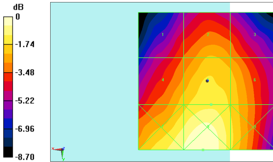
Fig B.4 HAC RF E-Field WIFI2.4G
