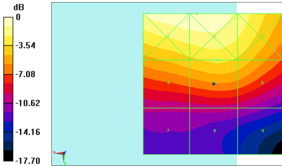
Fig B.3 HAC RF E-Field LTE Band41 PC2 QPSK
