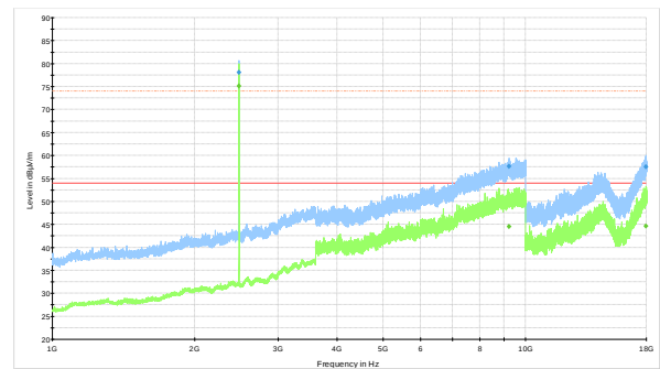
Figure 8.2-6: Radiated spurious emissions on high channel
