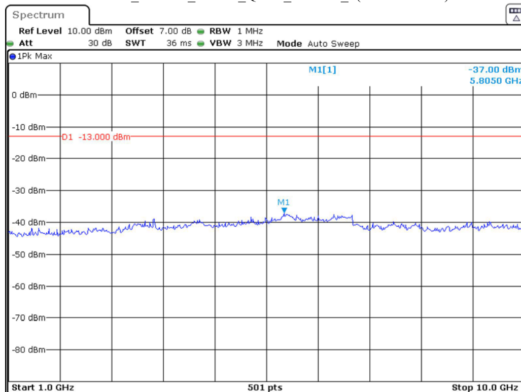
Band 12_10 MHz_Middle_QPSK_RB50#0_2(1GHz-10GHz)
