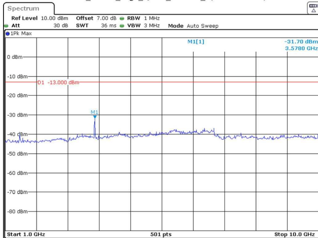
Band 12_3 MHz_High_QPSK_RB15#0_2(1GHz-10GHz)
