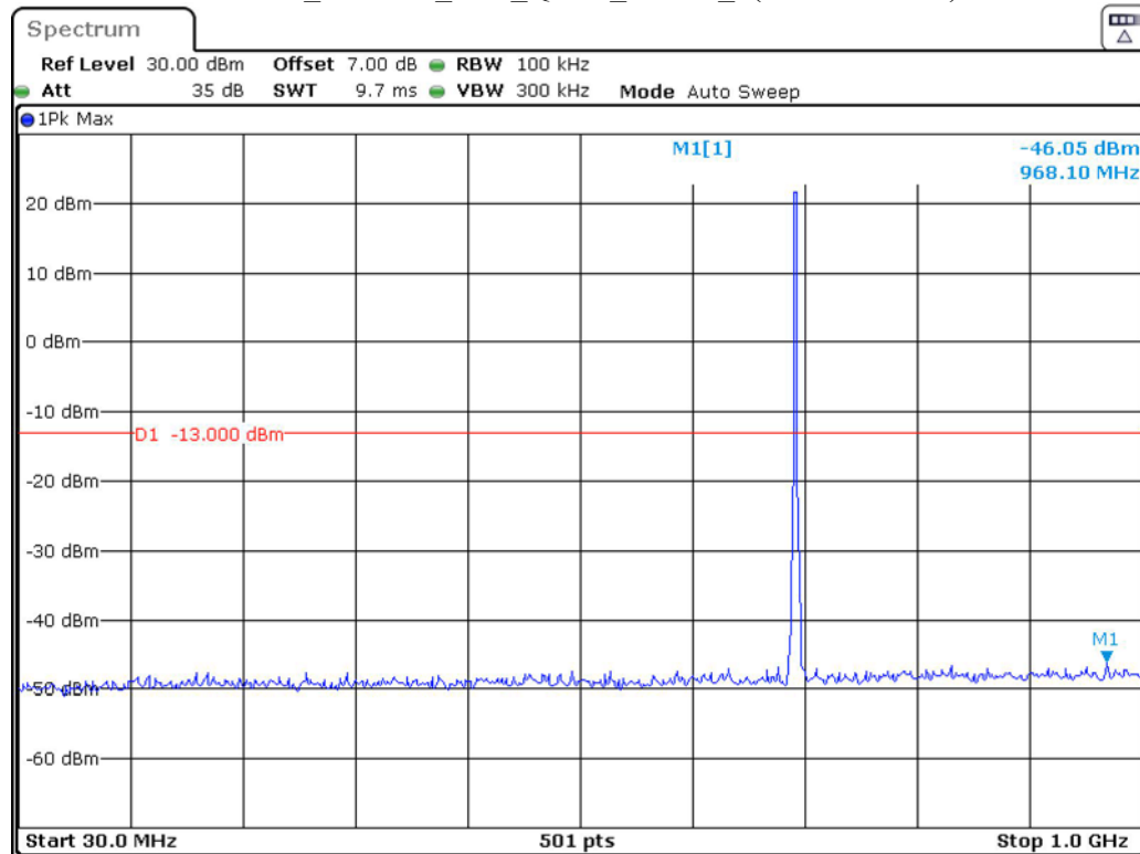
Band 12_1.4 MHz_Low_QPSK_RB6#0_1(30MHz-1GHz)
