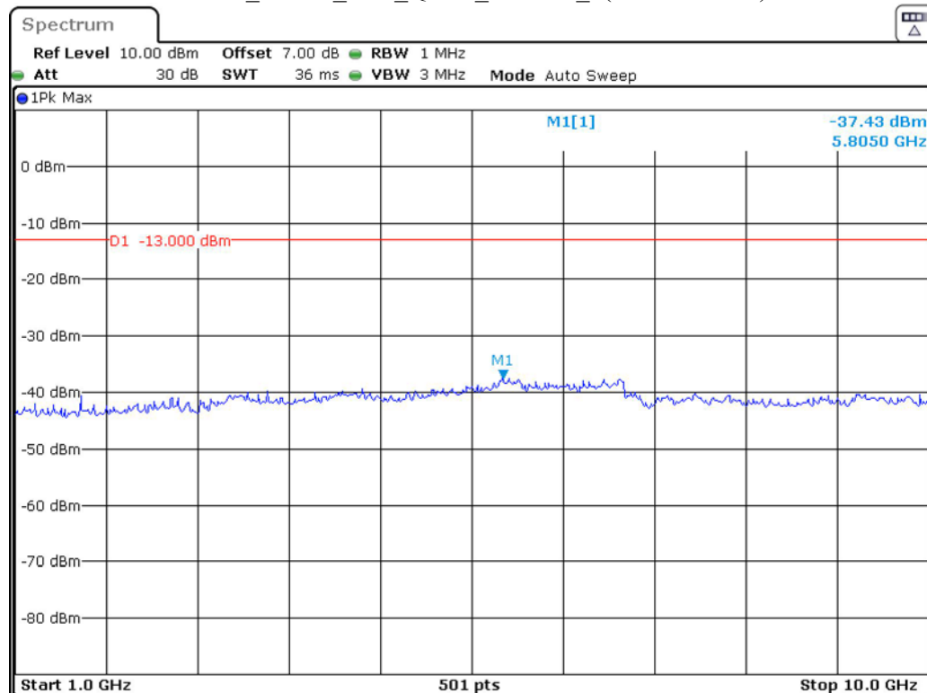
Band 5_5 MHz_Low_QPSK_RB25#0_2(1GHz-10GHz)
