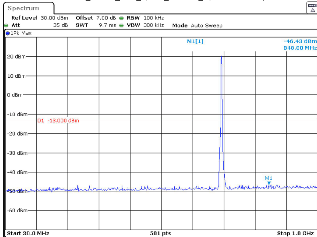
Band 12_3 MHz_Low_QPSK_RB15#0_1(30MHz-1GHz)
