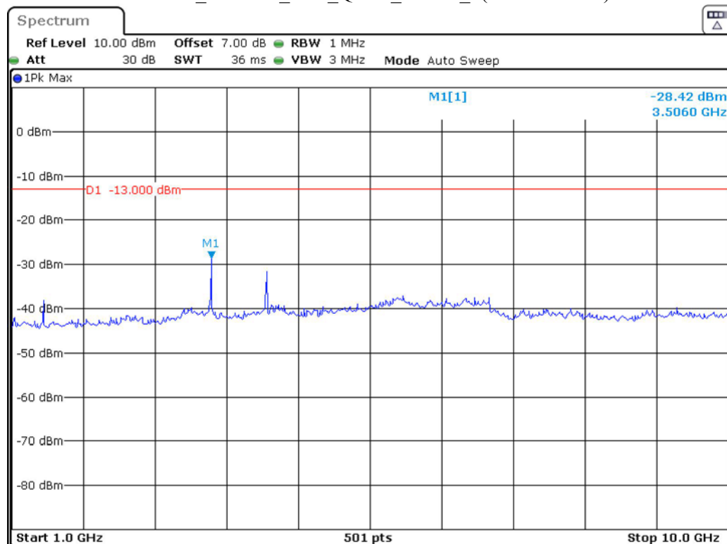
Band 12_1.4 MHz_Low_QPSK_RB6#0_2(1GHz-10GHz)
