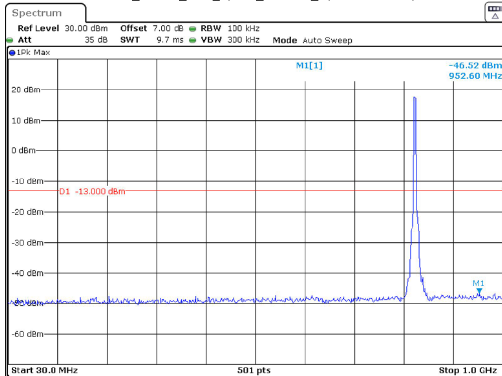
Band 5_5 MHz_Low_QPSK_RB25#0_1(30MHz-1GHz)
