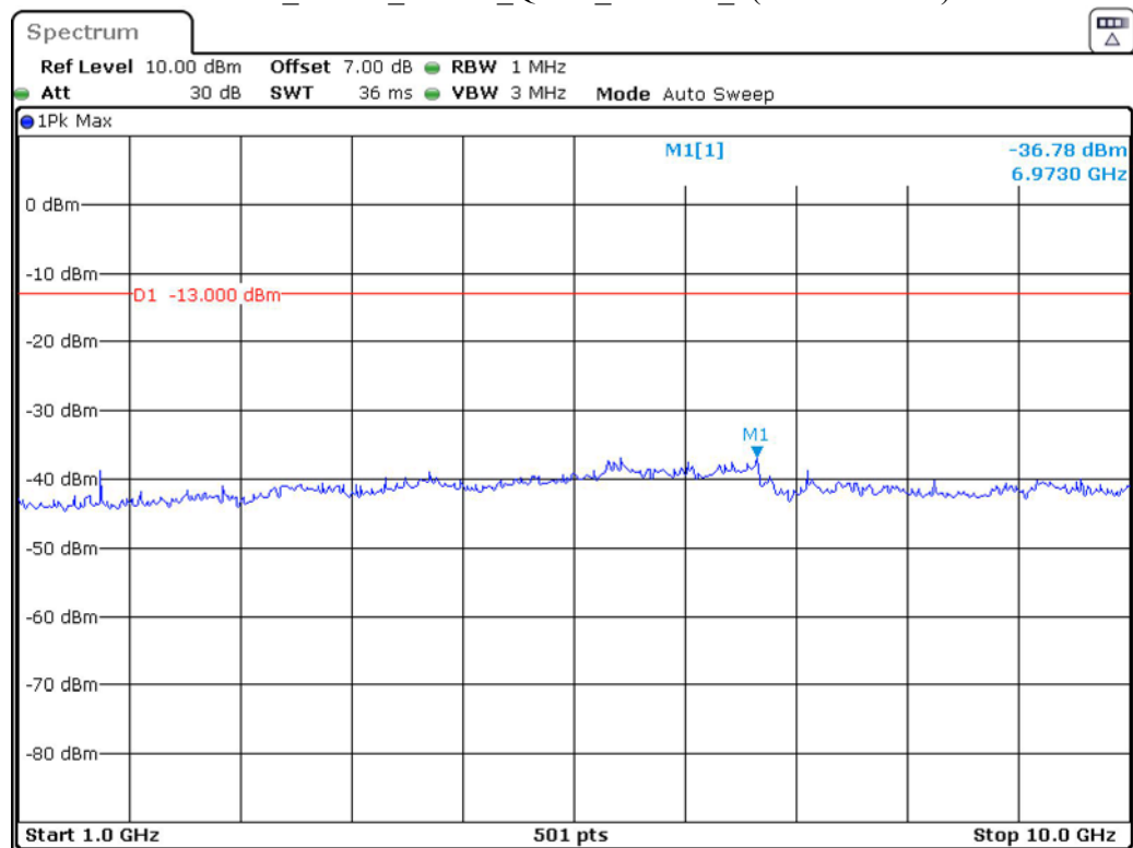
Band 5_3 MHz_Middle_QPSK_RB15#0_2(1GHz-10GHz)
