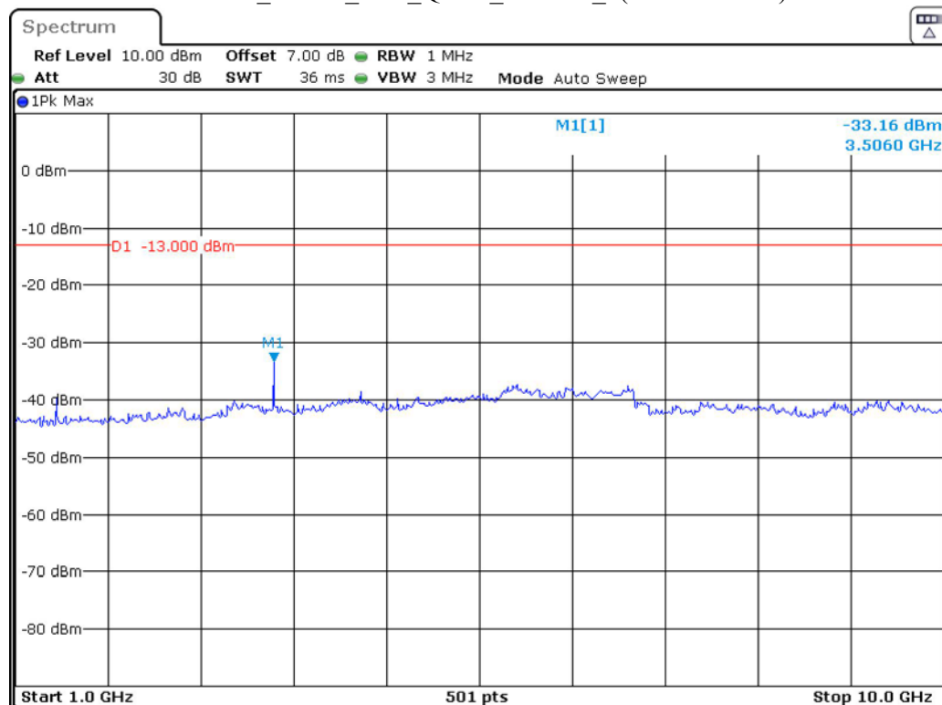
Band 12_3 MHz_Low_QPSK_RB15#0_2(1GHz-10GHz)
