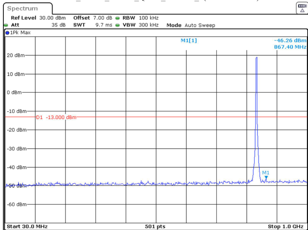
Band 5_3 MHz_Middle_QPSK_RB15#0_1(30MHz-1GHz)
