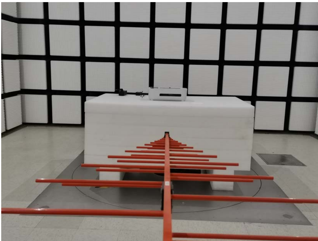
Radiated Emissions Above 1G front View
