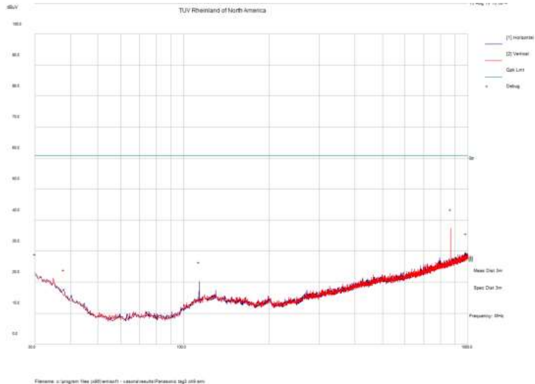
Figure 23: 30-1000 MHz, 434.568 MHz
