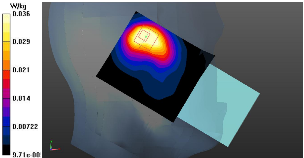
Fig.23 Bluetooth Head
