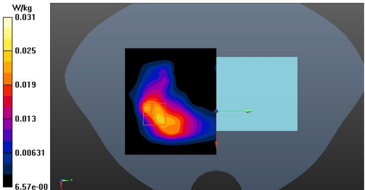
Fig.24 Bluetooth Body
