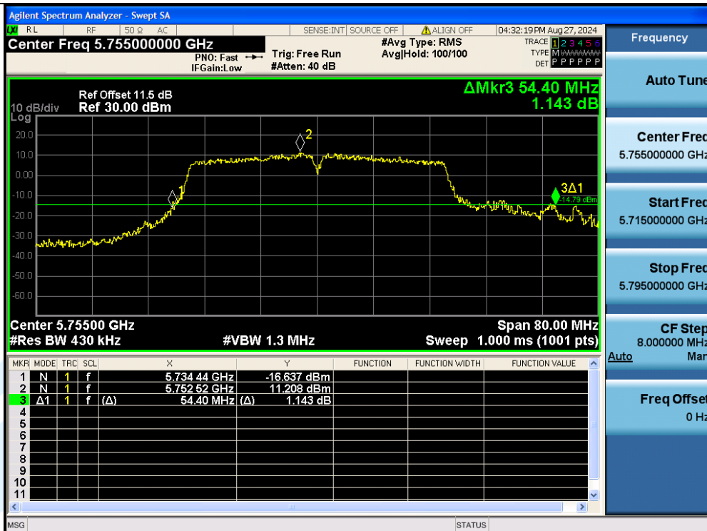
11AC40MIMO-Ant3-5755
