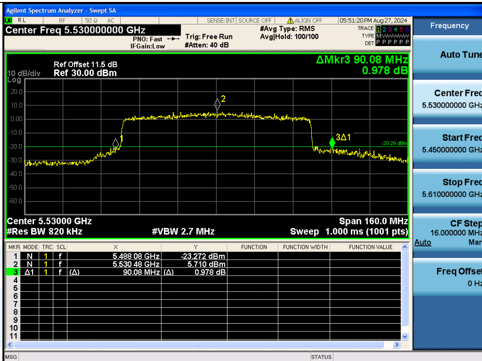
11AX80MIMO-Ant3-5530
