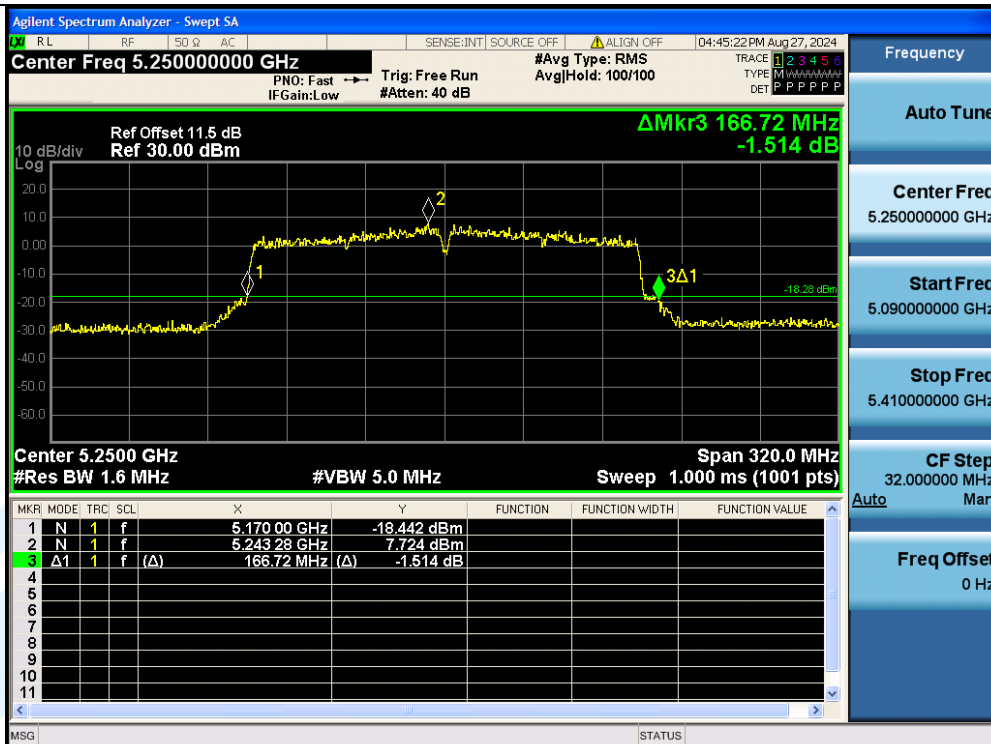
11AC160MIMO-Ant3-5250
