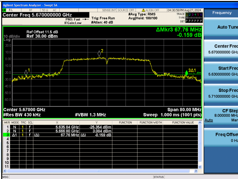
11AC40MIMO-Ant3-5670
