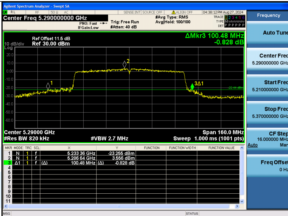
11AC80MIMO-Ant3-5290
