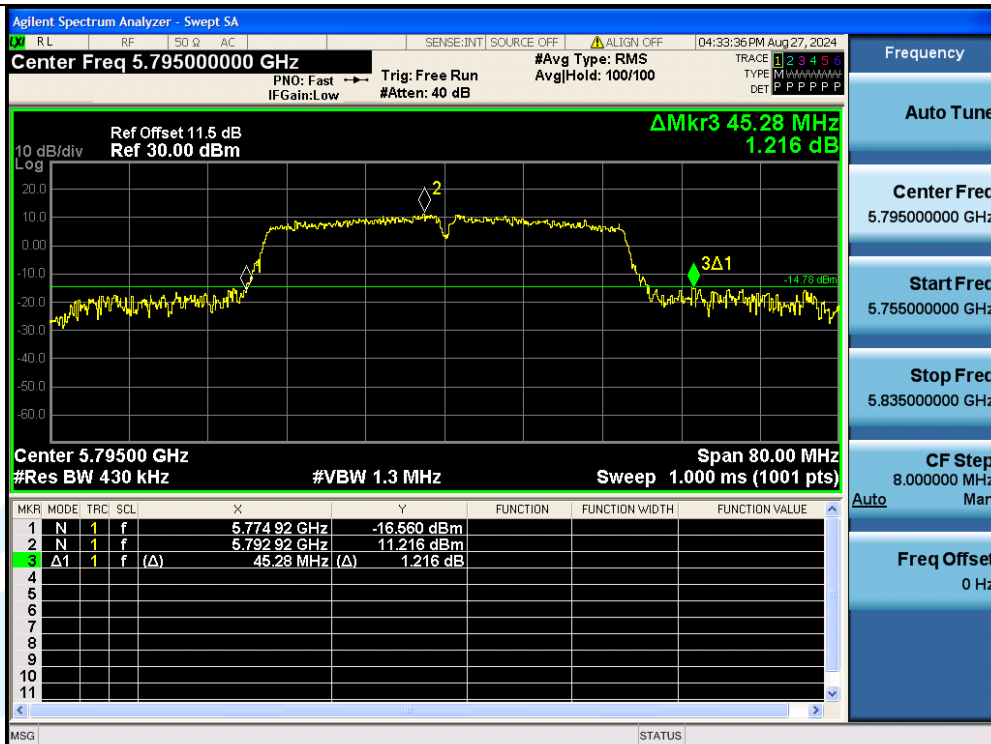
11AC40MIMO-Ant3-5795
