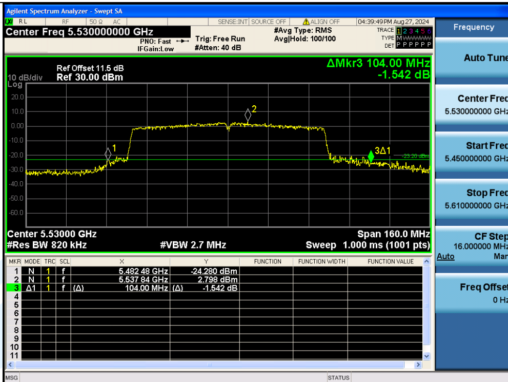
11AC80MIMO-Ant3-5530
