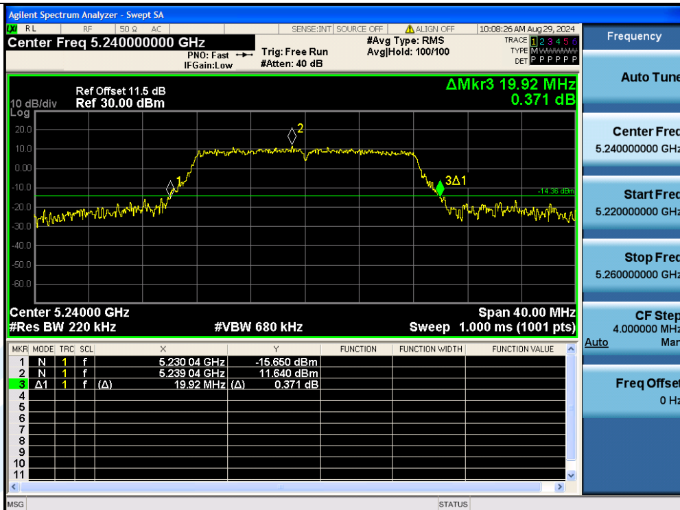
11A-Ant3-5240
