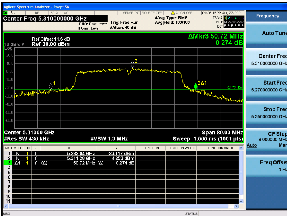
11AC40MIMO-Ant3-5310
