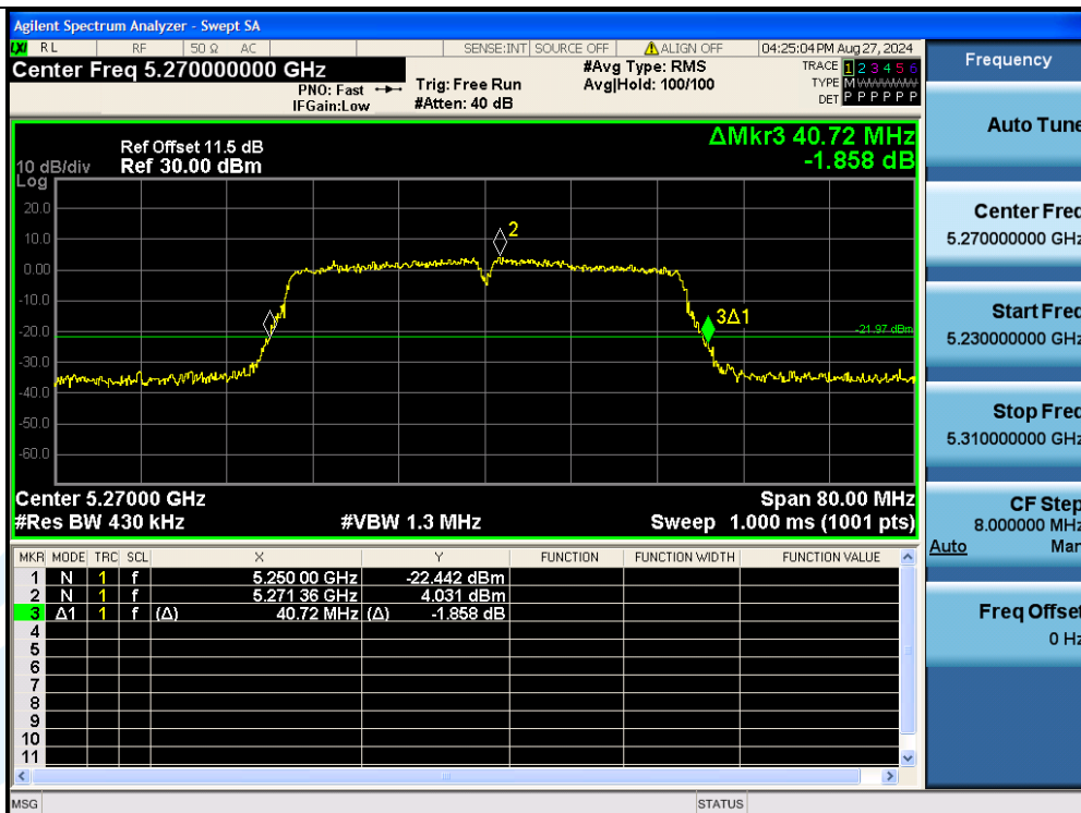
11AC40MIMO-Ant3-5270
