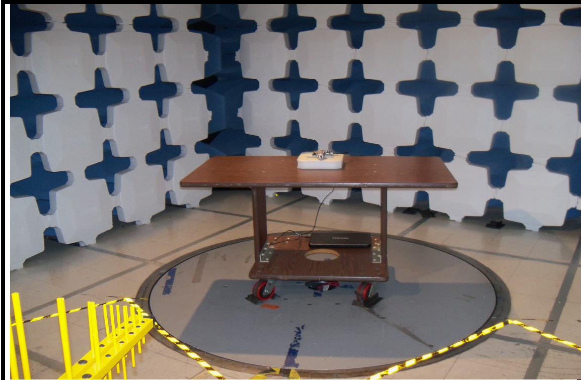
Test Setup Photo 1 – Radiated Emissions
