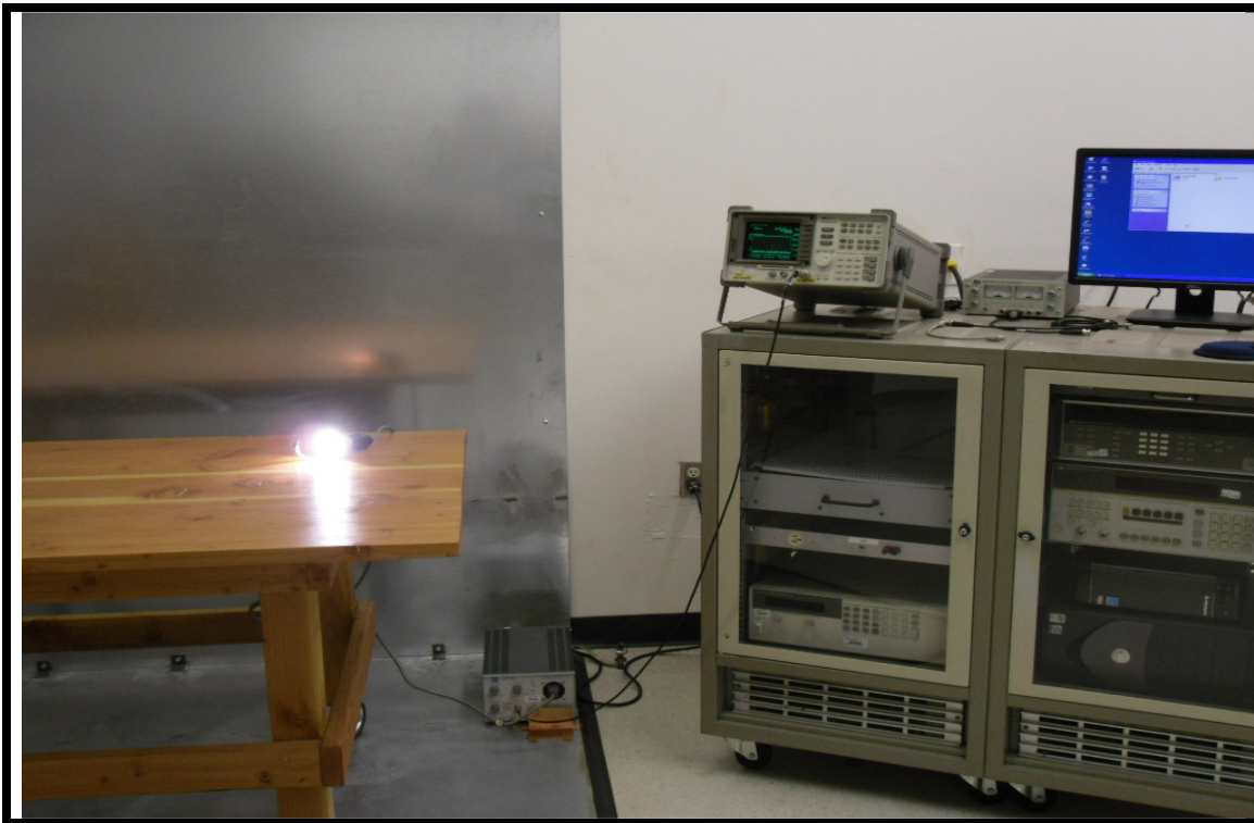
Test Setup Photo 4 – Conducted Emissions
