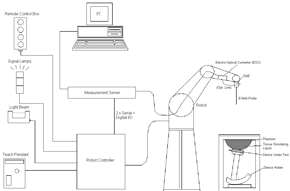
Fig-3.1 SPEAG DASY52 System Setup
