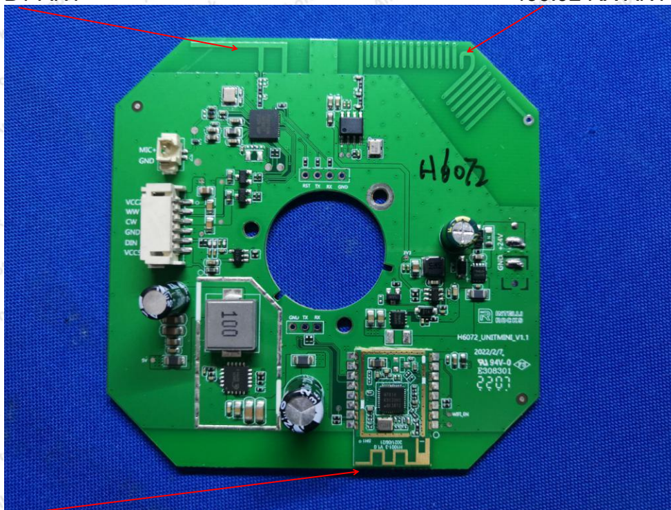
Wifi ANT
