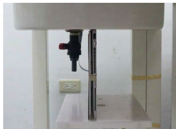
Fig.5 EUT Bottom side to flat phantom
