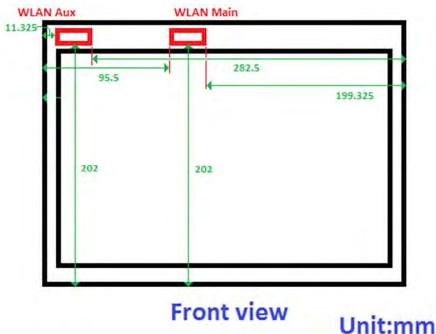
Fig.10 Antenna location of EUT (tablet mode)
