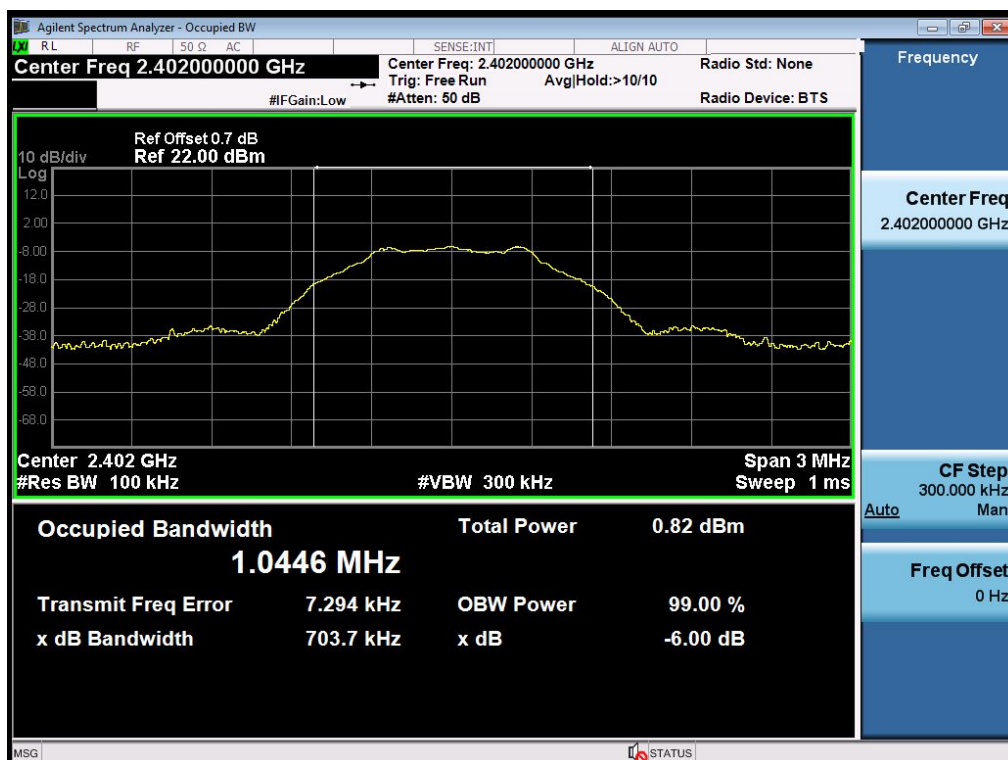
(Plot 4.7.1 A: Channel 00: 2402MHz @ GFSK)
