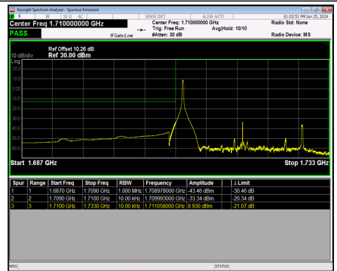
Band66-20MHz-16QAM-132072-100RB#0
