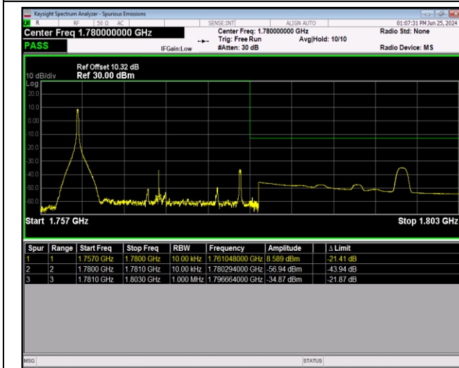
Band66-20MHz-16QAM-132572-100RB#0
