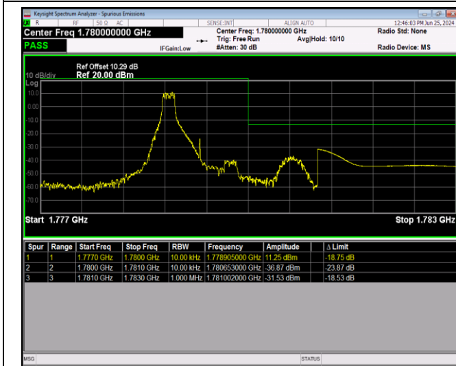
Band66-1.4MHz-64QAM-132665-6RB#0
