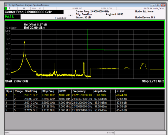
Band41-20MHz-64QAM-41490-100RB#0
