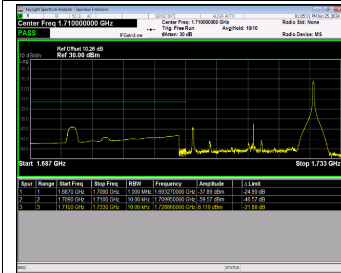
Band66-20MHz-64QAM-132572-1RB#0
