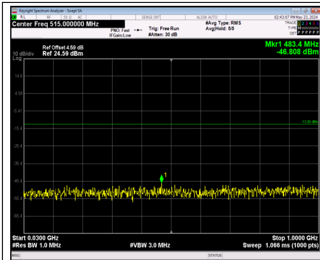
Band2-1.4MHz-16QAM-18607-1RB#0-Range1:30~1000MHz
