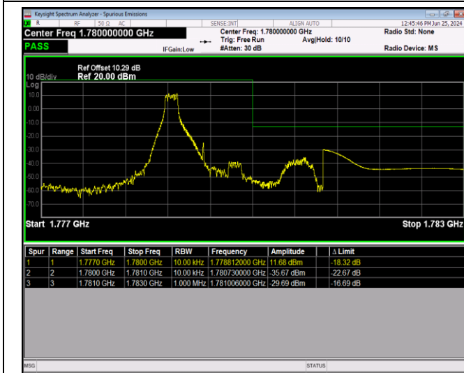
Band66-1.4MHz-16QAM-132665-6RB#0
