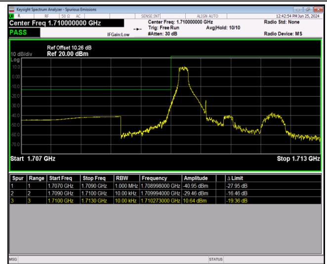
Band66-1.4MHz-64QAM-131979-6RB#0
