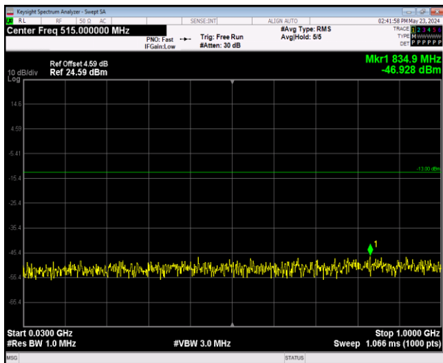
Band2-1.4MHz-64QAM-18900-1RB#0-Range1:30~10 00MHz
