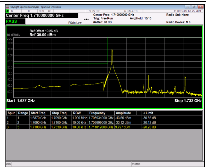
Band66-20MHz-QPSK-132072-100RB#0
