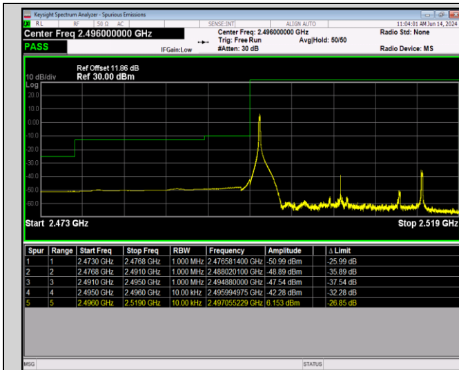
Band41-20MHz-64QAM-39750-100RB#0
