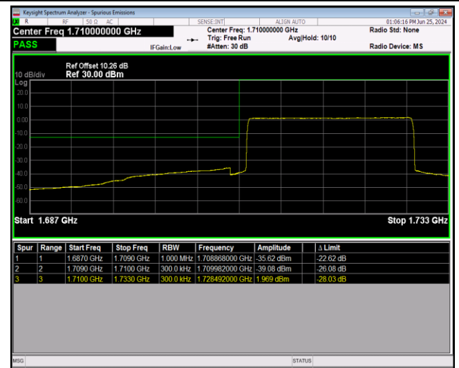
Band66-20MHz-16QAM-132572-1RB#99
