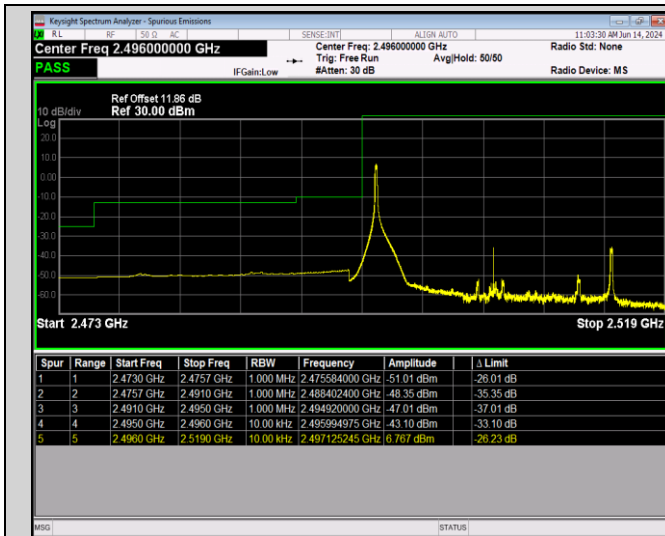
Band41-20MHz-16QAM-39750-100RB#0
