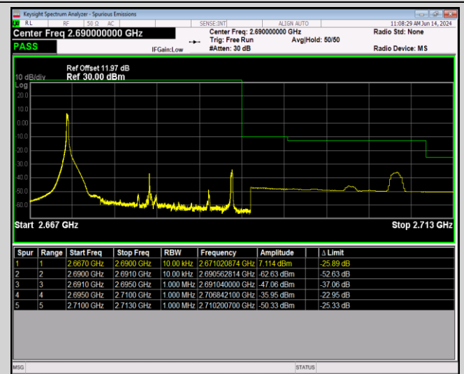
Band41-20MHz-16QAM-41490-100RB#0
