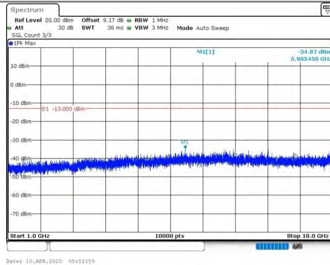
Band12-5MHz-16QAM-23155-1RB#0-Range2:1000~10000MHz
