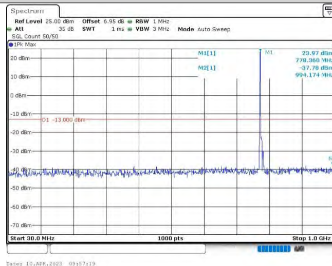
Band13-5MHz-16QAM-23205-1RB#0-Range1:30~1000MHz
