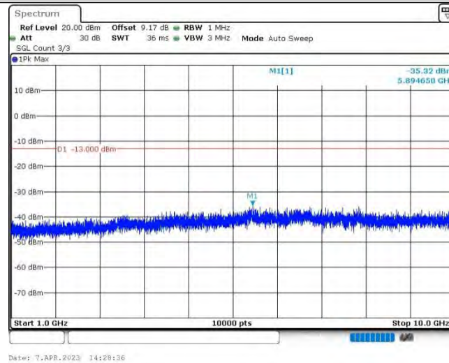
Band12-1.4MHz-16QAM-23173-1RB#0-Range2:1000~10000MHz
