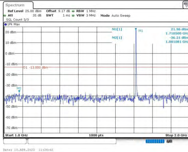
Band4-5MHz-16QAM-19975-1RB#0-Range2:1000~2000MHz
