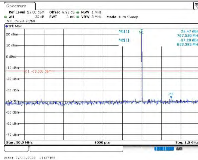
Band12-1.4MHz-16QAM-23095-1RB#0-Range1:30~1000MHz
