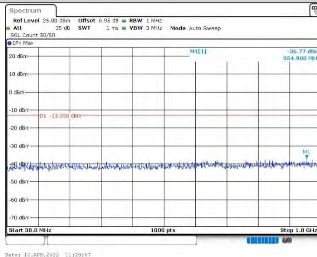
Band4-5MHz-16QAM-20375-1RB#0-Range1:30~1000MHz
