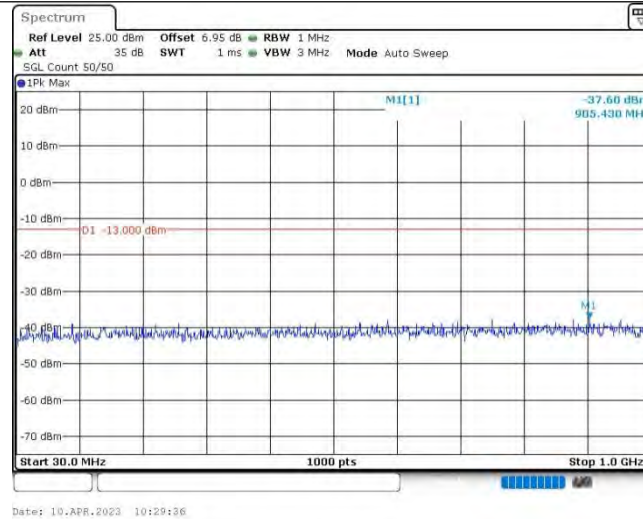
Band25-1.4MHz-16QAM-26365-1RB#0-Range1:30~1000MHz
