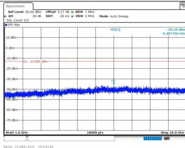
Band12-10MHz-QPSK-23095-1RB#0-Range2:1000~10000MHz
