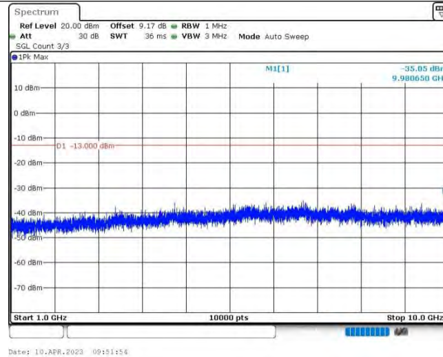
Band12-5MHz-16QAM-23035-1RB#0-Range2:1000~10000MHz
