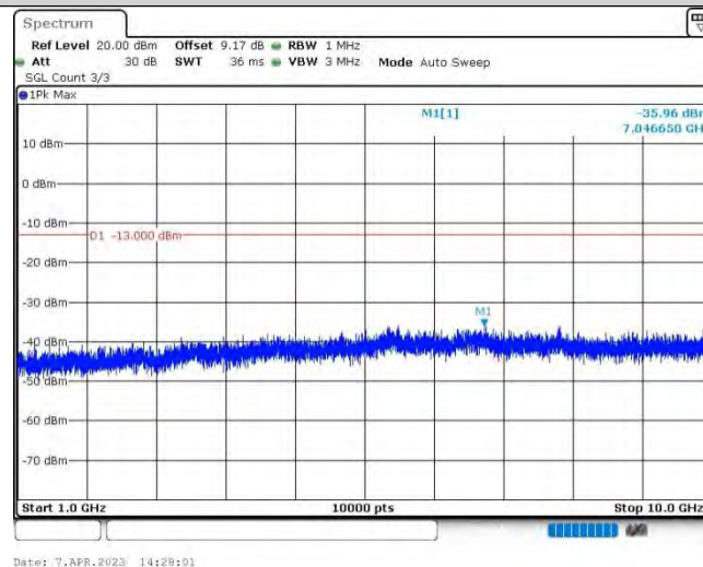
Band12-1.4MHz-16QAM-23095-1RB#0-Range2:1000~10000MHz
