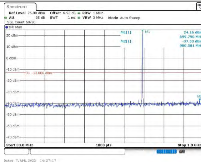
Band12-1.4MHz-16QAM-23017-1RB#0-Range1:30~1000MHz
