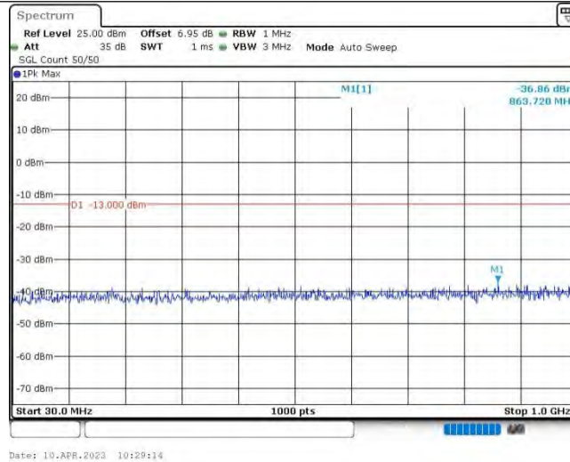
Band25-1.4MHz-QPSK-26365-1RB#0-Range1:30~1000MHz
