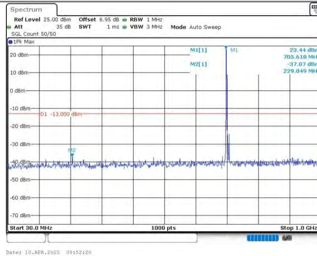
Band12-5MHz-16QAM-23095-1RB#0-Range1:30~1000MHz
