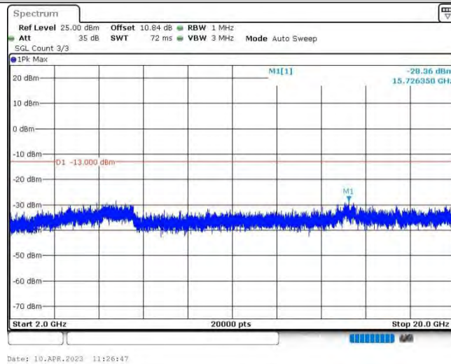
Band4-5MHz-16QAM-19975-1RB#0-Range3:2000~20000MHz
