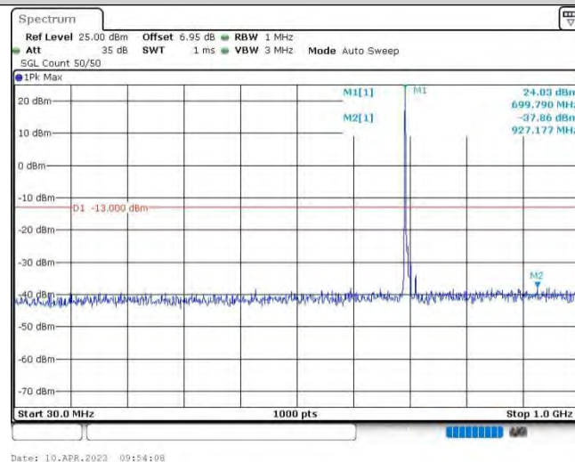
Band12-10MHz-QPSK-23060-1RB#0-Range1:30~1000MHz
