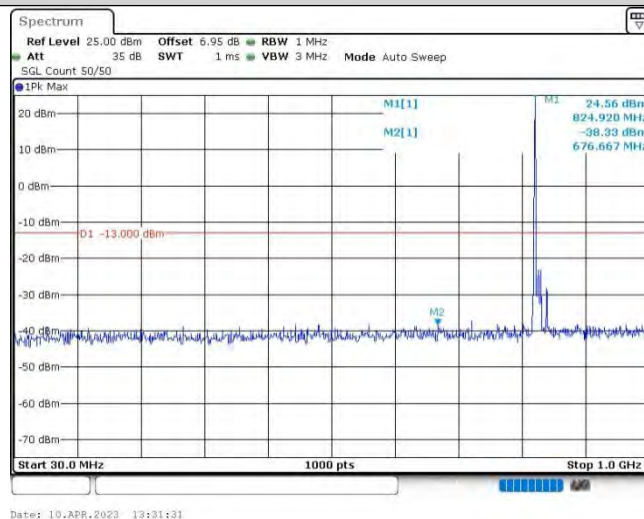
Band5-10MHz-QPSK-20450-1RB#0-Range1:30~1000MHz
