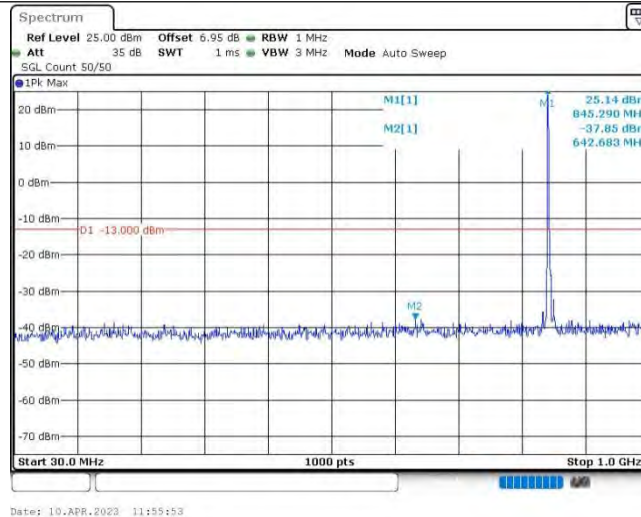
Band5-5MHz-QPSK-20625-1RB#0-Range1:30~1000MHz
