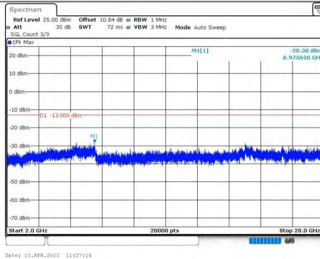
Band4-5MHz-QPSK-20175-1RB#0-Range3:2000~20000MHz
