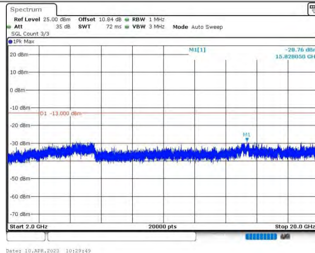
Band25-1.4MHz-16QAM-26365-1RB#0-Range3:2000~20000MHz
