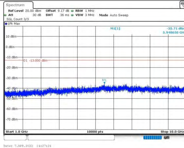
Band12-1.4MHz-16QAM-23017-1RB#0-Range2:1000~10000MHz
