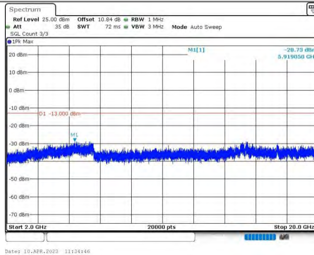
Band4-10MHz-QPSK-20175-1RB#0-Range3:2000~20000MHz
