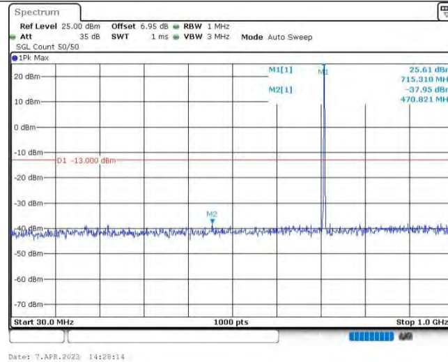
Band12-1.4MHz-QPSK-23173-1RB#0-Range1:30~1000MHz
