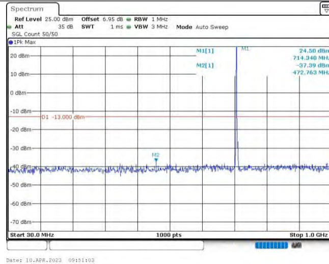
Band12-3MHz-16QAM-23165-1RB#0-Range1:30~1000MHz
