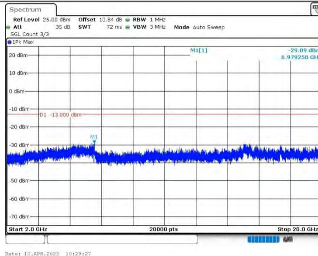
Band25-1.4MHz-QPSK-26365-1RB#0-Range3:2000~20000MHz
