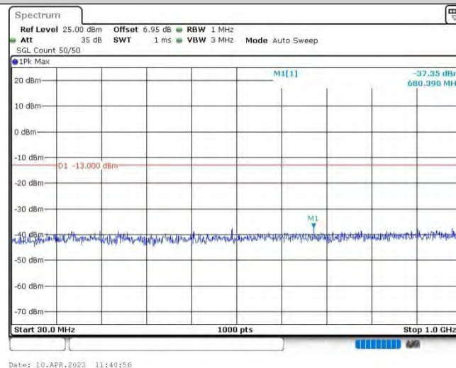
Band4-15MHz-QPSK-20175-1RB#0-Range1:30~1000MHz
