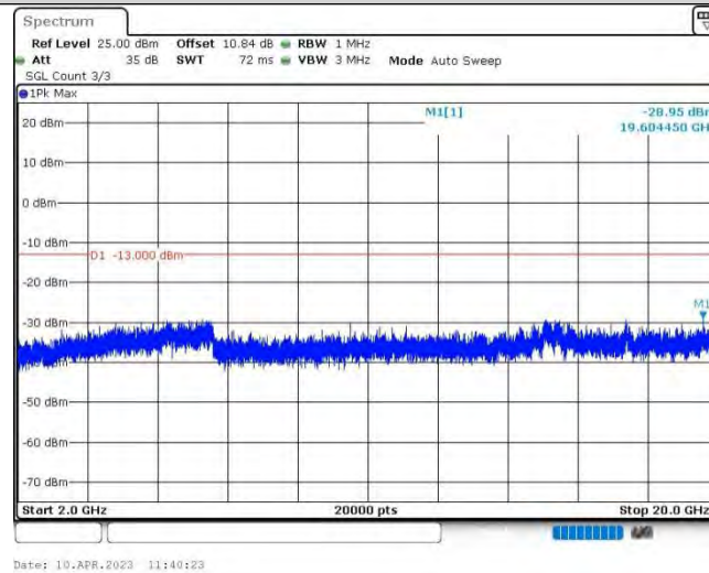
Band4-15MHz-QPSK-20025-1RB#0-Range3:2000~20000MHz
