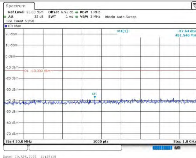
Band4-10MHz-QPSK-20350-1RB#0-Range1:30~1000MHz
