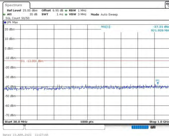
Band4-5MHz-QPSK-20375-1RB#0-Range1:30~1000MHz
