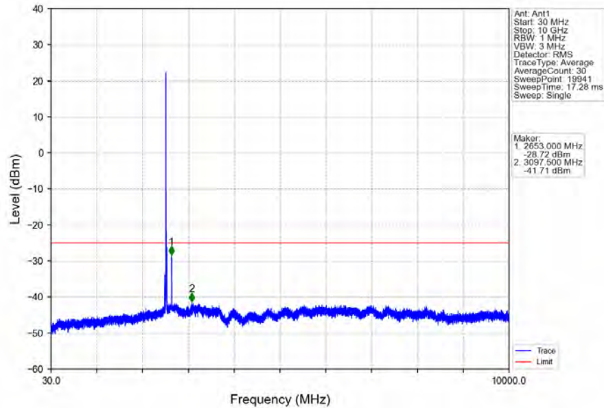
Band7_15MHz_16QAM_MCH_2535MHz_RB_1_0_NTNV
