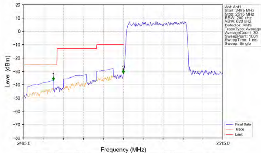
Band7_10MHz_16QAM_LCH_2505MHz_RB_50_0_NTNV
