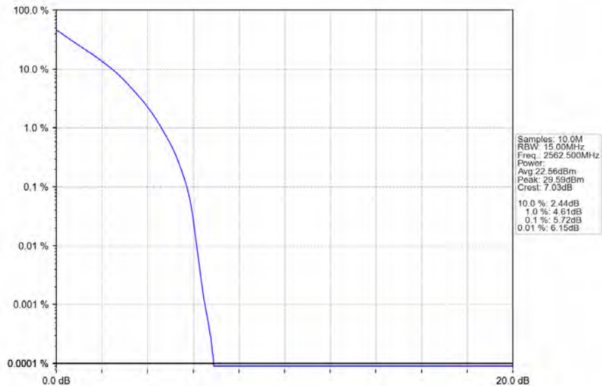
Band7_15MHz_QPSK_HCH_2562.5MHz_RB_75_0_NTNV
