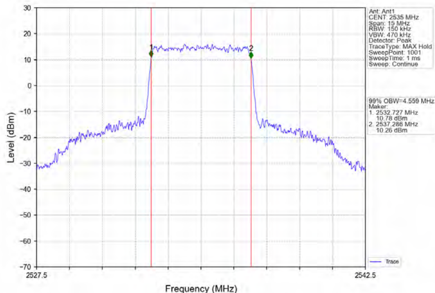
Band7_5MHz_64QAM_MCH_2535MHz_RB_25_0_NTNV
