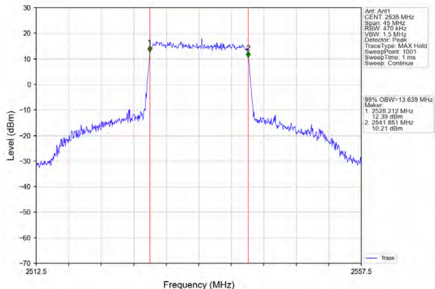
Band7_15MHz_64QAM_MCH_2535MHz_RB_75_0_NTNV
