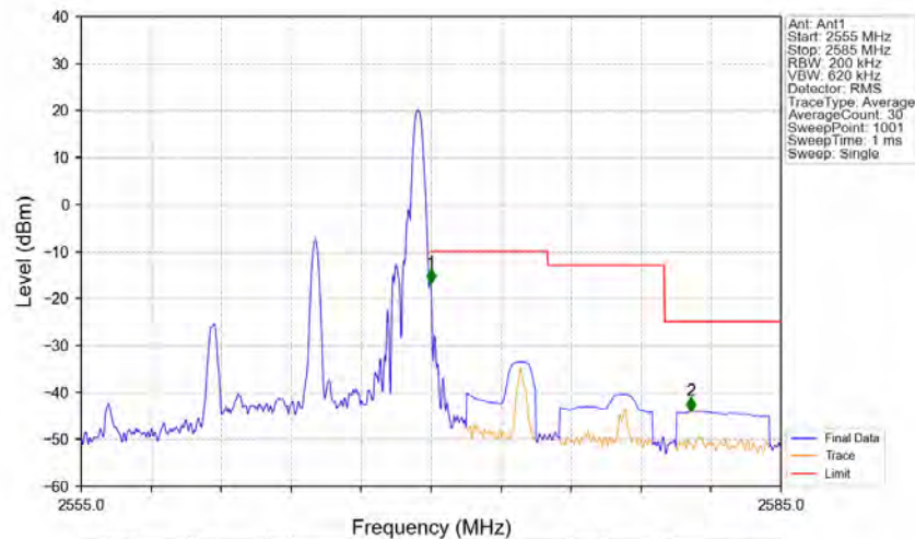
Band7_10MHz_64QAM_HCH_2565MHz_RB_1_49_NTNV
