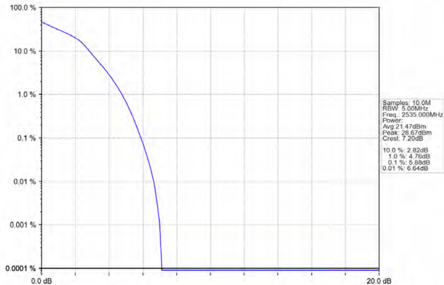
Band7_5MHz_16QAM_MCH_2535MHz_RB_25_0_NTNV
