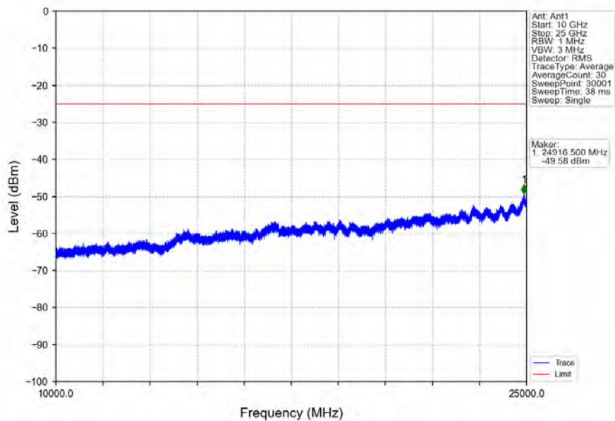
Band7_5MHz_16QAM_MCH_2535MHz_RB_1_0_NTNV
