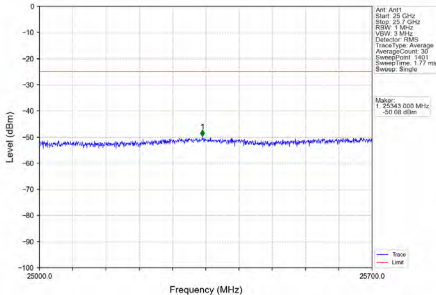
Band7_5MHz_16QAM_LCH_2502.5MHz_RB_25_0_NTNV
