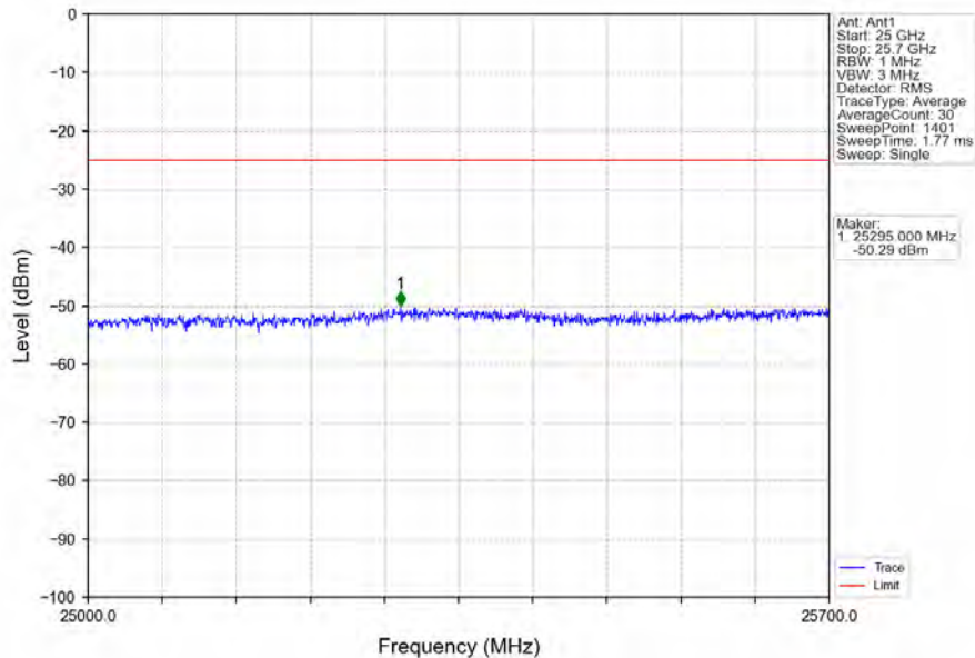
Band7_15MHz_16QAM_LCH_2507.5MHz_RB_75_0_NTNV
