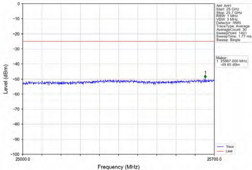
Band7_15MHz_64QAM_HCH_2562.5MHz_RB_1_74_NTNV
