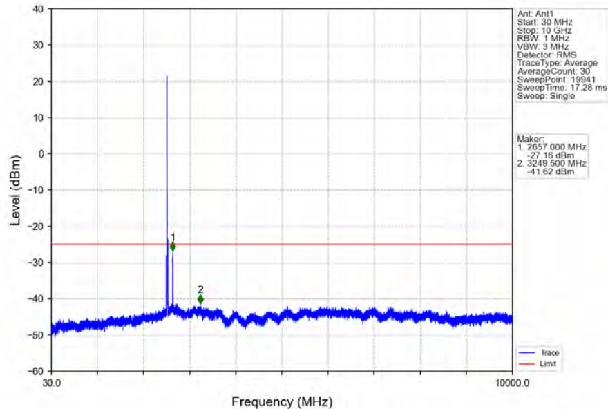
Band7_10MHz_16QAM_MCH_2535MHz_RB_1_0_NTNV
