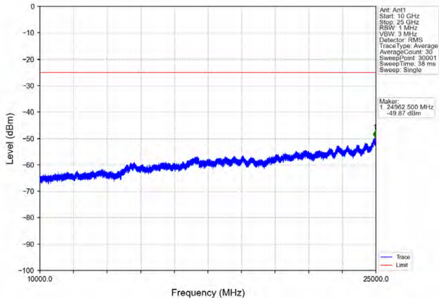
Band7_10MHz_16QAM_HCH_2565MHz_RB_1_0_NTNV
