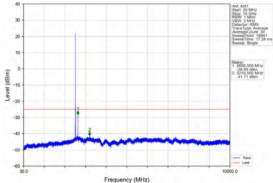
Band7_5MHz_16QAM_MCH_2535MHz_RB_1_0_NTNV
