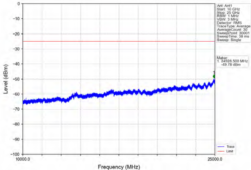
Band7_5MHz_16QAM_HCH_2567.5MHz_RB_1_0_NTNV
