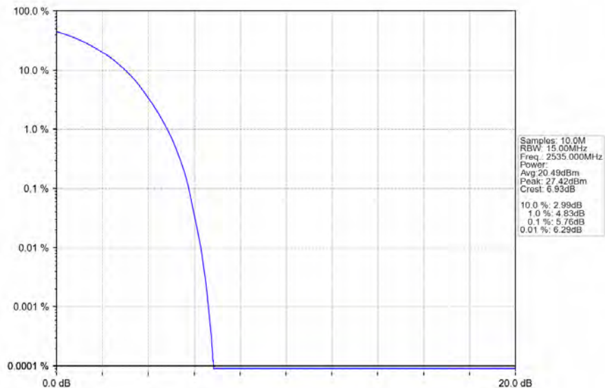
Band7_15MHz_64QAM_MCH_2535MHz_RB_75_0_NTNV
