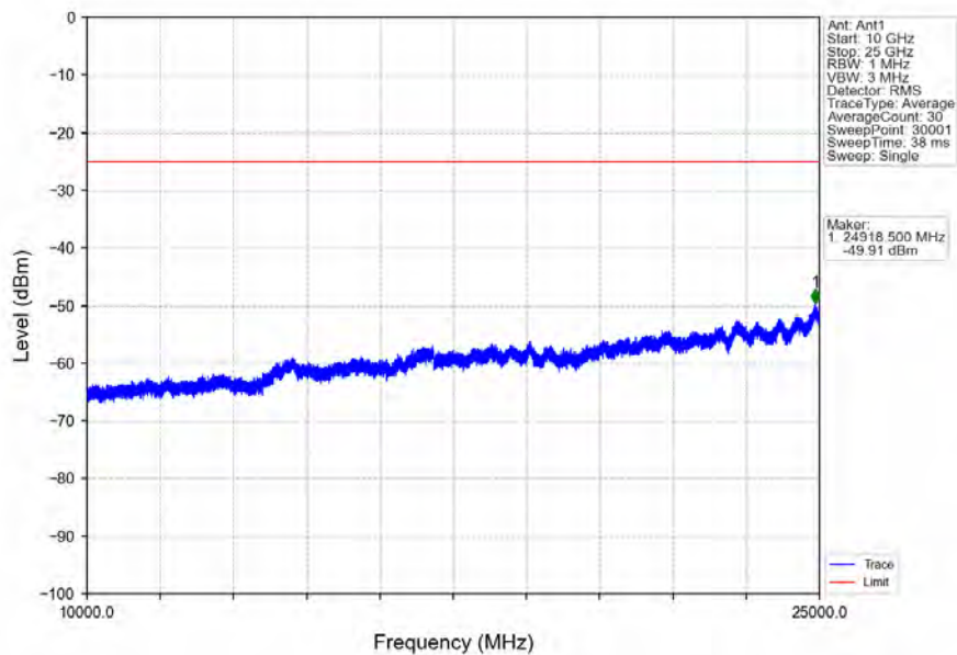
Band7_10MHz_64QAM_HCH_2565MHz_RB_1_0_NTNV
