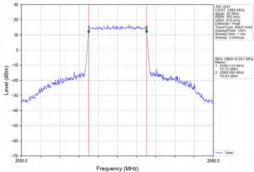
Band7_10MHz_64QAM_HCH_2565MHz_RB_50_0_NTNV
