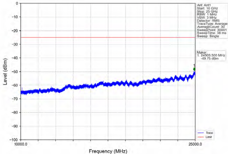
Band7_15MHz_QPSK_MCH_2535MHz_RB_1_0_NTNV
