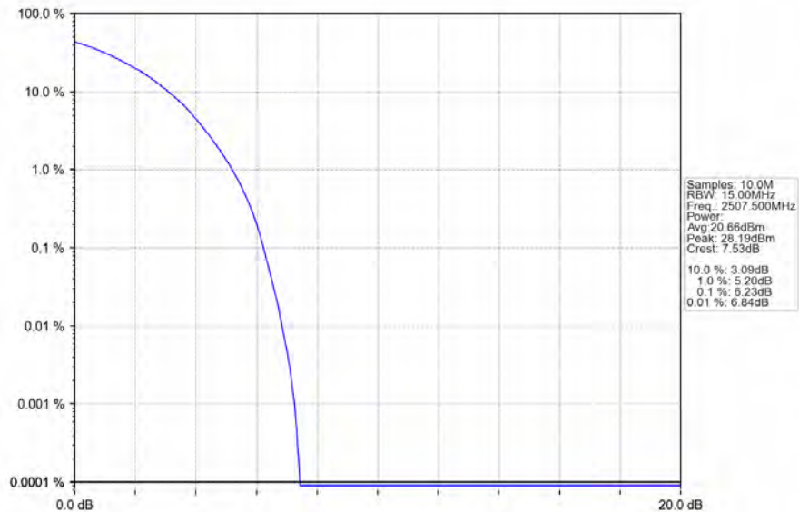
Band7_15MHz_64QAM_LCH_2507.5MHz_RB_75_0_NTNV
