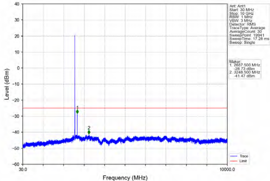
Band7_5MHz_64QAM_HCH_2567.5MHz_RB_1_0_NTNV
