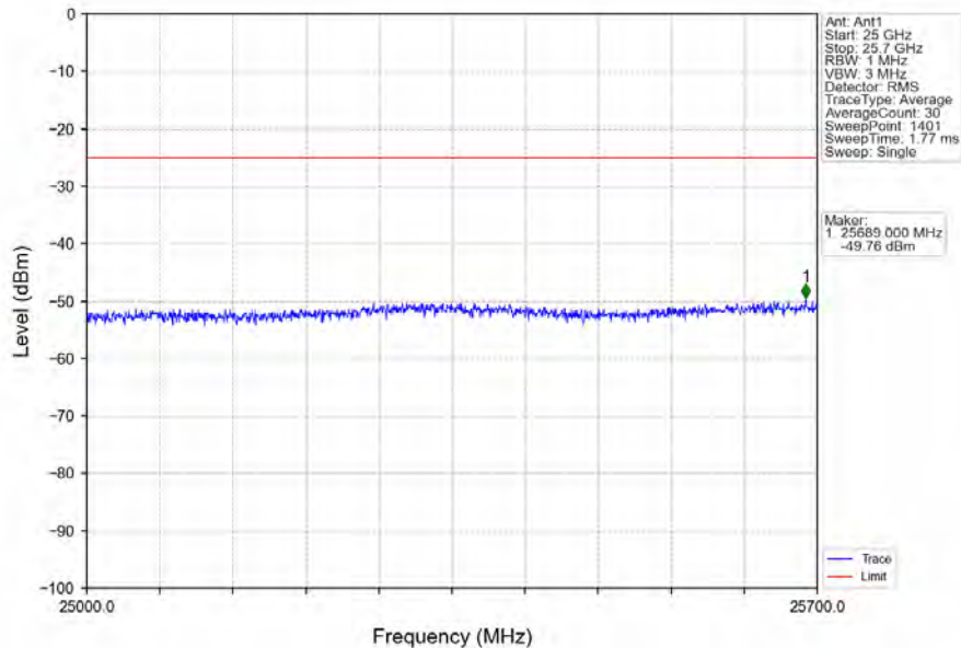
Band7_5MHz_64QAM_HCH_2567.5MHz_RB_1_24_NTNV
