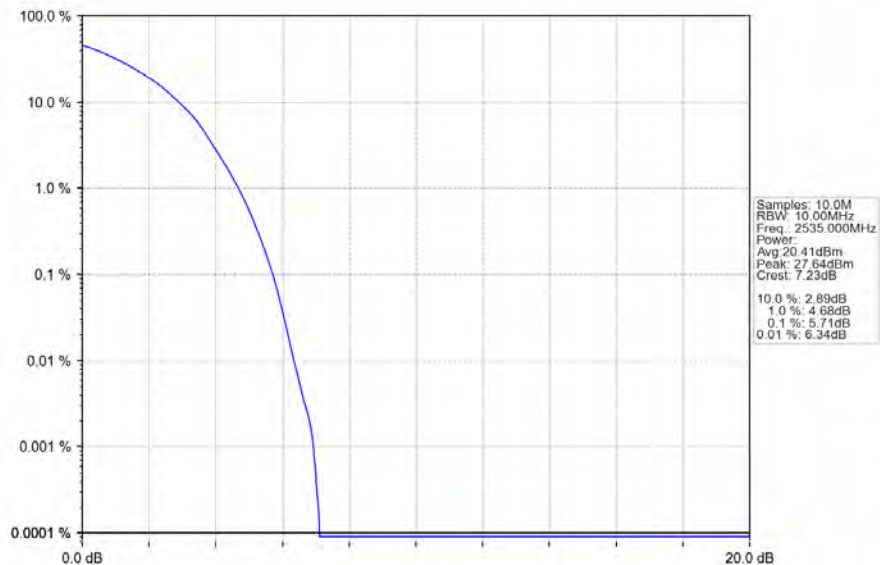
Band7_10MHz_64QAM_MCH_2535MHz_RB_50_0_NTNV
