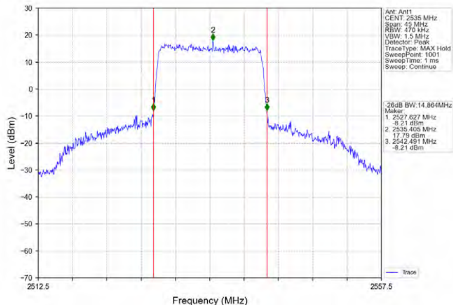
Band7_15MHz_64QAM_MCH_2535MHz_RB_75_0_NTNV
