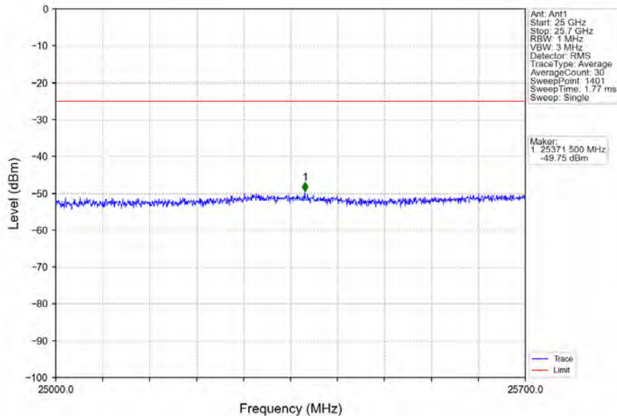
Band7_10MHz_64QAM_HCH_2565MHz_RB_1_49_NTNV
