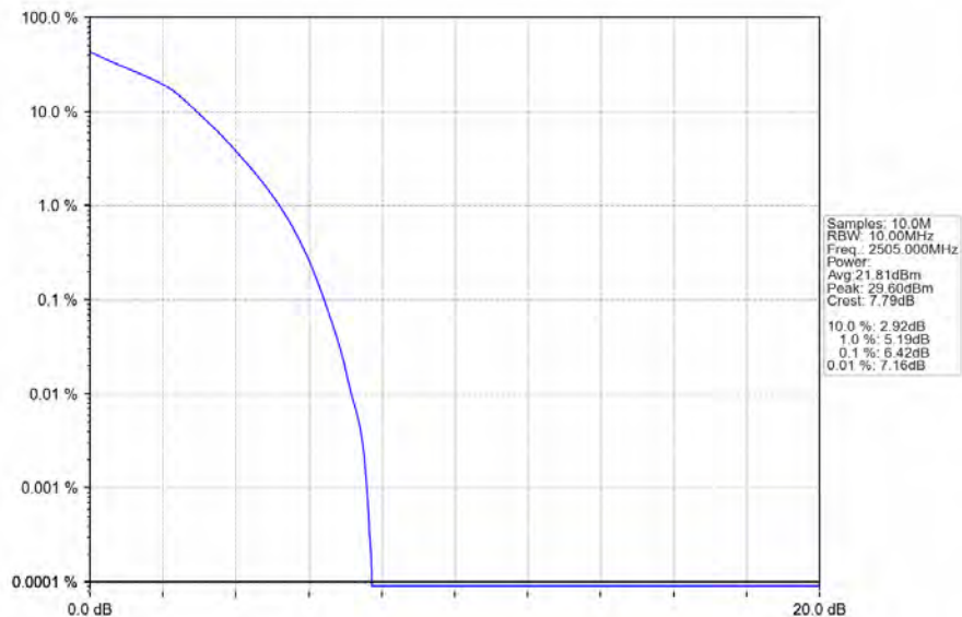
Band7_10MHz_16QAM_LCH_2505MHz_RB_50_0_NTNV
