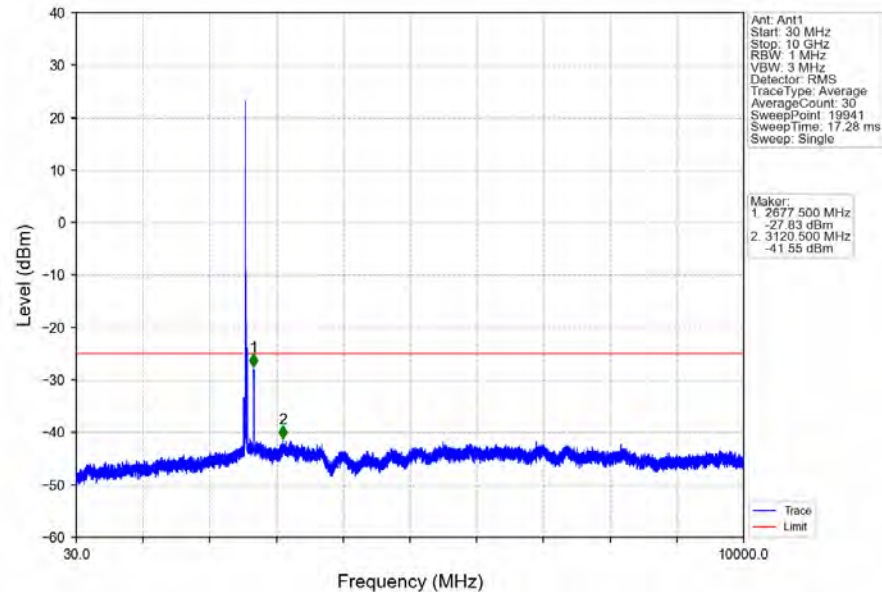
Band7_15MHz_QPSK_HCH_2562.5MHz_RB_1_0_NTNV
