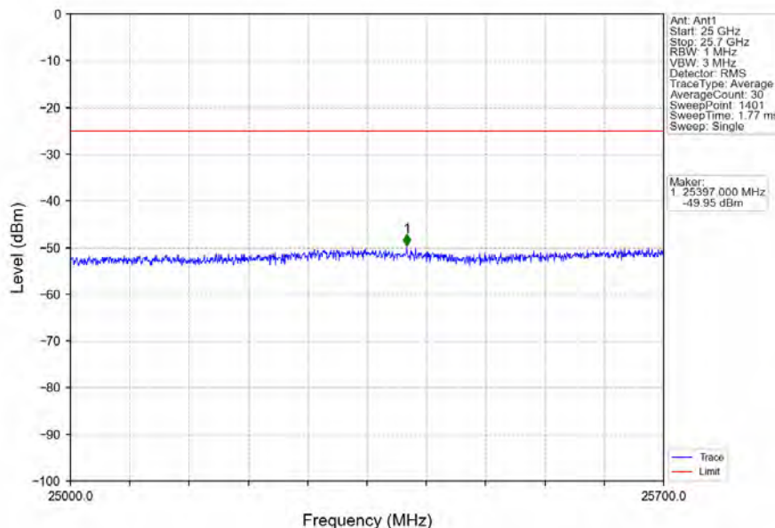
Band7_15MHz_64QAM_MCH_2535MHz_RB_1_0_NTNV
