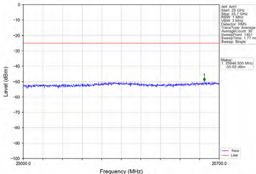
Band7_10MHz_64QAM_LCH_2505MHz_RB_1_0_NTNV
