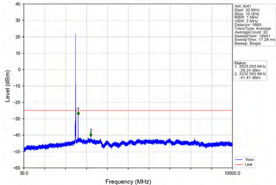
Band7_10MHz_16QAM_LCH_2505MHz_RB_1_0_NTNV
