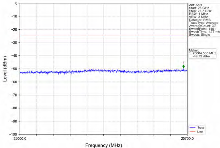
Band7_10MHz_16QAM_HCH_2565MHz_RB_1_0_NTNV
