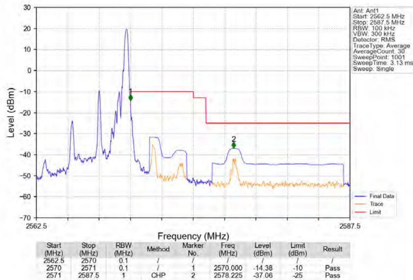
Band7_5MHz_16QAM_HCH_2567.5MHz_RB_1_24_NTNV
