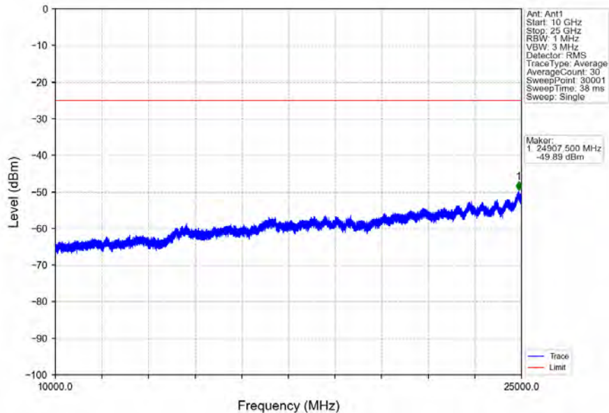
Band7_15MHz_QPSK_LCH_2507.5MHz_RB_1_0_NTNV
