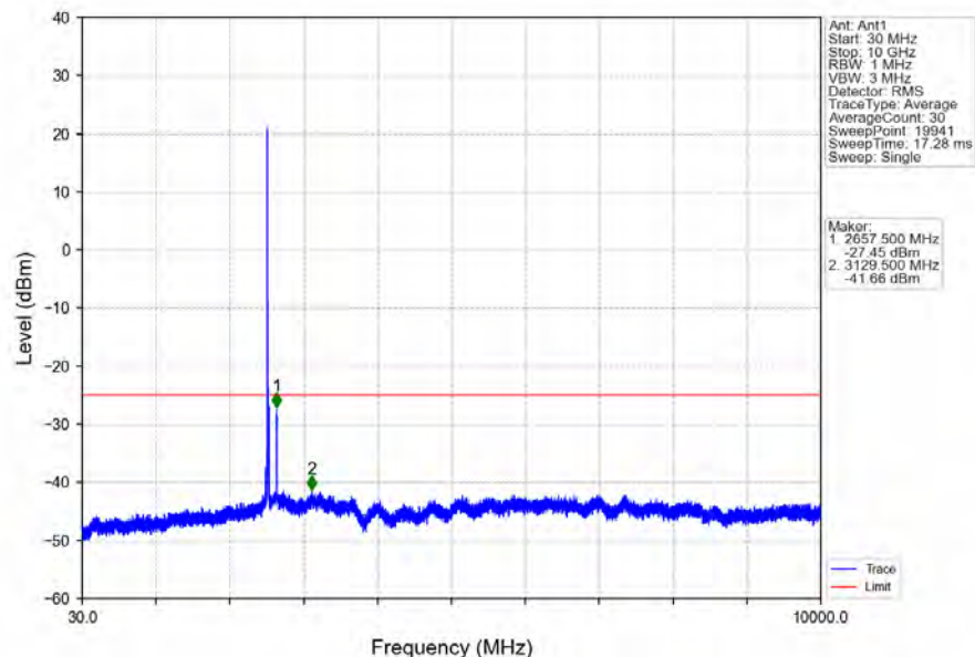
Band7_15MHz_64QAM_MCH_2535MHz_RB_1_0_NTNV
