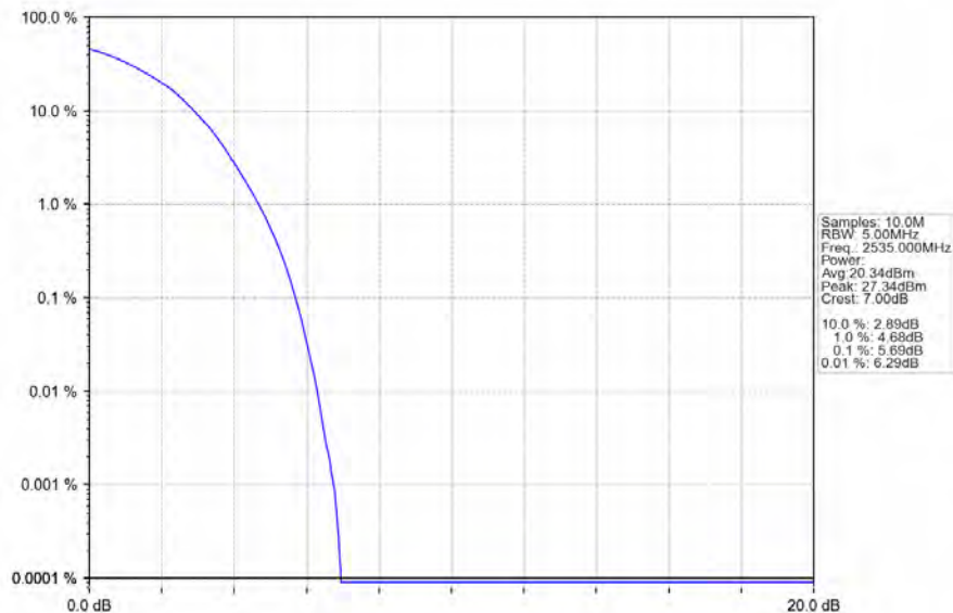
Band7_5MHz_64QAM_MCH_2535MHz_RB_25_0_NTNV
