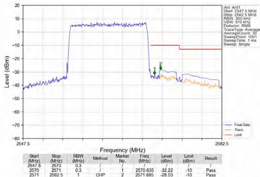
Band7_15MHz_16QAM_HCH_2562.5MHz_RB_75_0_NTNV
