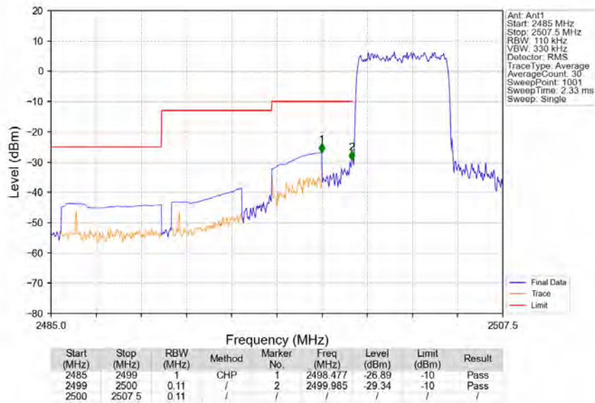
Band7_5MHz_64QAM_LCH_2502.5MHz_RB_25_0_NTNV
