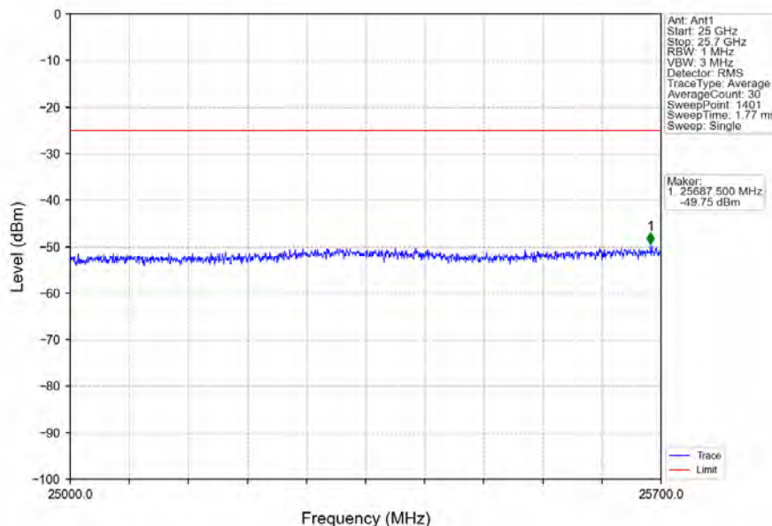
Band7_15MHz_64QAM_LCH_2507.5MHz_RB_1_0_NTNV
