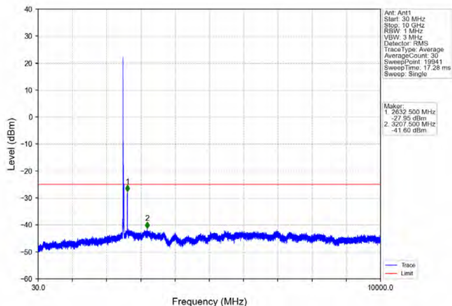
Band7_15MHz_64QAM_LCH_2507.5MHz_RB_1_0_NTNV
