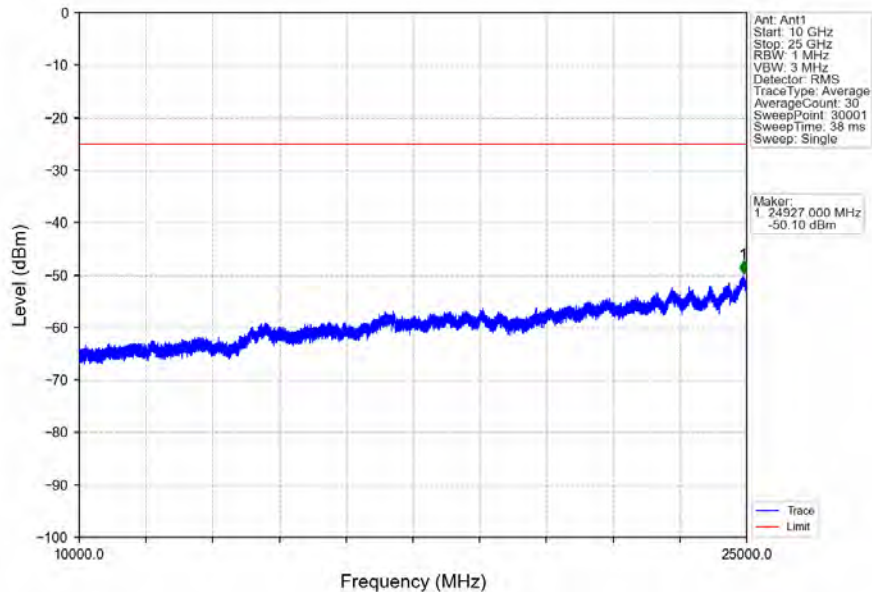
Band7_5MHz_64QAM_LCH_2502.5MHz_RB_1_0_NTNV
