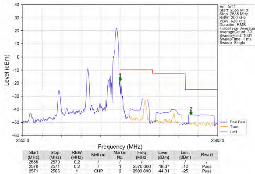
Band7_10MHz_16QAM_HCH_2565MHz_RB_1_49_NTNV
