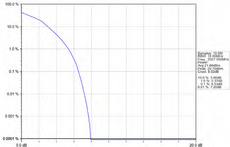
Band7_15MHz_16QAM_LCH_2507.5MHz_RB_75_0_NTNV
