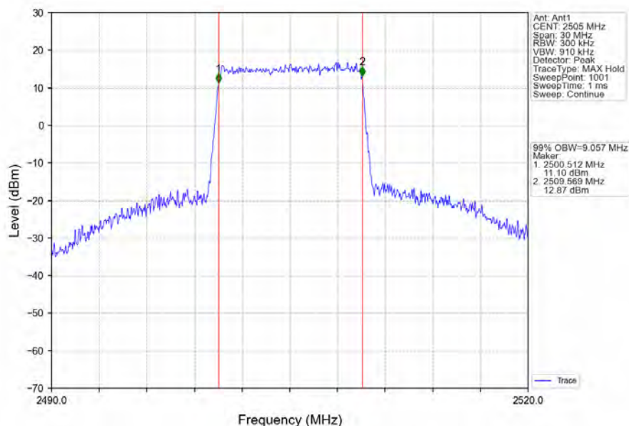
Band7_10MHz_64QAM_LCH_2505MHz_RB_50_0_NTNV
