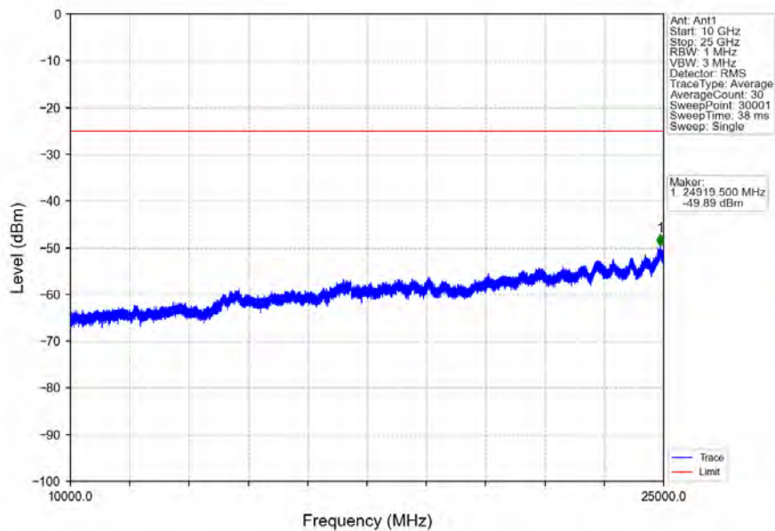
Band7_15MHz_16QAM_LCH_2507.5MHz_RB_1_0_NTNV
