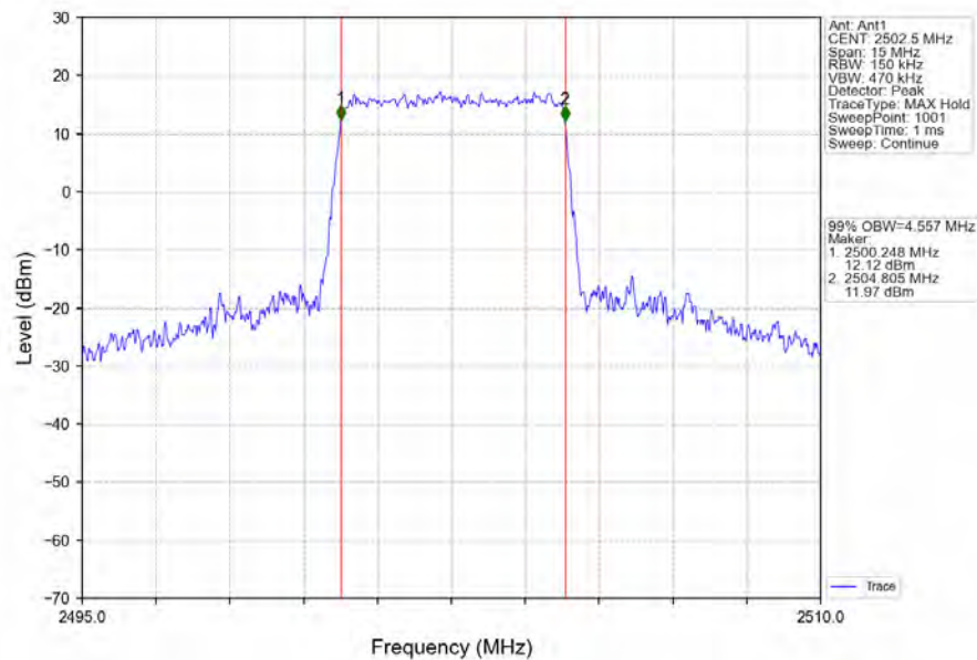
Band7_5MHz_16QAM_LCH_2502.5MHz_RB_25_0_NTNV
