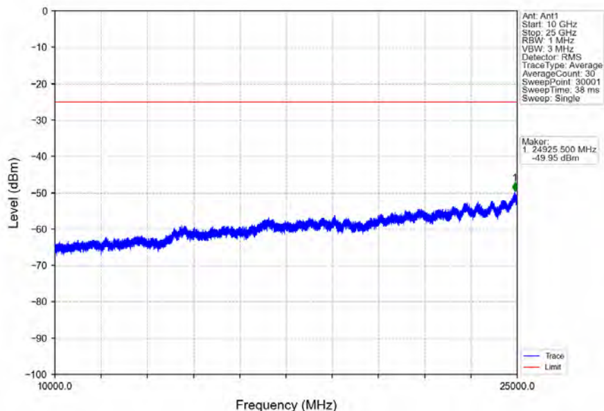
Band7_5MHz_16QAM_LCH_2502.5MHz_RB_1_0_NTNV
