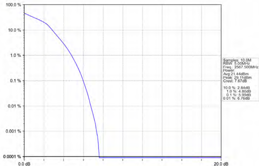
Band7_5MHz_16QAM_HCH_2567.5MHz_RB_25_0_NTNV
