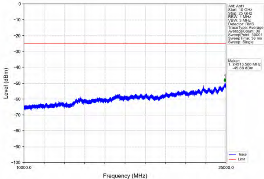
Band7_15MHz_16QAM_HCH_2562.5MHz_RB_1_0_NTNV
