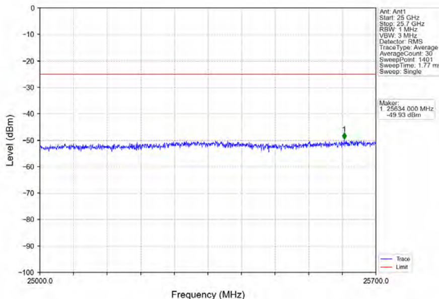
Band7_10MHz_64QAM_MCH_2535MHz_RB_1_0_NTNV
