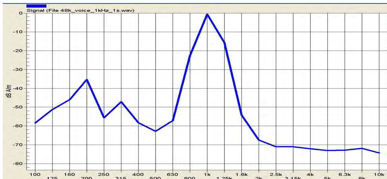
48KHz_Voice_1KHz_1S
