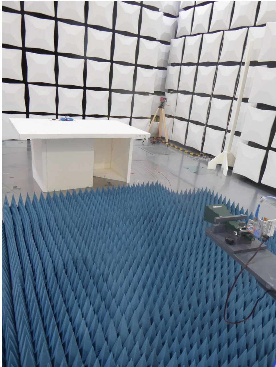
Test setup semi anechoic chamber M276, 12 GHz – 14 GHz
