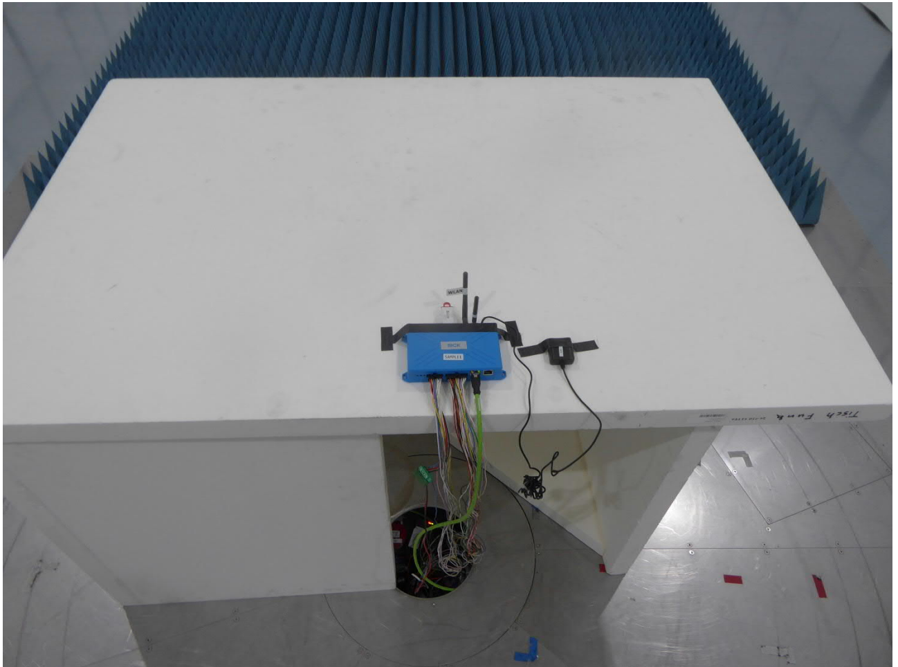
Test setup semi anechoic chamber M276 12 GHz – 14 GHz
