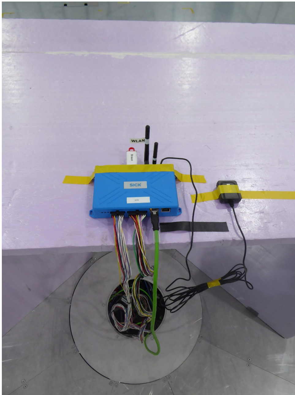
Test setup semi anechoic chamber M276 30 MHz – 12 GHz
