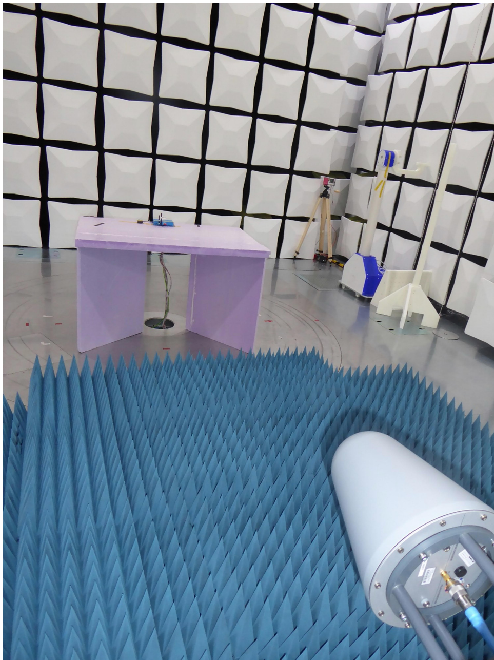
Test setup semi anechoic chamber M276, 1 GHz – 12 GHz
