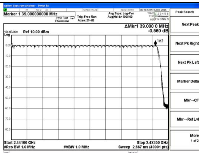
Test Plot 2 For Number of Hopping Channel(GFSK)
