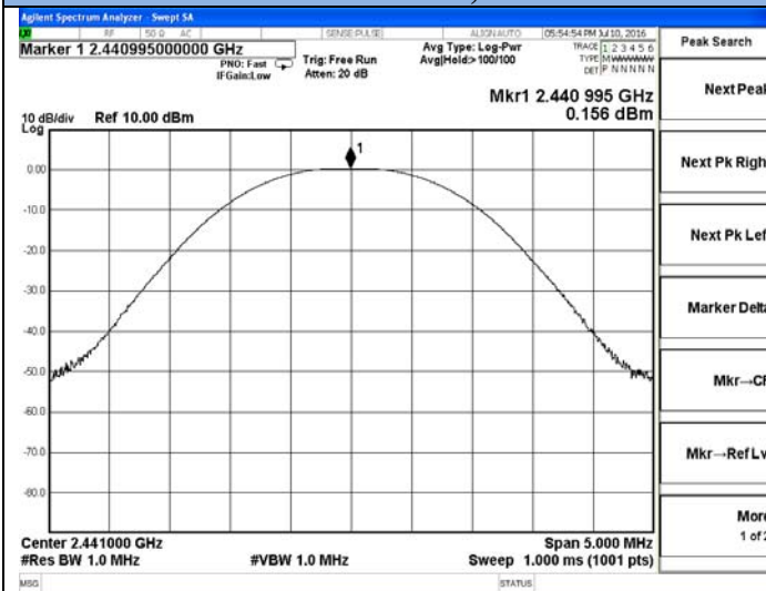
GFSK-Middle Channel, 2441MHz
