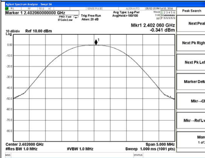
GFSK-Low Channel, 2402MHz
