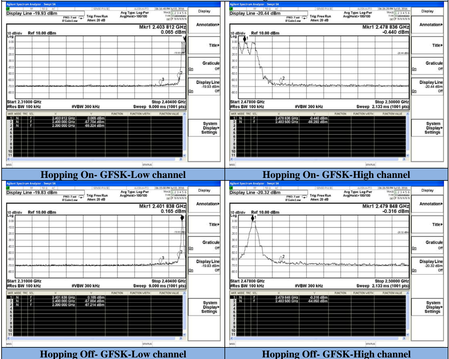
Test Plot of Band Edges
