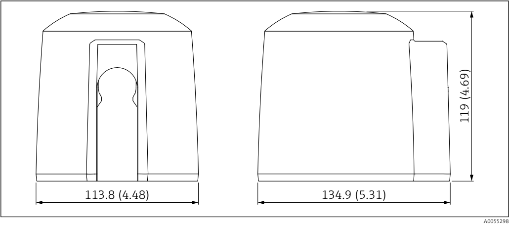
24 Dimensions for weather protective cover . Unit of measurement mm (in)
