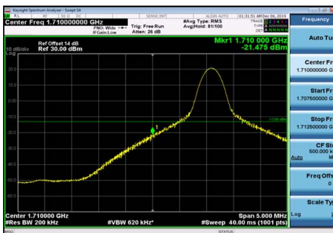
LowRange_FDD66_20MHz_1720_OneRB _low_QPSK
