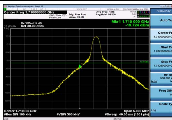
LowRange_FDD66_10MHz_1715_fullRB _Low_QPSK
