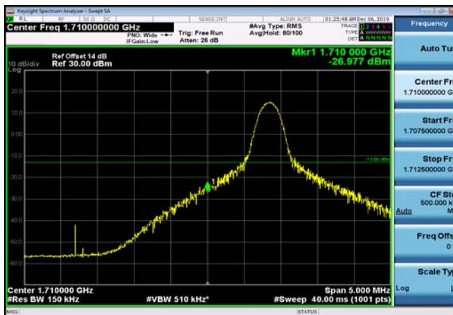
LowRange_FDD66_15MHz_1717.5_fullRB _Low_QPSK
