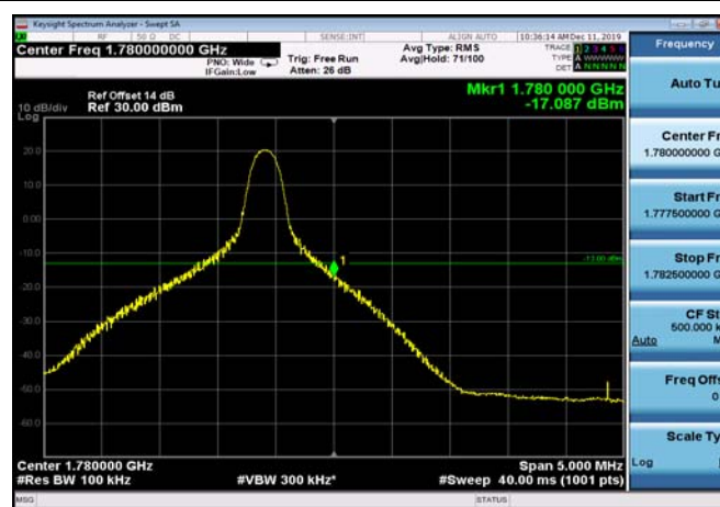
HighRange_FDD66_10MHz_1775_fullRB _High_QPSK
