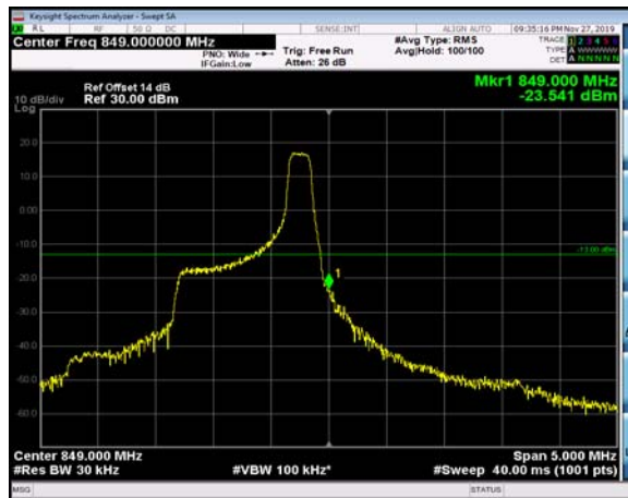
HighRange_FDD05_1.4MHz_848.3_fullRB _High_QPSK
