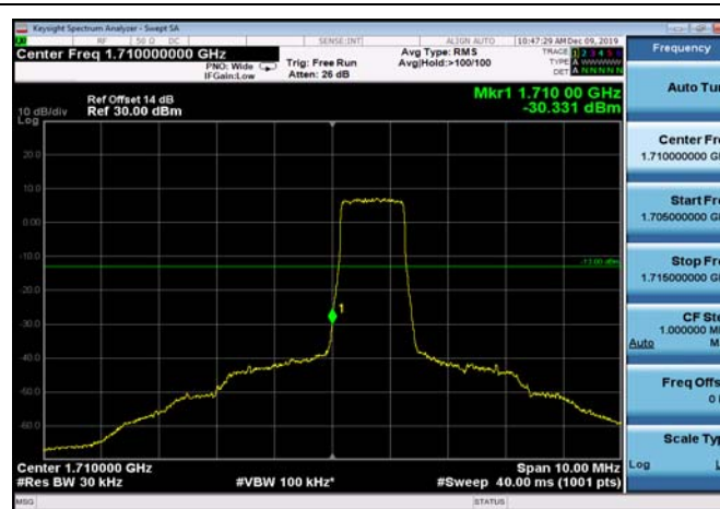
LowRange_FDD66_1.4MHz_1710.7_fullRB _Low_QPSK
