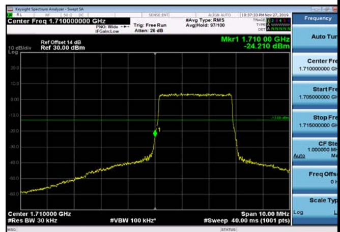
LowRange_FDD66_5MHz_1712.5_OneRB _low_Q16
