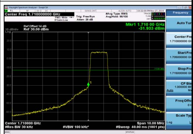
LowRange_FDD66_1.4MHz_1710.7_fullRB _Low_Q16
