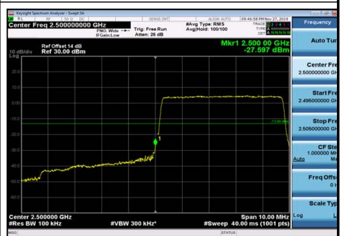
LowRange_FDD07_5MHz_2502.5_fullRB _Low_QPSK
