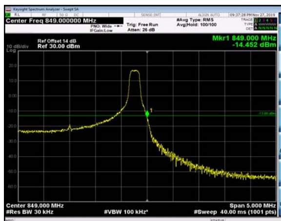
HighRange_FDD05_3MHz_847.5_OneRB _high_QPSK
