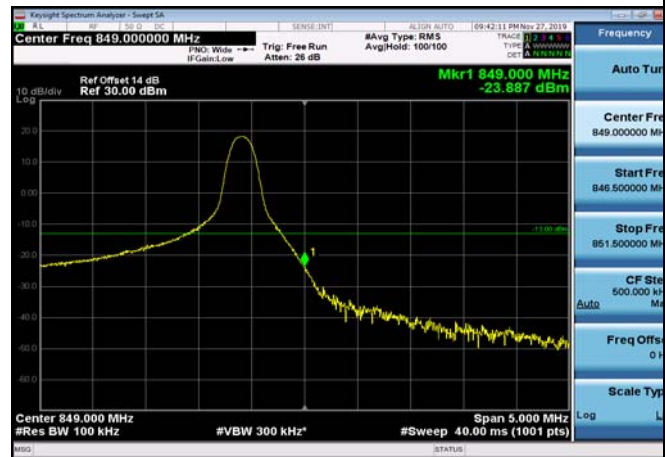
HighRange_FDD05_10MHz_844_fullRB _High_Q16
