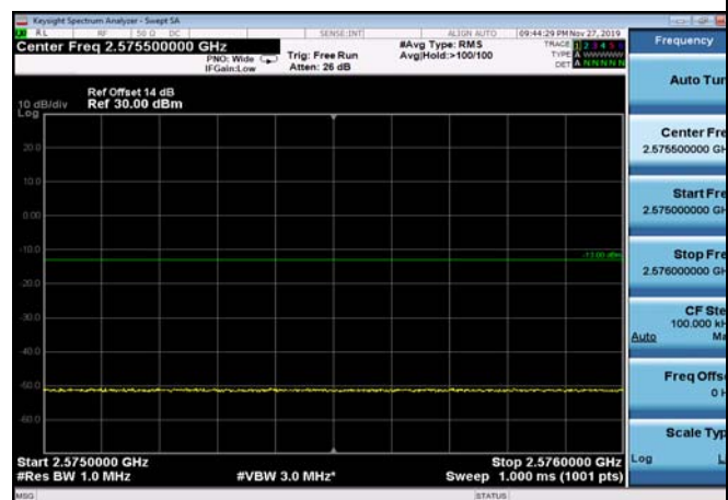
FDD07_5MHz_2502.5_QPSK_OneRB_high _ExtraBands_Range_2575~2576
