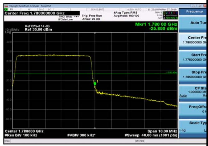
HighRange_FDD66_5MHz_1777.5_fullRB _High_Q16
