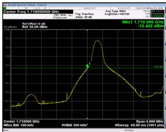
LowRange_FDD66_5MHz_1712.5_OneRB _low_QPSK
