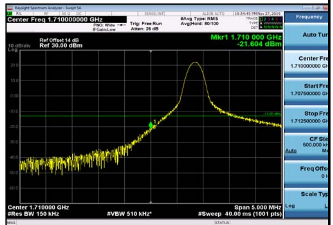
LowRange_FDD66_15MHz_1717.5_fullRB _Low_Q16
