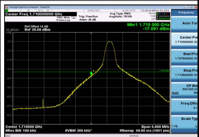
LowRange_FDD66_10MHz_1715_fullRB _Low_Q16
