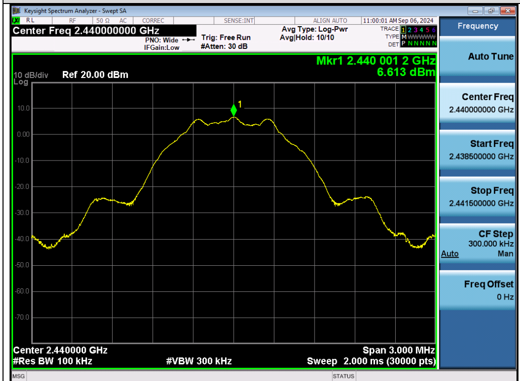
Test_Graph_LE1M_ANT1_2440_1Mbps_Reference Level
