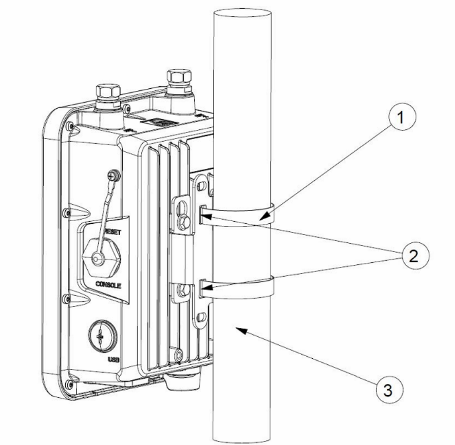
Figure 6 Cisco LoRaWAN Interface Module and Fixed Mount Kit Installed on a Pole
