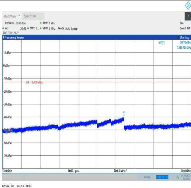
5-5-10MHz-10MHz-QPSK-QPSK-20501-20600-1RB#0-0RB#0 -3000~10000MHz-PASS
