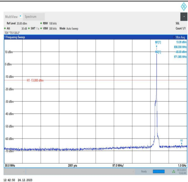
5-5-10MHz-10MHz-QPSK-QPSK-20501-20600-1RB#49-0RB# 0-30~1000MHz-PASS
