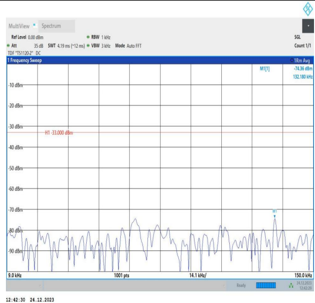
5-5-10MHz-10MHz-QPSK-QPSK-20501-20600-1RB#49-0RB# 0-0.009~0.15MHz-PASS
