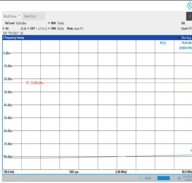
5-5-10MHz-10MHz-QPSK-QPSK-20476-20575-50RB#0-50RB #0-0.15~30MHz-PASS
