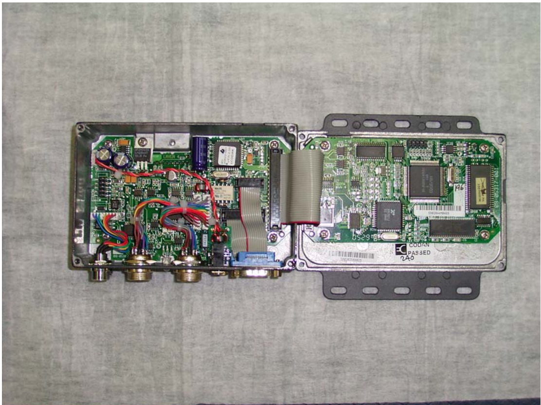
12. 2030 internal assembly (Audio assy 08-05986-001 on left, Microprocessor assy 08-05317-001 on right)
