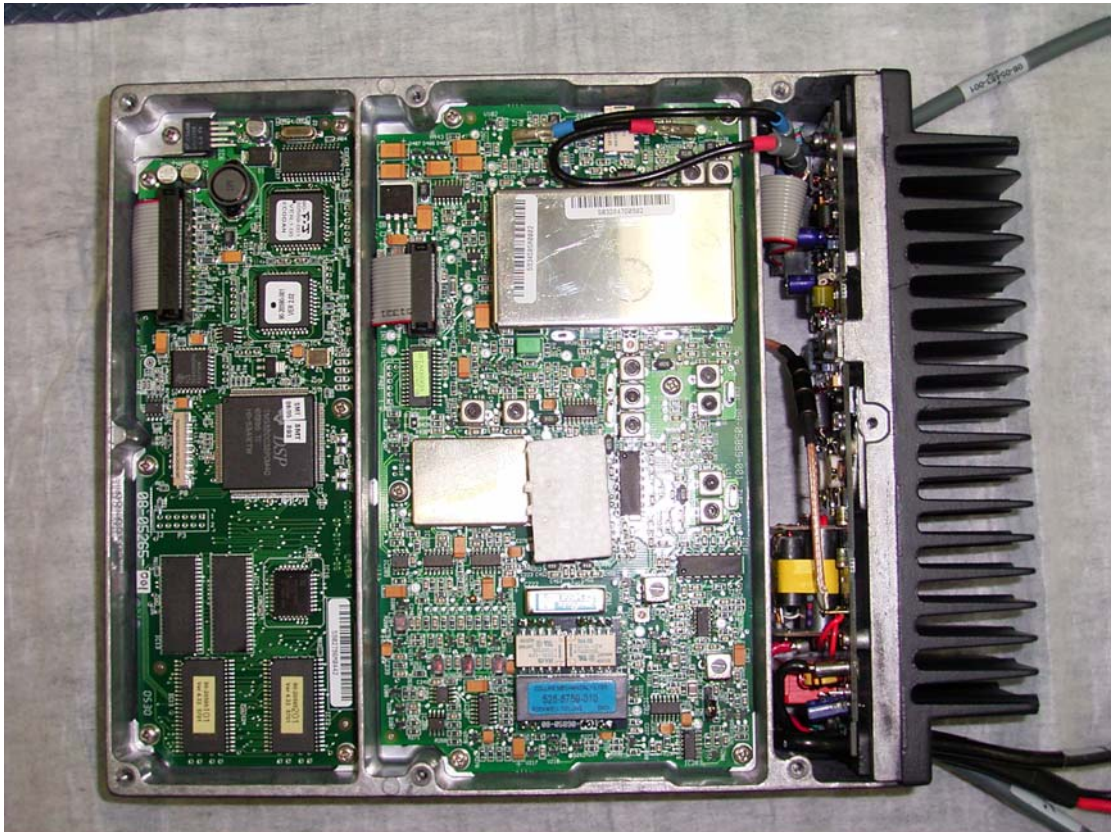
6. 2010 PA Filter and Control assembly (08-05910-001)
