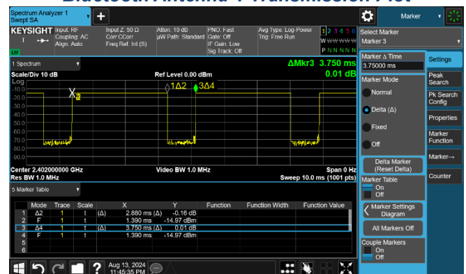
Bluetooth Antenna-1 Transmission Plot
