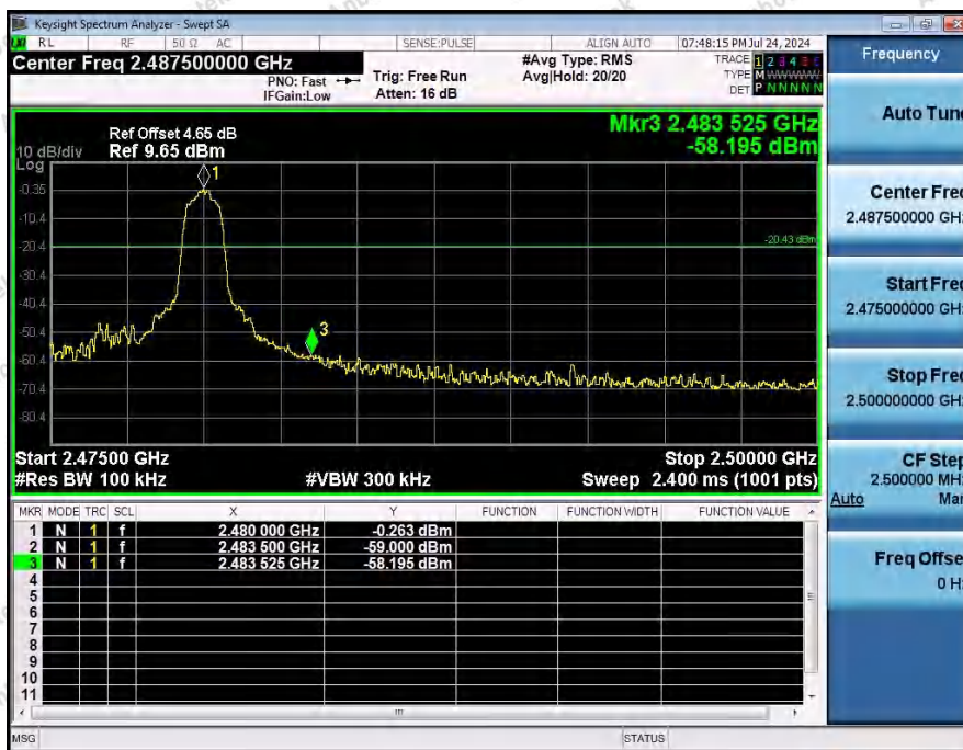
1_Reference_Level_Hopping_NVNT_ANT1_2-DH5_Hopping
