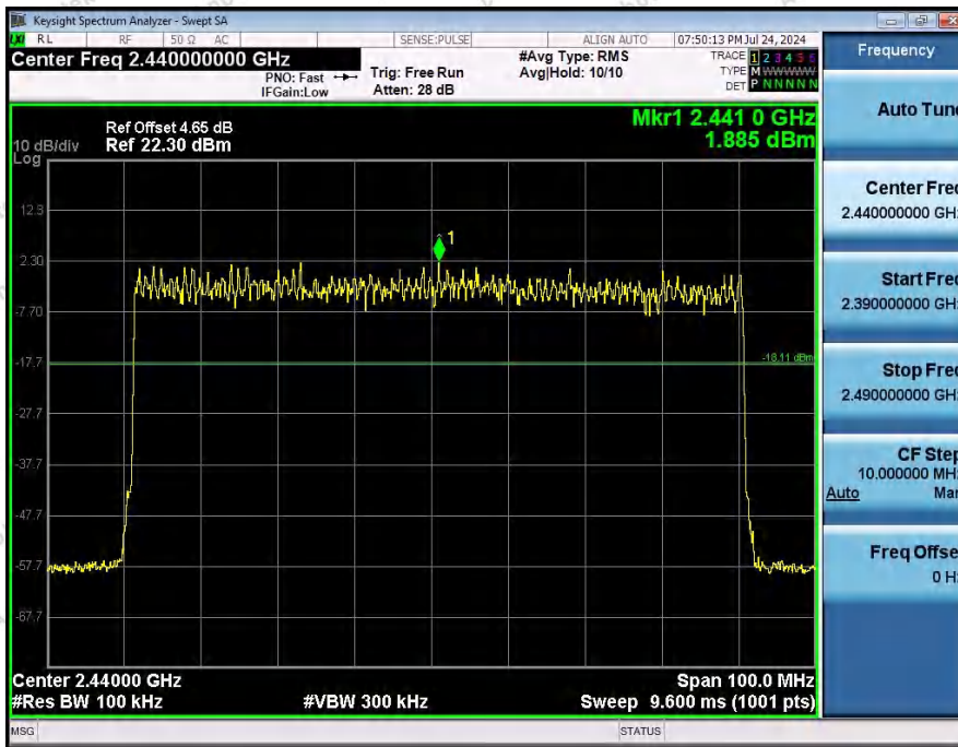
2_Band_Edge_(Hopping)_NVNT_ANT1_2-DH5_Hopping
