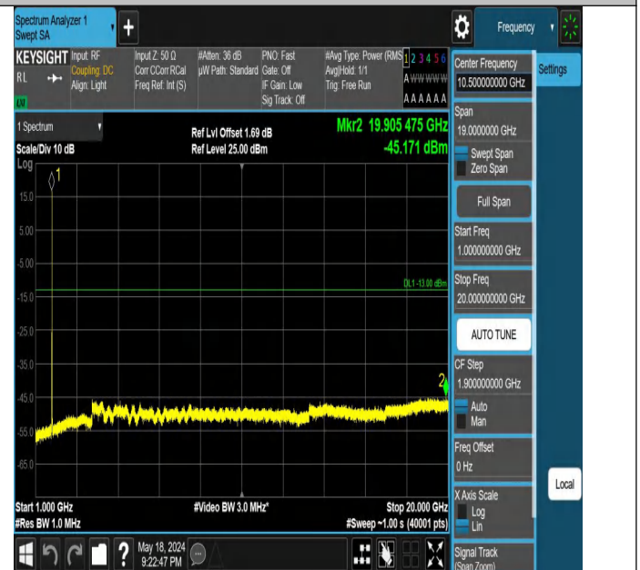
Band4-1513-1-1000~20000MHz-PASS
