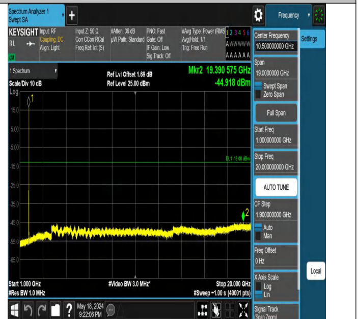
Band4-1413-1-1000~20000MHz-PASS
