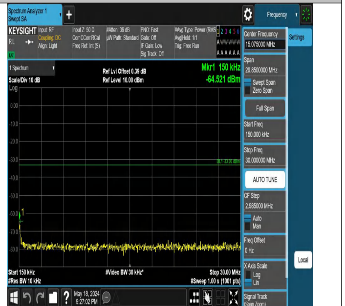
Band4-1413-3-0.15~30MHz-PASS
