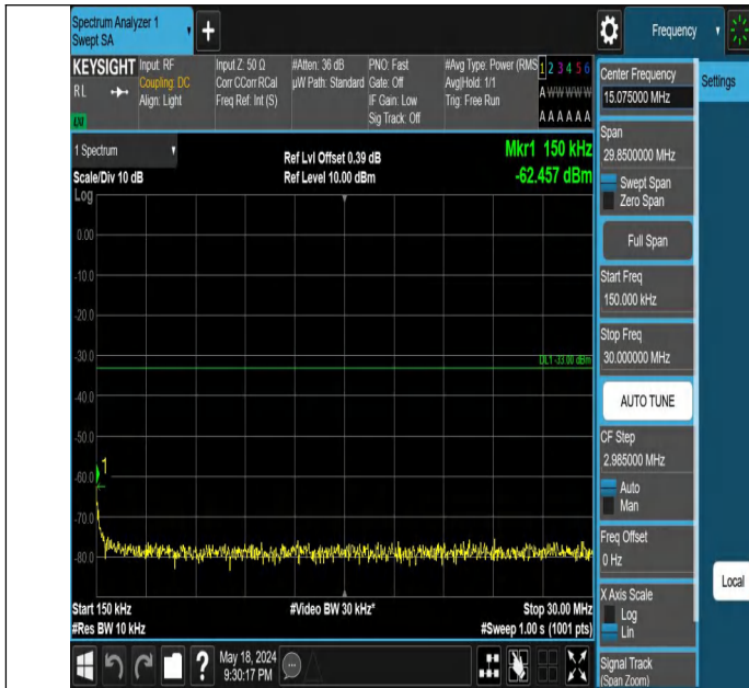
Band4-1513-4-0.15~30MHz-PASS
