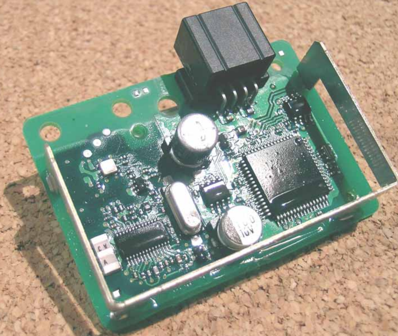
Model L0101456 PCB (top)
