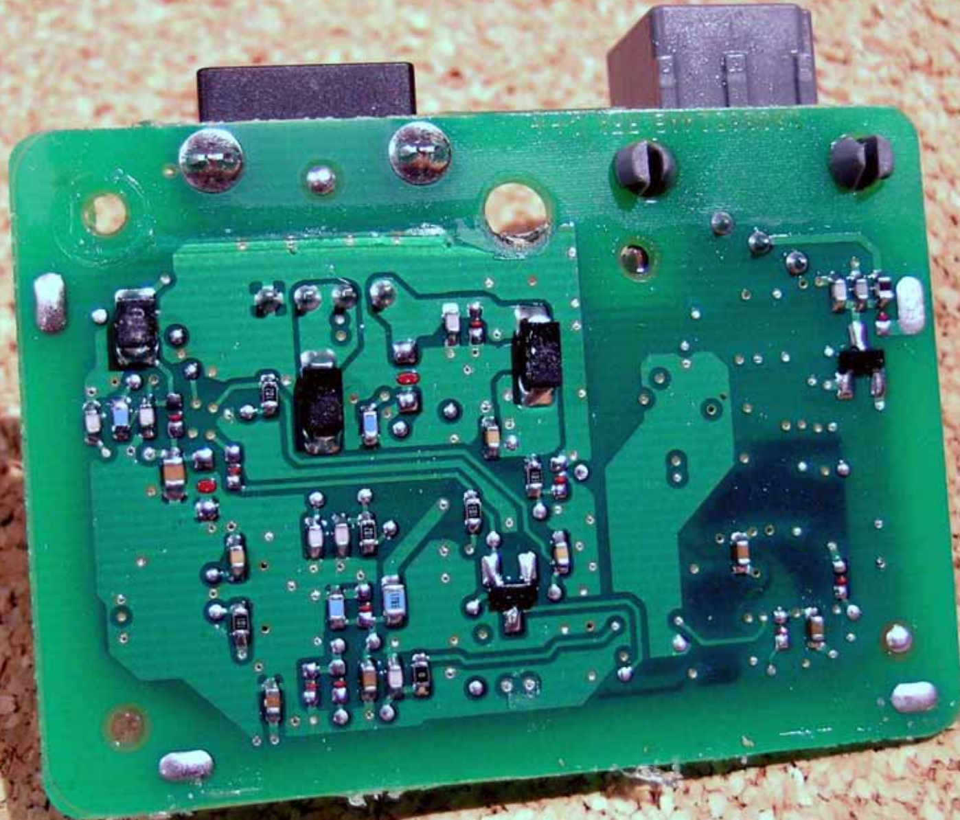
Model L0111925 PCB (bottom)
