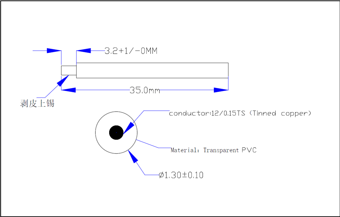
产品规格图(Antenna Specification chart)
