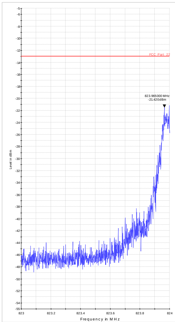
Diagram 37.05_BE_Ch128_EGPRS
