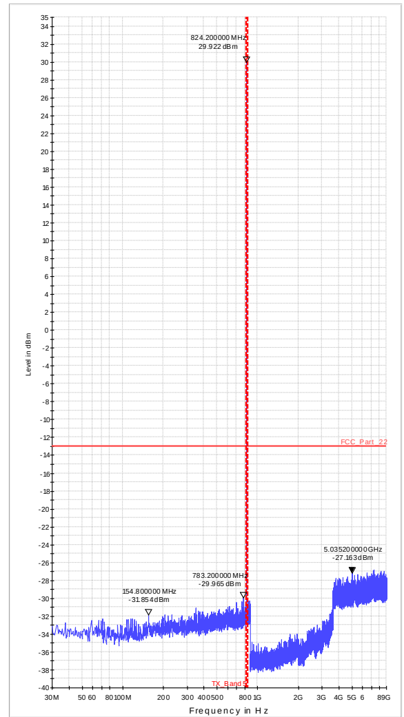
Diagram 36.14_RSE_Ch128_EGPRS_Sweep2
