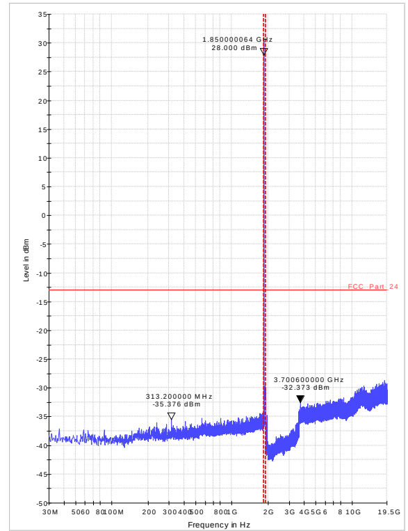
Diagram 36.21_RSE_Ch512_GPRS_Sweep2
