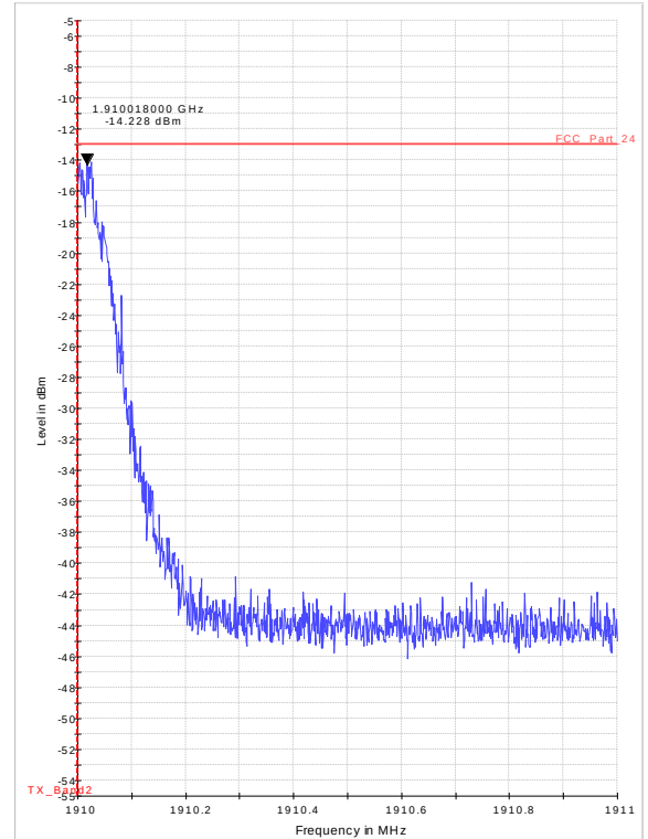
Diagram 37.11_BE_Ch810_GPRS_PK
