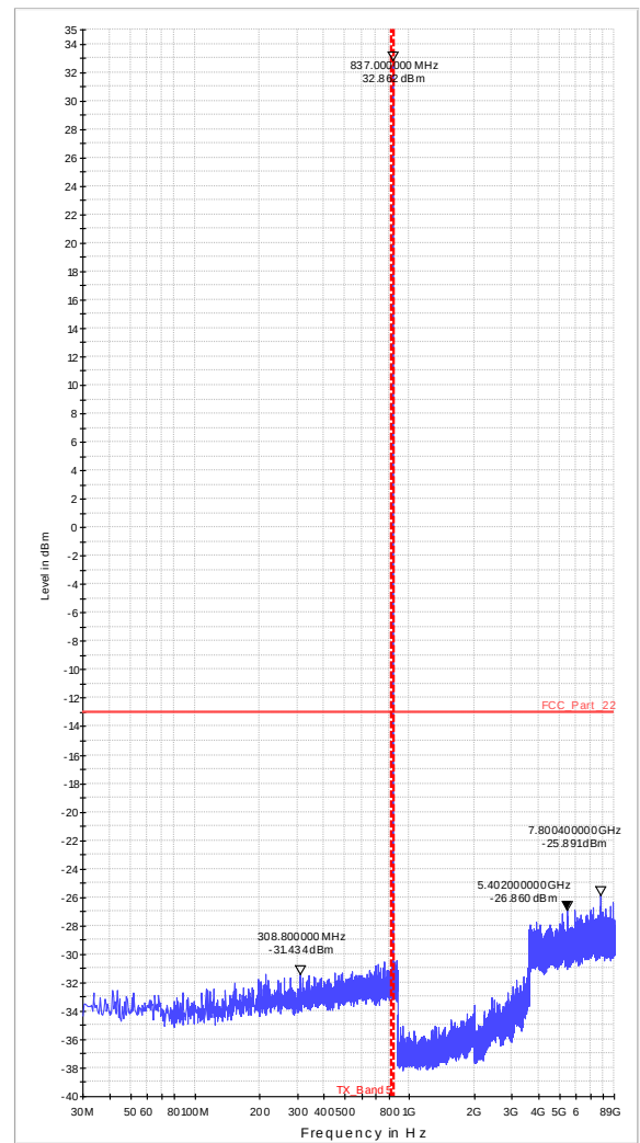
Diagram 36.10_Ch192_GRPS_Sweep2
