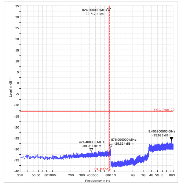
Diagram 36.08_Ch128_GRPS_Sweep2
