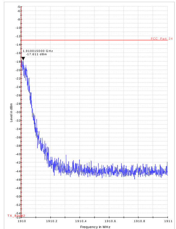
Diagram 37.13_BE_Ch810_EGPRS_PK
