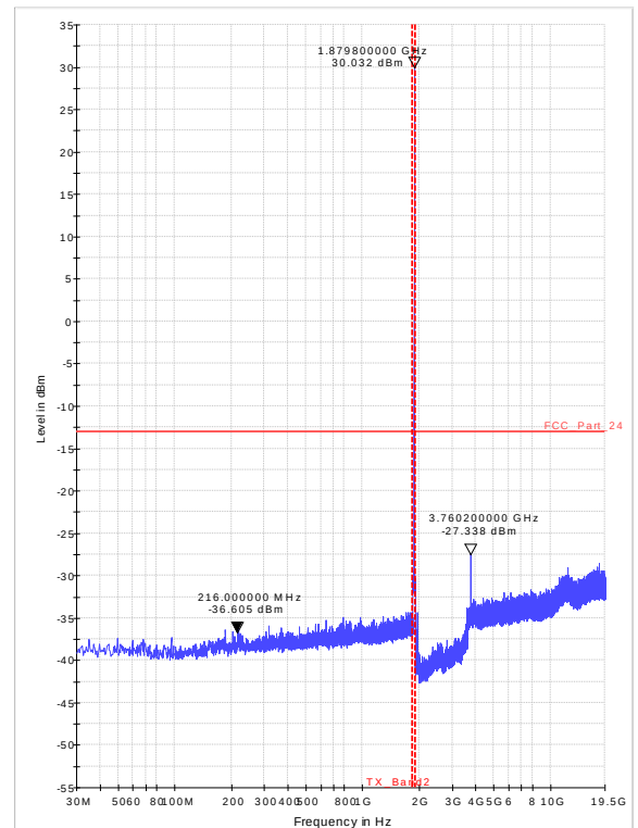
Diagram 36.23_RSE_Ch661_GPRS_Sweep2
