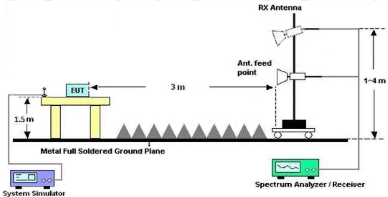
Figure 3. Above 1 GHz
