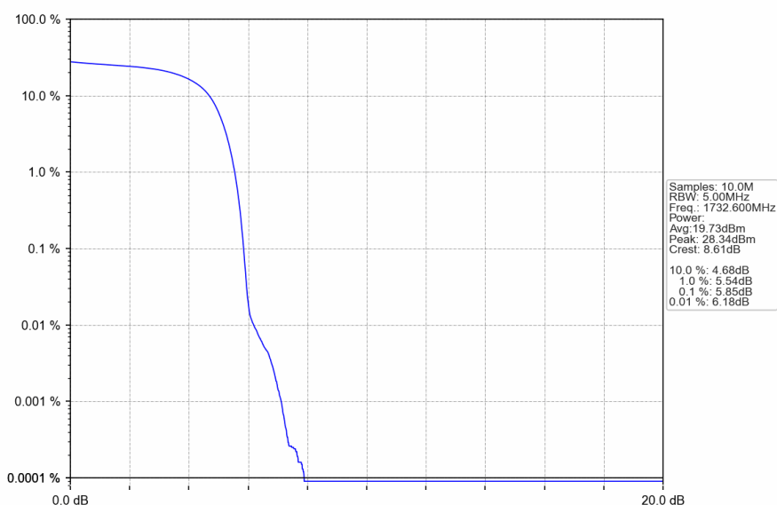
Band4_HSUPA_MCH_1732.6MHz_Subtest 1_NTNV
