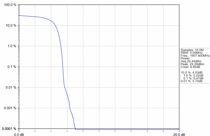
Band2_HSDPA_HCH_1907.6MHz_Subtest 1_NTNV
