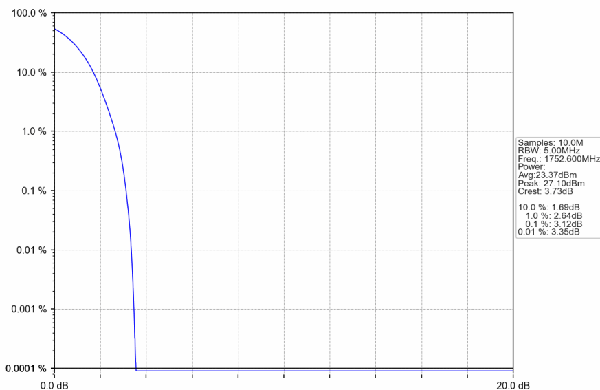
Band4_RMC_HCH_1752.6MHz_12.2kbps RMC_NTNV
