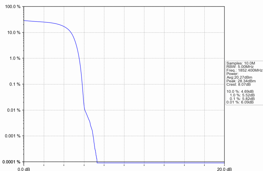
Band2_HSDPA_LCH_1852.4MHz_Subtest 1_NTNV
