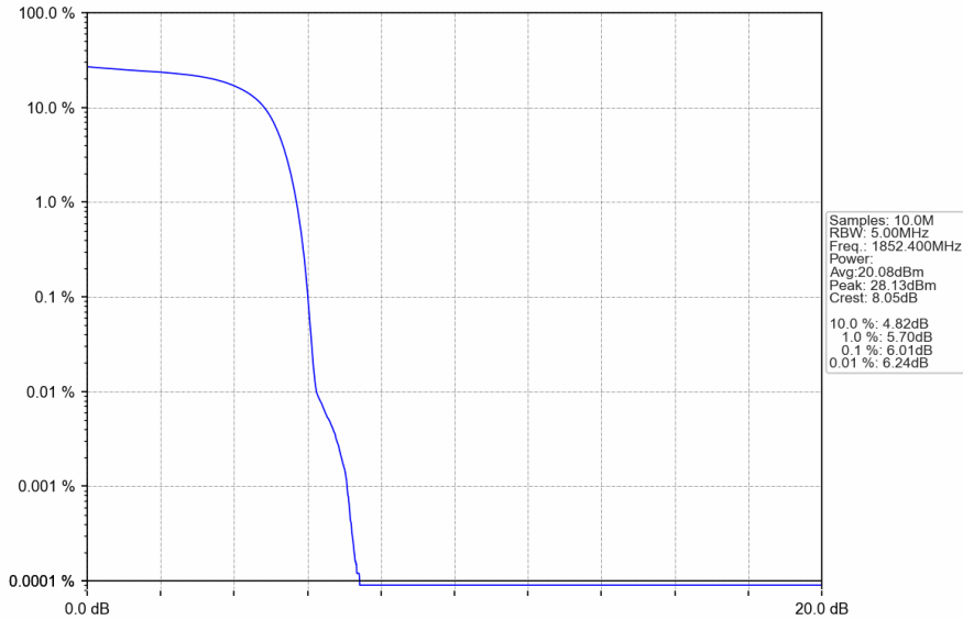
Band2_HSUPA_LCH_1852.4MHz_Subtest 1_NTNV
