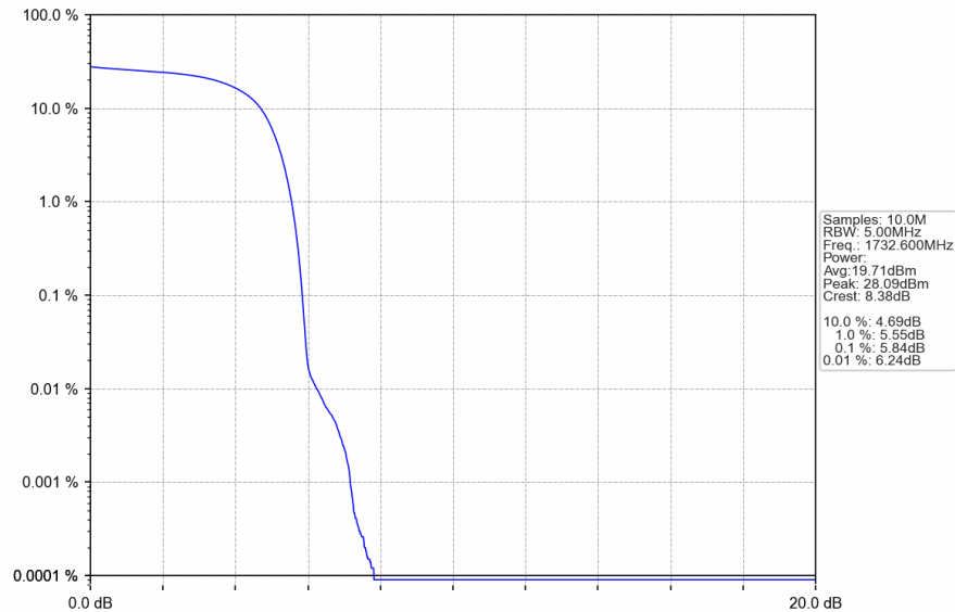
Band4_HSDPA_MCH_1732.6MHz_Subtest 1_NTNV
