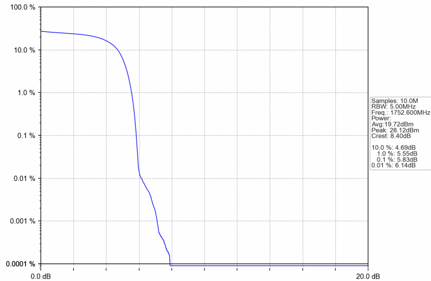
Band4_HSUPA_HCH_1752.6MHz_Subtest 1_NTNV
