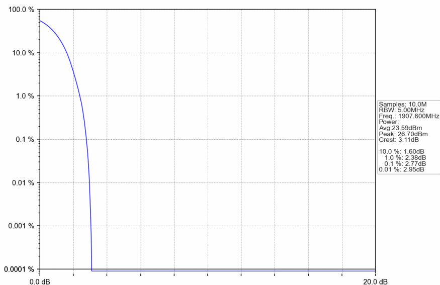
Band2_RMC_HCH_1907.6MHz_12.2kbps RMC_NTNV
