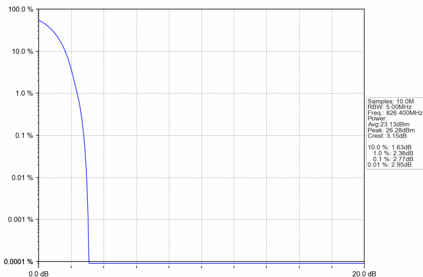
Band5_RMC_LCH_826.4MHz_12.2kbps RMC_NTNV
