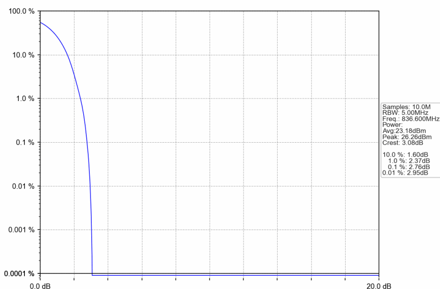
Band5_RMC_MCH_836.6MHz_12.2kbps RMC_NTNV
