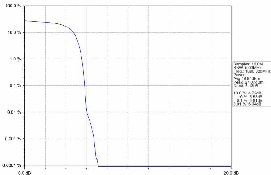
Band2_HSDPA_MCH_1880MHz_Subtest 1_NTNV
