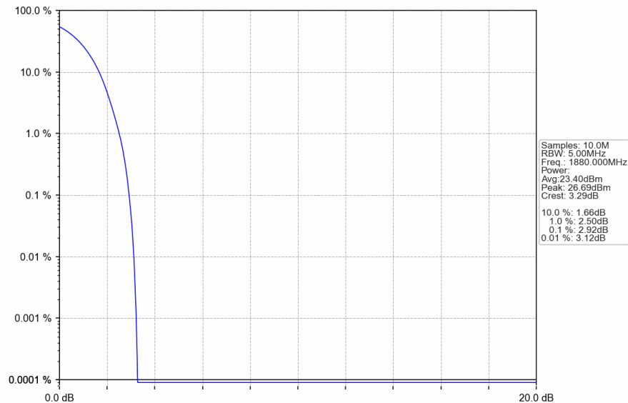
Band2_RMC_MCH_1880MHz_12.2kbps RMC_NTNV
