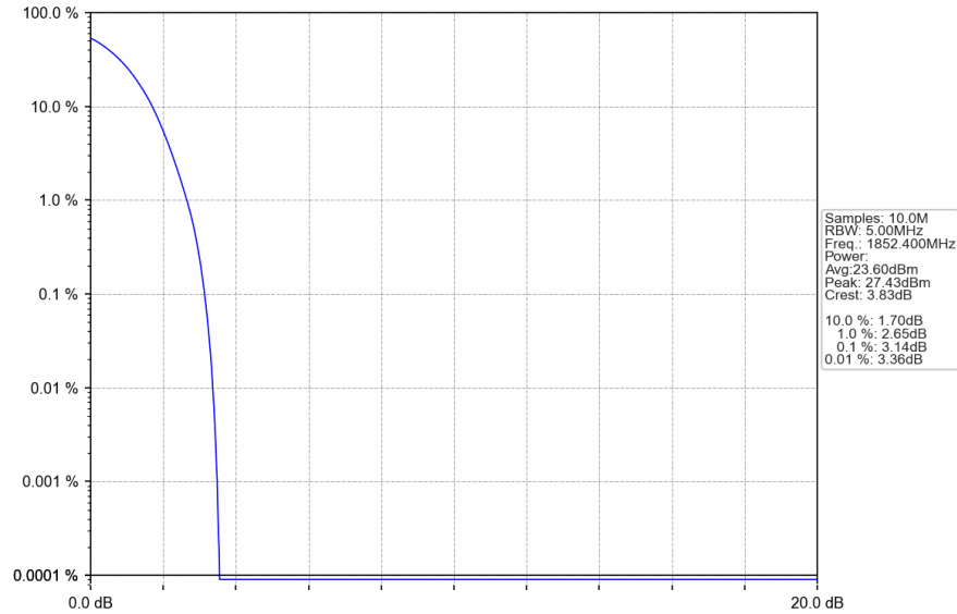
Band2_RMC_LCH_1852.4MHz_12.2kbps RMC_NTNV
