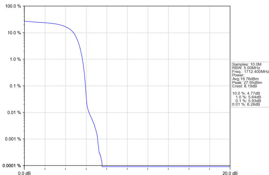
Band4_HSDPA_LCH_1712.4MHz_Subtest 1_NTNV
